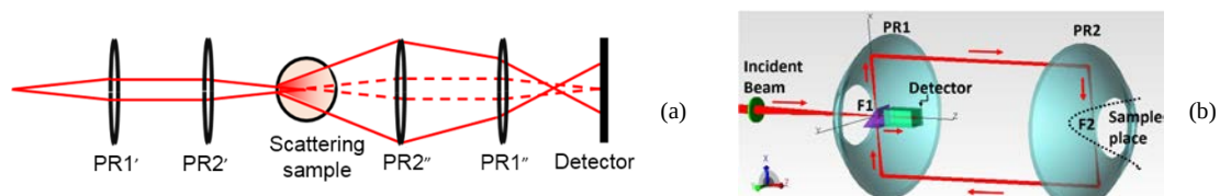
Fig. 1. (a) Effective equivalent optical train of the volume scanner and, (b) schematic TracePro design
