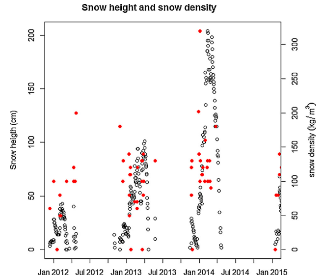
Fig. 5. Measured snow height and snow density during the years 2012, 2013 and 2014. The snow height (cm) is depicted by the black dots and the snow density (kg/m 3 ) by the red points. The values are not measured on site but at nearby a meteorological site.
