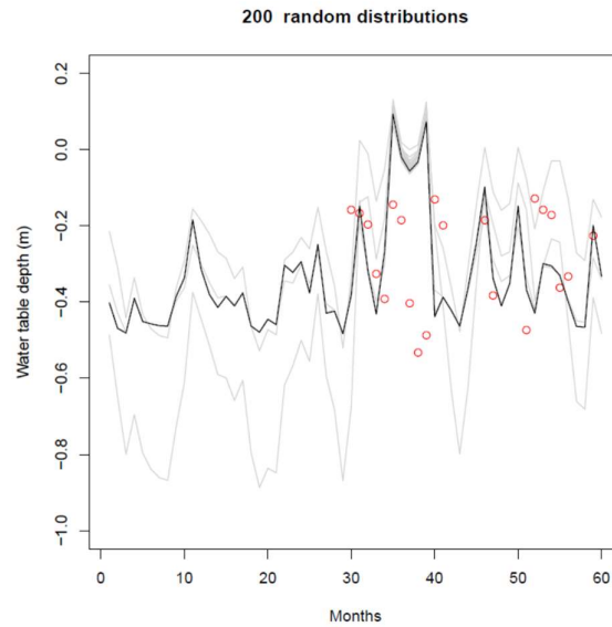
Figure 7-7 Water table depth at Monte Bondone. In grey, the result of 200 randomly taken parameter set from the posterior distribution, in red the measured values and in black, the water table depth calculated with the maximum a posteriori values.
