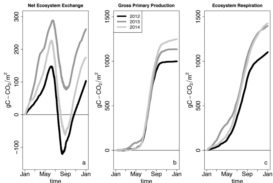
Fig. 6. (a) Cumulative NEE flux for each year (b) Cumulative GPP flux for each year (c) cumulative R_{eco} flux for each year.
