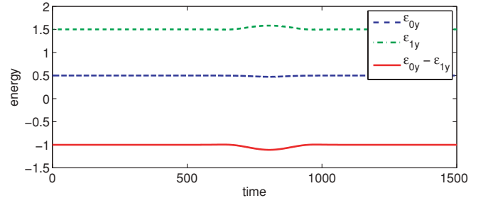
FIG. 4. (Color online) Evolution of \epsilon_{0y} (blue dashed), \epsilon_{1y} (green dot-dashed), and \epsilon_{0y} - \epsilon_{1y} (red solid) over the course of the CTAP process. Both energies are initially separated by \omega = 1 , but they do not maintain this separation due to the modification of the potential as the traps move closer together. Time is measured in units of 1/\omega and energy in units of \hbar\omega .
