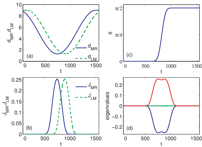
FIG. 2. (Color online) (a) Distance between the left-middle and the middle-right trap. (b) Tunneling strength between neighboring traps derived from the analytical model described in the text. (c) Mixing angle \theta and (d) time-dependent eigenvalues of the Hamiltonian (1). Time is measured in units of 1/\omega , energy in units of \hbar\omega , and distance in units of a_0 .
