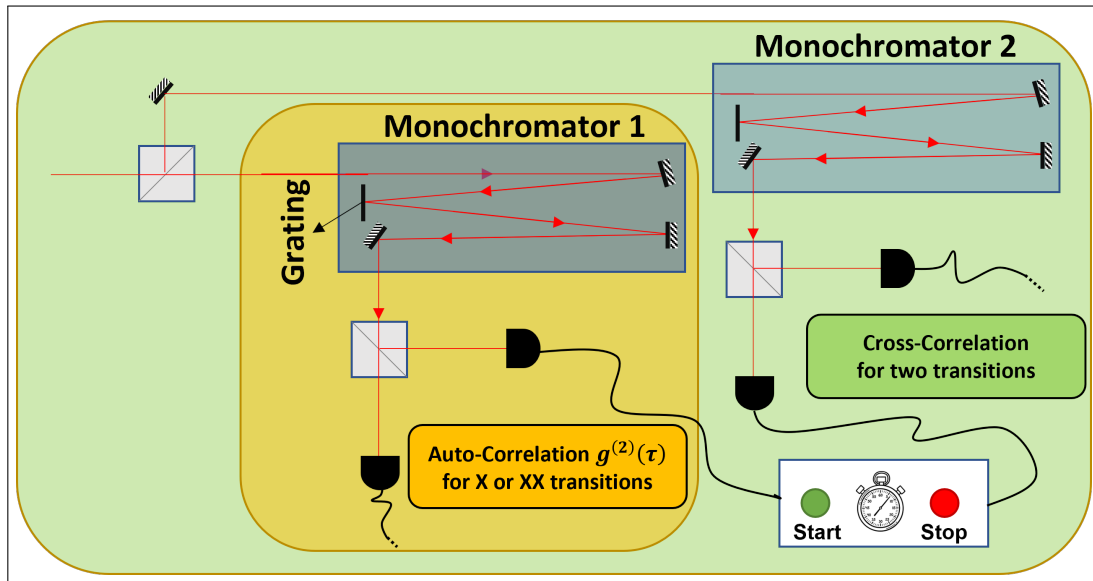
Figure 1.18: Time resolved spectroscopy. Auto-Correlation measurement to measure second order correlation function value g^{(2)}(\tau) for one transition (X or XX) and Cross-Correlation measurement to measure X lifetime or observing cascade.
