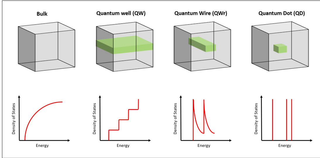
Figure 1.5: Energy of an electron in different confinements. From left to right: In bulk material, quantum well, quantum wire and quantum dot respectively.
