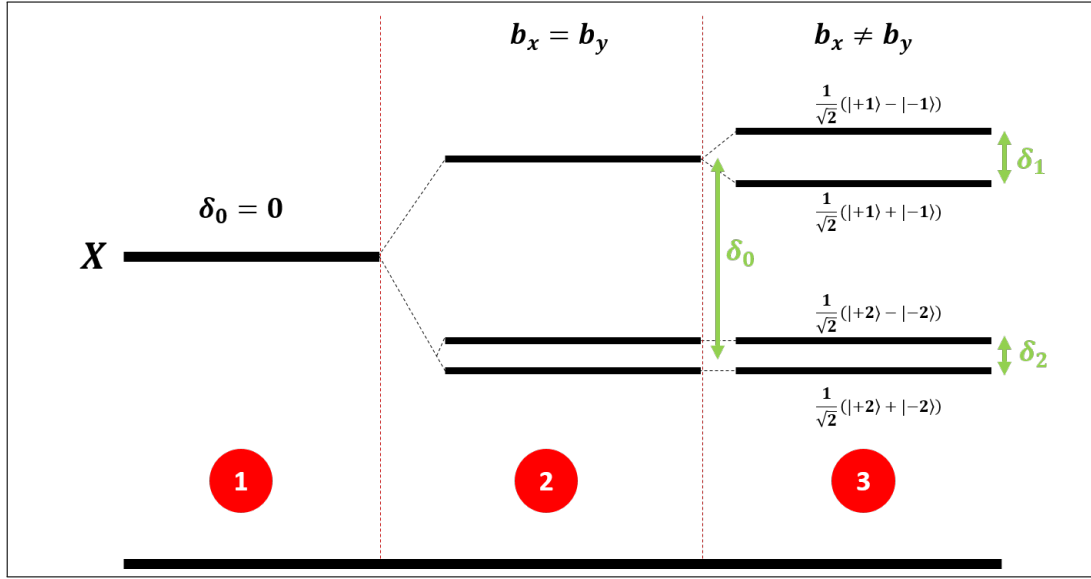
Figure 1.7: The schematics of “standard” exciton fine structure. The panel 1 shows neglecting the heavy and light hole splitting. Panel 2 showing the presence of splitting of heavy and light holes due to strain in self-assembled QDs. And panel 3 indicating the presence of fine structure splitting.
