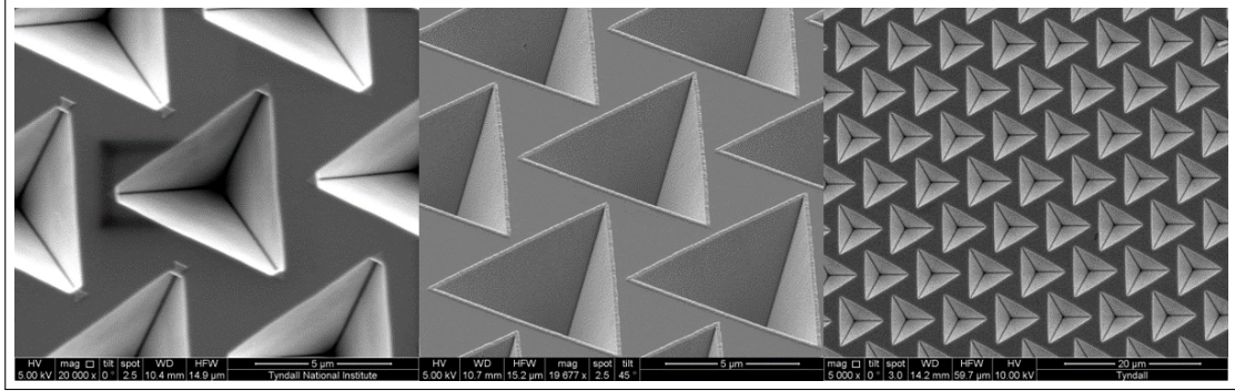
Figure 1.11: Inverted tetrahedral pyramidal recesses for epitaxial growth of QDs.
