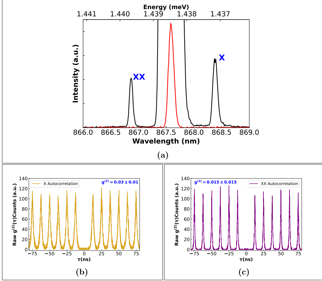
Figure 2.2: (a) The spectrum under TPE excitation with 10 ps pulses (red curve). (b) and (c) show the second order auto-correlation curves of the exciton (X) and biexciton (XX) transitions.
