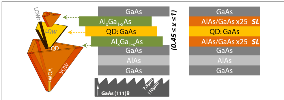
Figure 3.3: Schematics of the QD structure design. The sketch presents a complex ensemble of nanostructuring forming inside the pyramidal recesses. The epitaxial layer stacks show a generic QD layers' structure with two different designs for the confinement barriers: \text{Al}_x\text{Ga}_{1-x}\text{As} and Ga/Al digital alloy superlattice.
