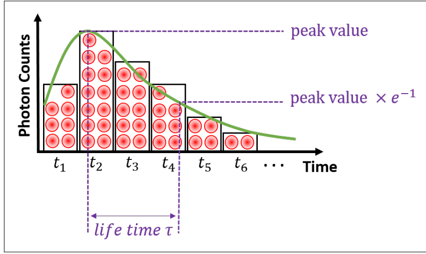
Figure 1.17: Time resolved spectroscopy. A method used to measure the emission life time of different excitonic transitions.
