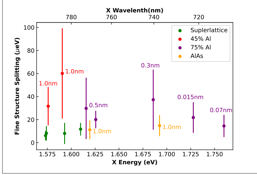
Figure 3.6: Average fine-structure splitting of GaAs QDs with different designs: nominal thickness and/or confinement barrier type. See Figure 3.3 and tables with the summary of the full epitaxial structure in Table 3.1-Table 3.3. Percentages in the legend refer to the AlGaAs nominal barrier Al content.
