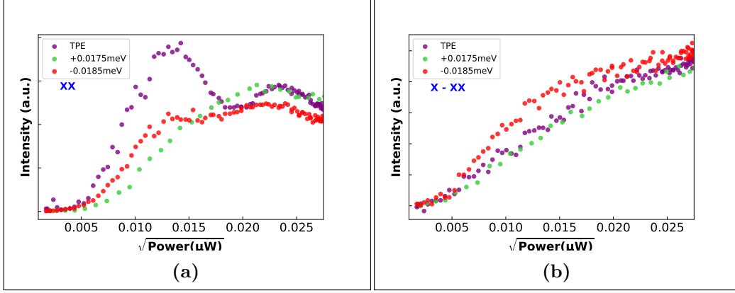
Figure 2.4: Power dependence of the biexciton and phonon-assisted exciton emission under different laser energy tuning conditions.
