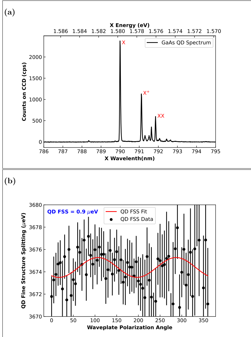
Figure 3.7: (a) The spectrum of the QD upon which the polarization entanglement was measured.(b) The measured FSS for the QD representative for entanglement measurements.
