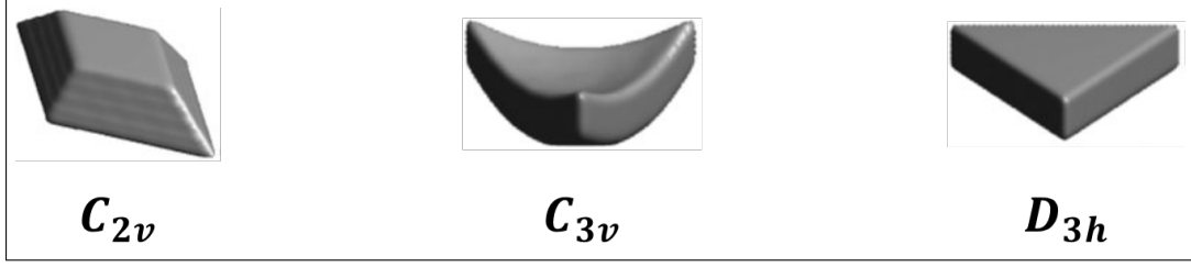
Figure 1.8: Different symmetries of QDs. C_{2v} ( C_{3v} ) symmetry has a two-fold (three-fold) rotation axis and two (three) vertical mirror planes containing the rotation axis. D_{3h} symmetry has a three-fold rotation axis, 3 two-fold rotation axes perpendicular to the first rotation axis and a horizontal mirror plane. The figure is taken from M. A. Dupertuis et al., Phys. Rev. Lett. 107, 127403 (2011).
