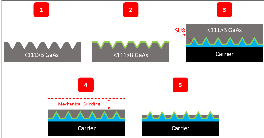
Figure 1.13: The Growth and post-growth process flow. (1) Tetrahedral pyramidal recesses are patterned on \langle 111 \rangle B GaAs wafer. (2) The QD heterostructure is grown in the MOVPE reactor. (3) As-grown sample is flipped and attached to a carrier with, for example, SU8(photoresist) for mechanical grinding. (4) Sample is ground until \sim 30\mu\text{m} of GaAs wafer is left. (5) Sample is then immersed into etching solution until pyramid's tips are exposed(chemical back-etching).
