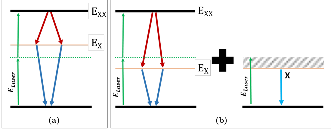
Figure 2.1: Two-photon excitation schema in QDs with different types of biexcitons (XX). (a) A binding biexciton two-photon excitation (TPE). (b) An antibinding biexciton TPE competing with the phonon-assisted exciton (X) population.
