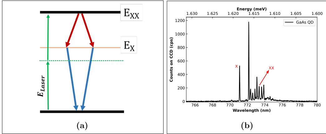
Figure 3.1: (a) A schematic diagram showing that binding biexciton, due to absence of phonon assisted exciton state excitation, is more efficient than antibinding biexciton (b) A typical GaAs QD spectrum. The XX transition is embedded among many other transitions once none-resonantly excited.
