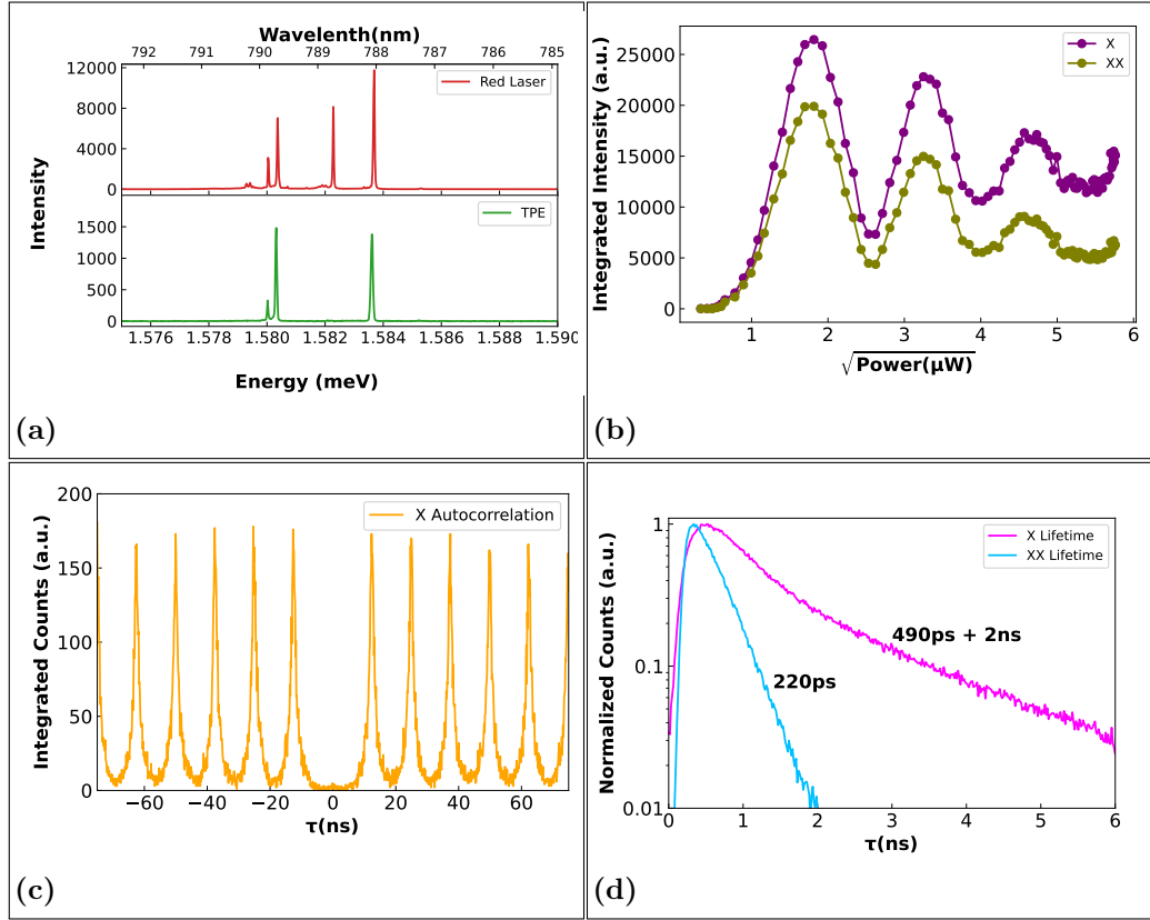
Figure 3.9: (a) Spectra of a GaAs/Al 0.45 Ga 0.55 As QD under non-resonant (top) and resonant (bottom) excitation. (b) Rabi oscillations. (c) An autocorrelation curve of the X transition demonstrating single photon emission with g^{(2)}(0) = 0.028 \pm 0.003 ( \pm 3\text{ns} range). (d) The lifetime decays of the exciton and biexciton.
