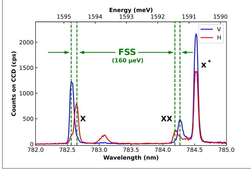
Figure 1.9: FSS phenomenology as a function of polarization. Different polarizations are well separated energetically from each other. X^* represents a charged transition which does not show any splitting due to its singlet spin state. The difference between counts of H and V polarizations is due to the CCD polarization-wavelength response difference.
