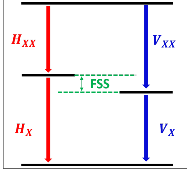
Figure 1.10: Schematics of excitonic complex of a QD energy levels with the presence of FSS
