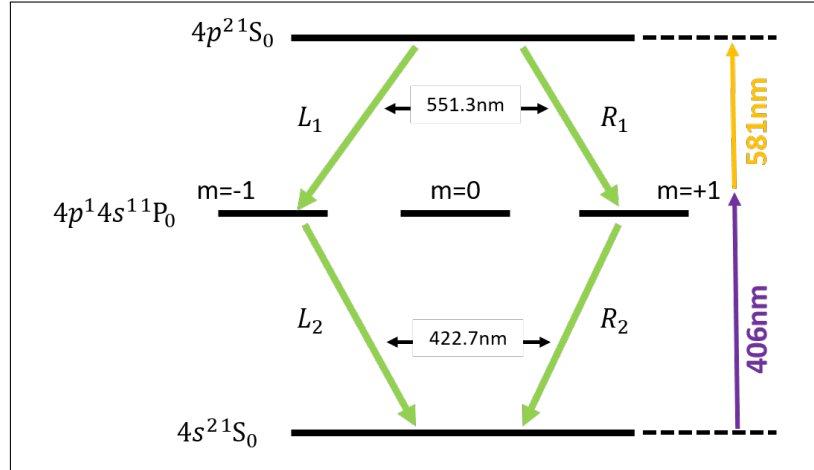
Figure 1.4: Polarization-entangled photon emission from a single atom via recombination cascade
