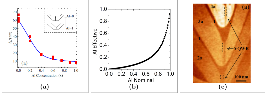
Figure 3.2: Growth model used to calculate the effect of Al content in self-limiting profile width during epitaxial growth over inverted tetrahedral pyramidal recesses. Images (a) and (c) are reproduced from V. Dimastrodonato et al, Phys. Rev. Lett. 2012, 108, 256102 with the permission of the American Physical Society Publishing
