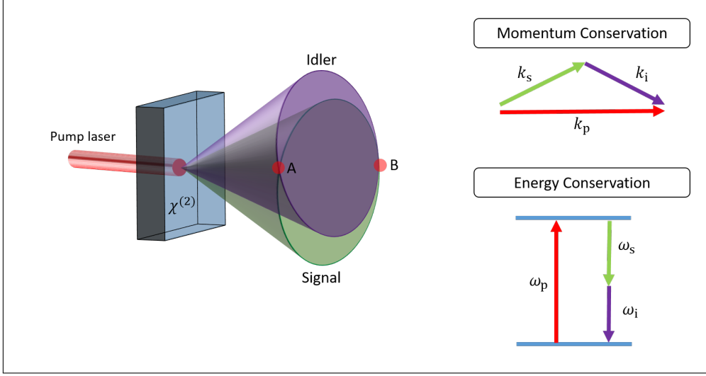
Figure 1.2: SPDC schematics with phase matching condition. This process is a probabilistic photon pair/single photon generation.
