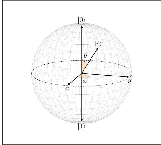
Figure 1.1: Bloch sphere, a graphical representation of a single state for two-level quantum system.
