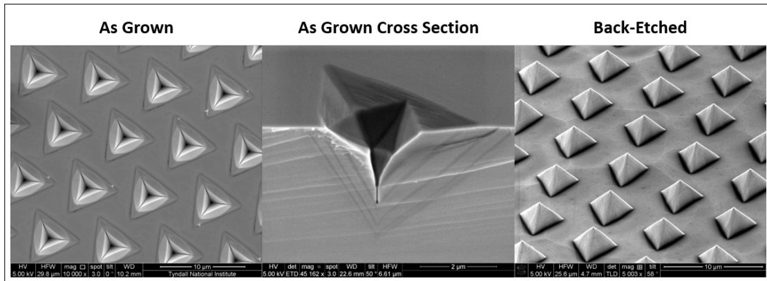
Figure 1.14: As grown (top view and cross-section) and back-etched pyramids.
