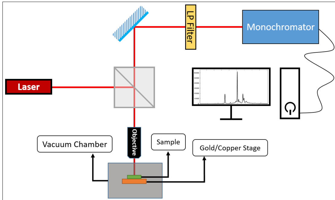
Figure 1.15: Schematic diagram of photoluminescence optical setup. Long pass (LP) filter, filters the laser and the QD emission is sent to the monochromator. The BS is 10:90 (10% Reflection, 90% Transmission).
