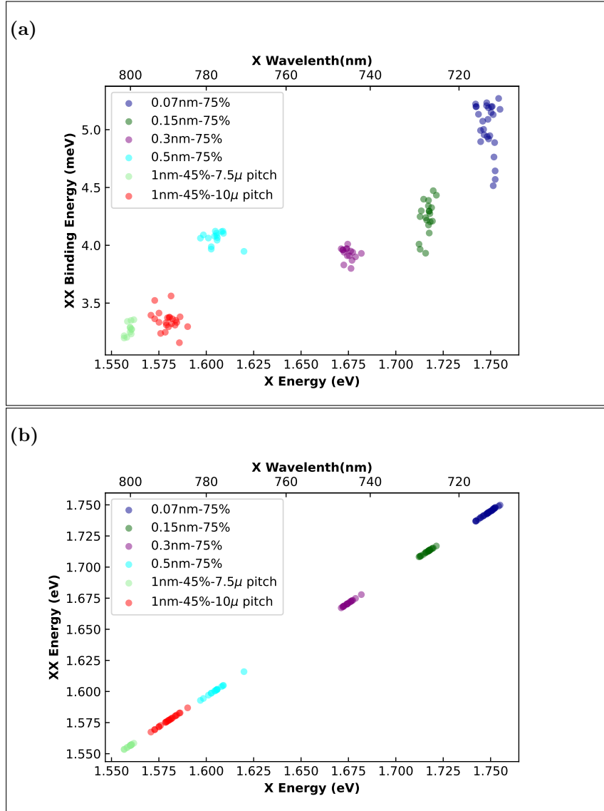
Figure 3.4: Distribution of Binding Energy for different samples. In plot legends the numbers are QD thickness and Al content in the \text{Al}_x\text{Ga}_{1-x}\text{As} barrier. (a) The scatter distribution of Binding energy for selected different QD thicknesses and Al contents. (b) the XX vs X transitions in selected cases showing a well linear relation
