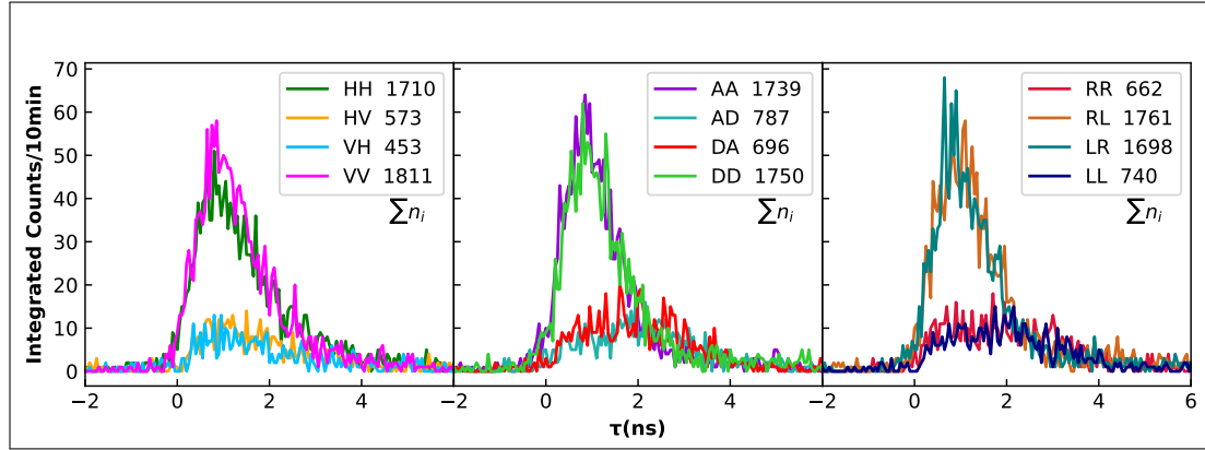
Figure 2.6: Polarization entanglement between the photons emitted during the biexciton-exciton recombination cascade. Full measurements in linear, diagonal, and circular polarization bases. The fine-structure splitting of the representative QD is 0.4 \pm 0.4 \mu\text{eV} .
