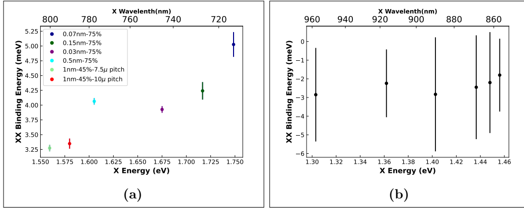
Figure 3.5: Distribution of Binding Energy for different samples. In plot legend the numbers are QD thickness and Al content in the \text{Al}_x\text{Ga}_{1-x}\text{As} barrier. (a) Distribution of averaged binding energy for different QD thicknesses and Al contents. (b) Distribution of binding \text{In}_x\text{Ga}_{1-x}\text{As} QDs counterpart. By comparing the standard deviations, GaAs are more uniform than \text{InGaAs} QDs.
