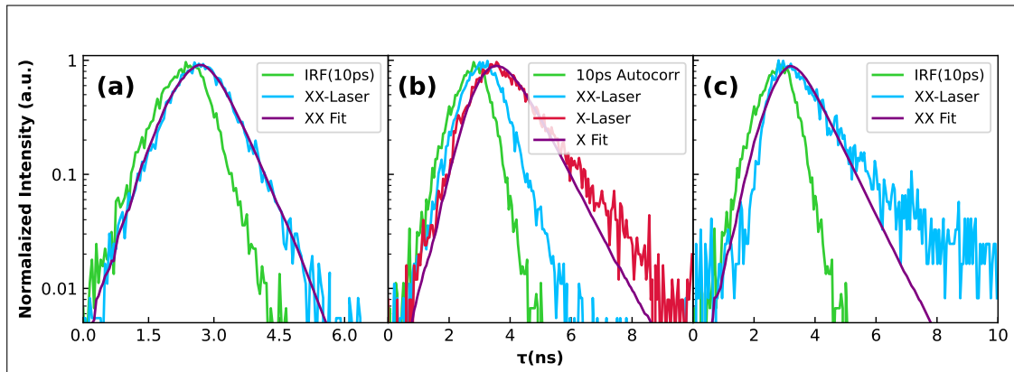
Figure 2.8: Lifetime extraction. (a) The biexciton-laser correlation; \tau_{xx} = 0.44\text{ns} \pm 0.03\text{ns} . (b) Correlations with the laser signal; \tau_x = 0.77\text{ns} \pm 0.04\text{ns} . (c) Exciton lifetime from the biexciton-exciton recombination cascade, i.e. the g^{(2)}(0) peak; \tau_x = 0.78\text{ns} \pm 0.04\text{ns} .
