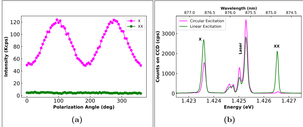
Figure 2.10: (a) QD photoluminescence under circularly polarized TPE showing strong suppression of the biexciton recombination cascade. Here a different QD was used than the one discussed in the main text. (b) Comparison of non-polarized spectra obtained under circularly and linearly polarized laser light tuned to the TPE resonance ( \pi pulse area for the biexciton transition).
