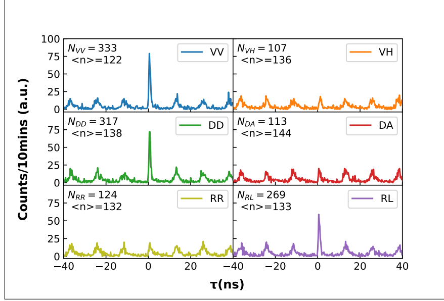
Figure 3.8: Six curves in linear, diagonal and circular bases were taken. As we can see, correlations between linearly co-polarized and anti-correlations between circularly polarized photons are observed.
