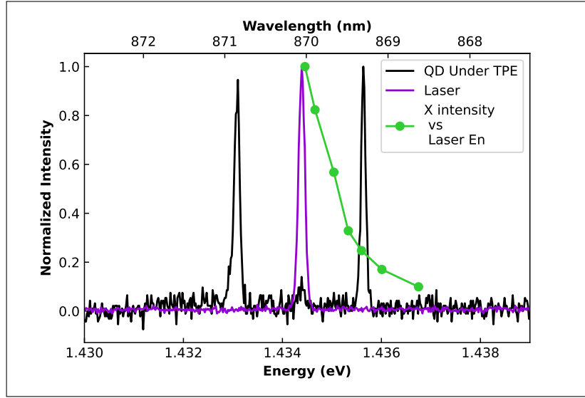
Figure 2.5: The exciton intensity dependence as a function of a laser pulse energy detuning. The spectrum is linearly polarized in a way to transmit photons originating from the biexciton recombination cascade only.
