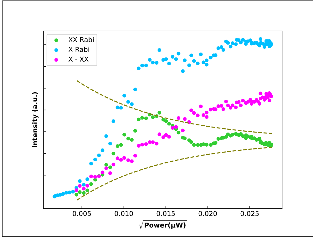
Figure 2.3: Excitation power dependence. The dashed lines are the envelopes of the damped Rabi oscillations. The X-XX curve is the difference between the exciton and biexciton intensity at the same excitation power. These are photoluminescence events occurring due to the phonon-assisted exciton population, which do not originate in the biexciton-exciton recombination cascade. The curves are represented not explicitly normalised to the dot population to allow an easier comparison of the different events. In an ideal case, the biexciton population maximum intensity would correspond to its 100 per cent occupancy
