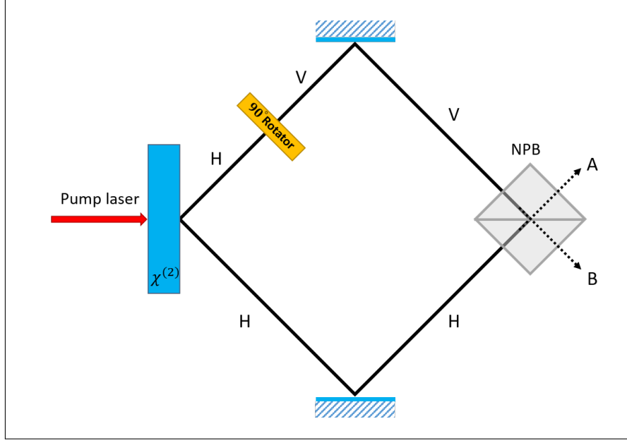
Figure 1.3: Post-selective entanglement generation with type-I photon pair generation
