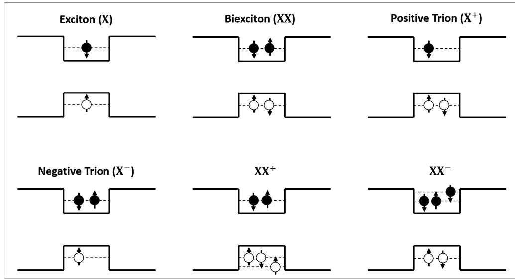
Figure 1.6: Name and structure of different excitonic complexes forming inside the QD.
