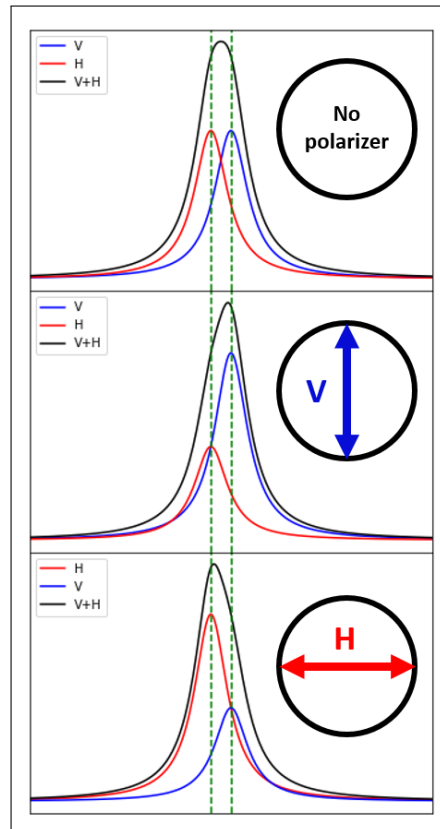
Figure 1.16: Polarization resolved spectroscopy. The upper most inset indicates the overlapped V and H polarizations when there is no polarization optics on the way. By introducing a linear polarizer, once it is vertically aligned, the H polarization is suppressed and the overall peak moves toward the vertical polarization as indicated in the middle inset. The opposite will happen when the polarizer is horizontal (the bottom inset).
