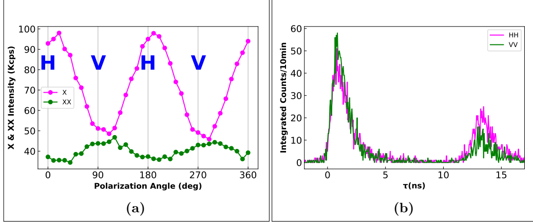
Figure 2.7: Polarization-resolved g^{(2)}(\tau) (a) Linear polarization analysis of exciton and biexciton transitions. (b) Comparison of correlation curves between horizontally and vertically co-polarized biexciton and exciton photons.
