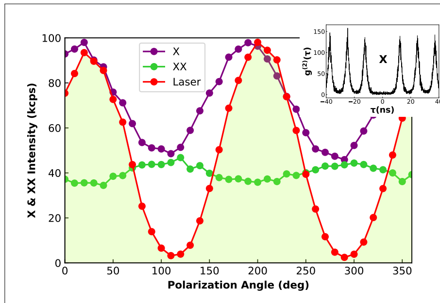
Figure 2.9: Linear polarization analysis of the detected light originating from the laser, exciton, and biexciton. The inset shows an antibunching curve collected from the exciton transition.
