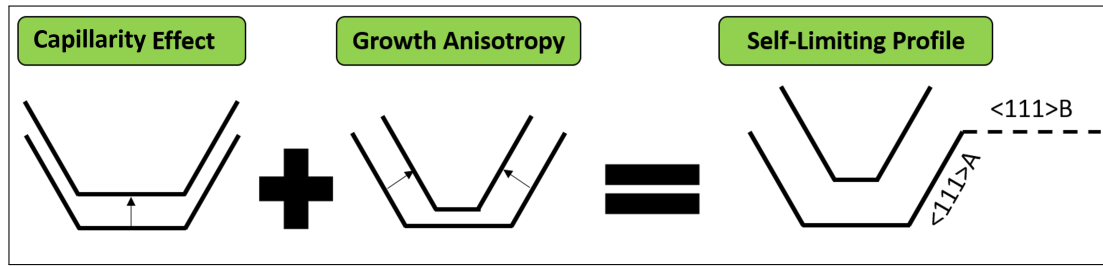
Figure 1.12: The self-limiting profile which is a balance between the capillary effect and anisotropic growth for non planar facets.
