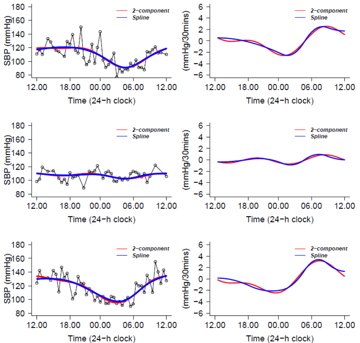
Figure 9-6 ABPM readings of three individuals with fitted subject-specific trajectories from a two-component cosinor mixed-effects model (five parameters) and spline model (six parameters - cubic spline with four knots at 18:00, 24:00, 04:00 and 08:00) (left panels). Their corresponding rate of change curves (first derivatives) are also plotted (right panels). The plots indicated an extremely similar pattern thus giving further justification of the two-component cosinor model.
