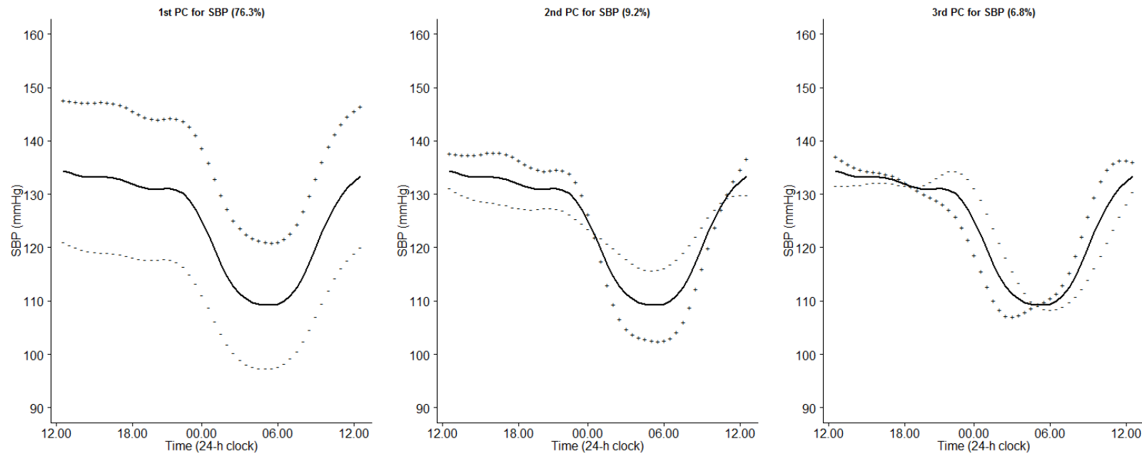
Figure 6-4 FPCA: Each of the first three FPCs as variations about the mean along with the percentage of total variation explained by the component. The solid black line represents the mean SBP over the day and the functions obtained by adding and subtracting \pm SD of the eigenfunctions to the mean. Plus signs indicate addition and minus signs indicate subtraction.
