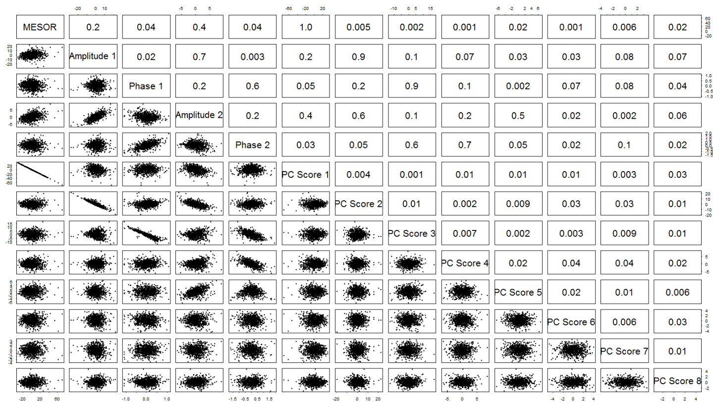
Figure 9-10 Scatter plots and the corresponding correlations between all the two-component cosinor random-effects model parameters and the principle component scores from FPCA. Eight FPCs contribute to 99% of the total variance in the data.
