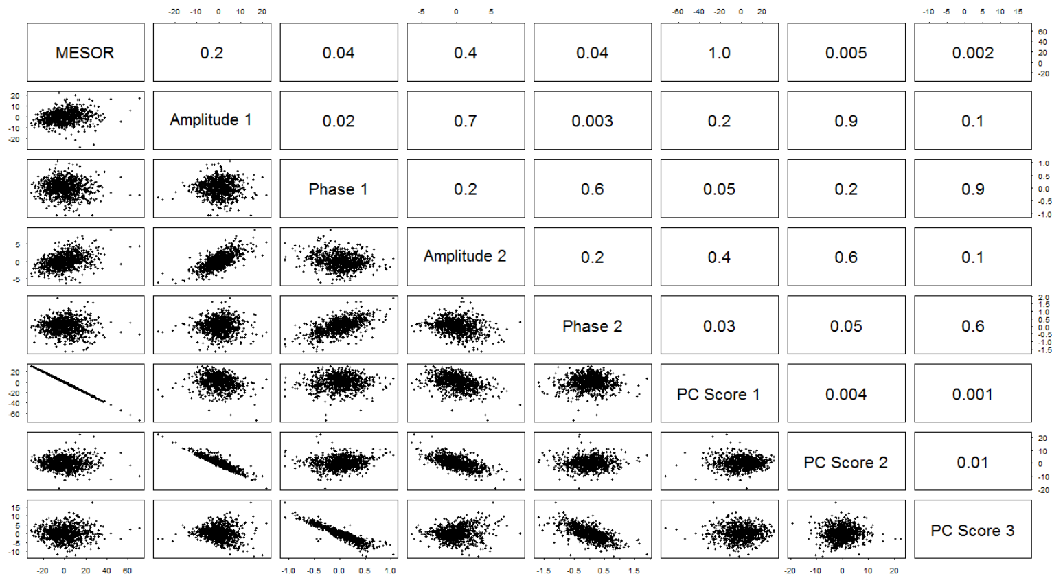
Figure 6-5 Scatter plots and the corresponding correlations between the two-component random-effects cosinor model parameters and the first three FPC scores from FPCA.
