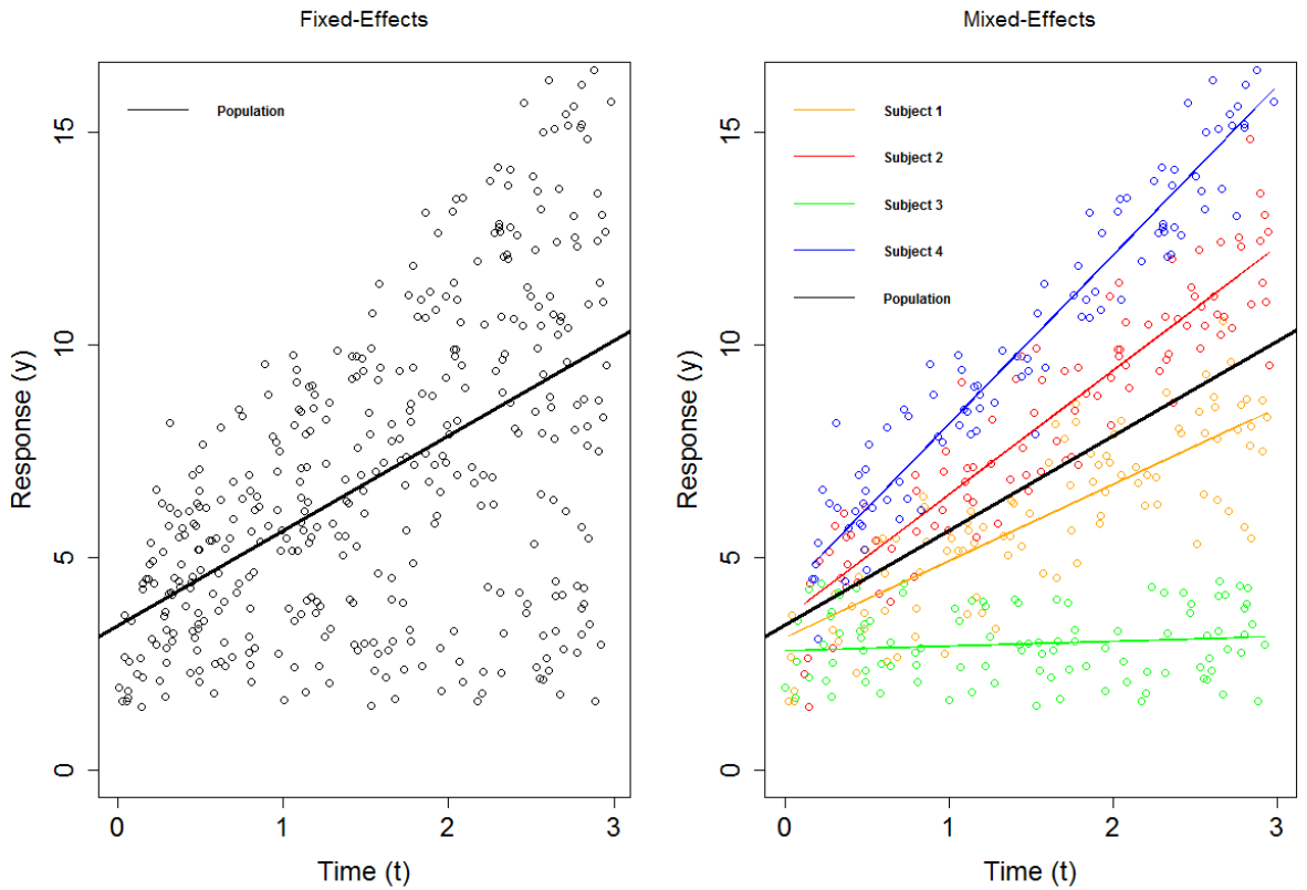
Figure 2-2 Illustration of simple linear regression model and simple linear mixed effects model where the data are clustered
