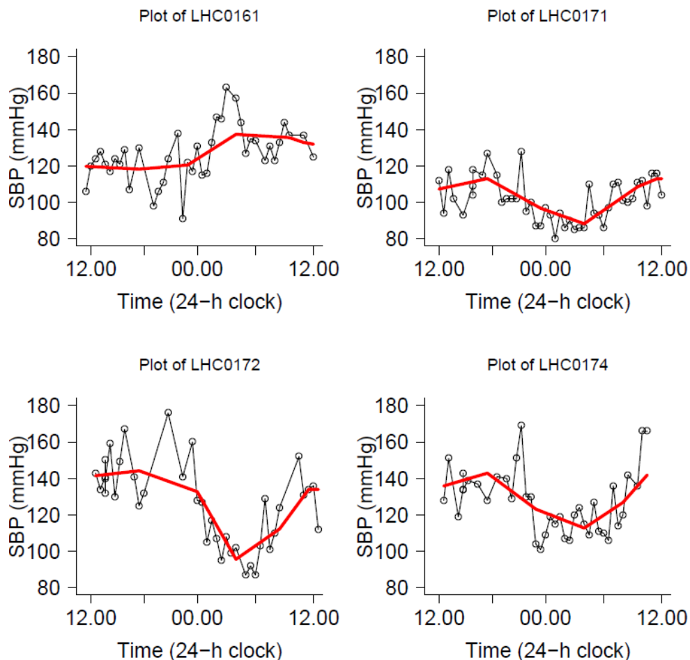
Figure 2-5 Illustration of piecewise linear splines
