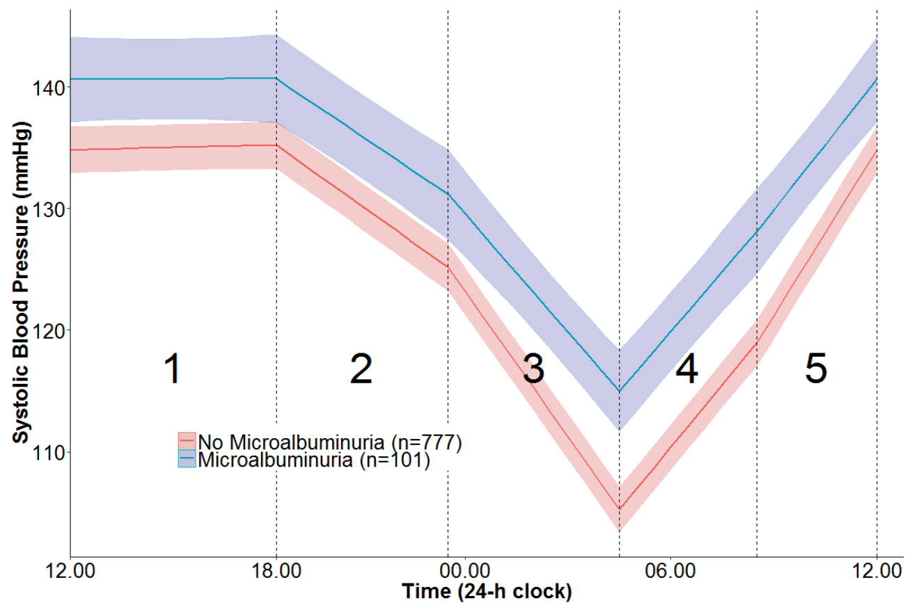
Figure 9-5 Predicted average (95% CI) piecewise linear trajectory of those with/without presence of microalbuminuria adjusted for age, sex, BMI and including an interaction of the spline terms with microalbuminuria using a linear mixed-effects model (Model 3). Each linear spline represents the rate of BP increase or decrease (slope) for that time period which is referred to in Table 5-2.
