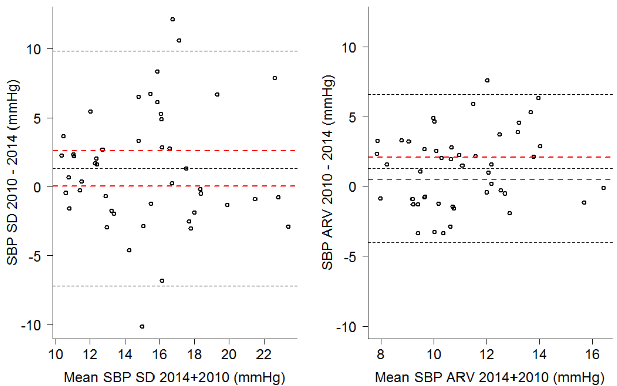
Figure 7-3 Bland-Altman scatter-plots of agreement of measurements of 24h SBP SD and 24h SBP ARV four years apart. The x-axis represents the mean of the two measurements and the y-axis represents the difference between them. The black dashed lines represent the mean and limits of agreement. The dashed red lines represent the 95%CI for the differences in mean values.
