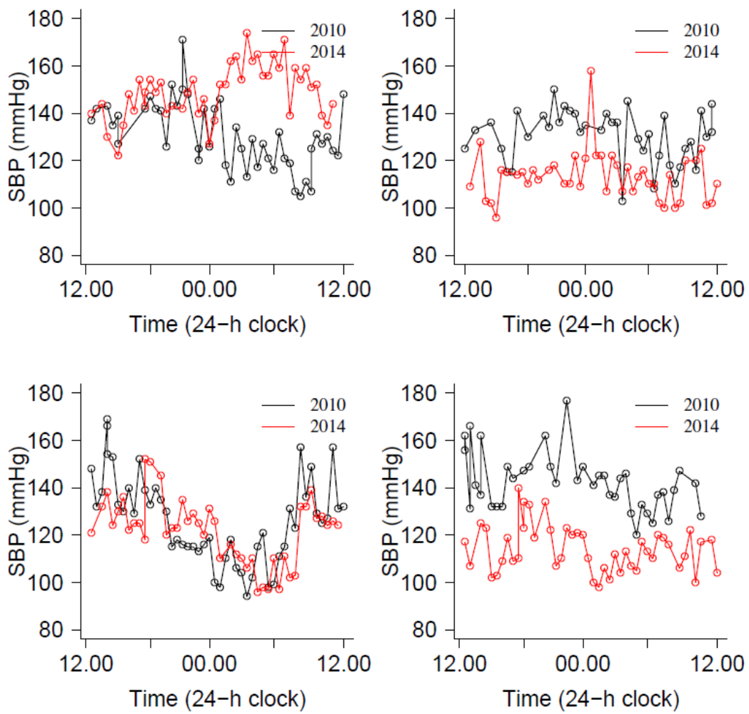
Figure 7-1 Data from four individuals 2010 vs 2014
