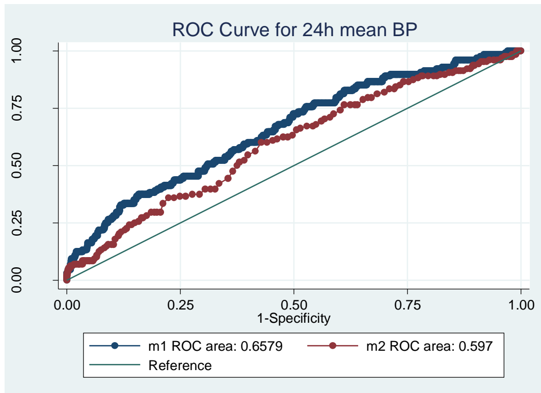
24-h mean BP ROC curve. M1: 24-h mean BP, clinic BP; M2: clinic BP (p-value=0.01)
