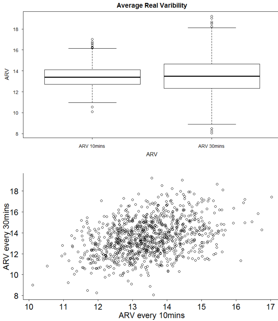
Figure 9-11 Simulated ARV values taken every 10mins and every 30mins.
