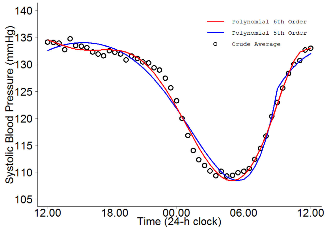
Figure 9-1 Population Level Effects for polynomial regression (Chapter 2)
