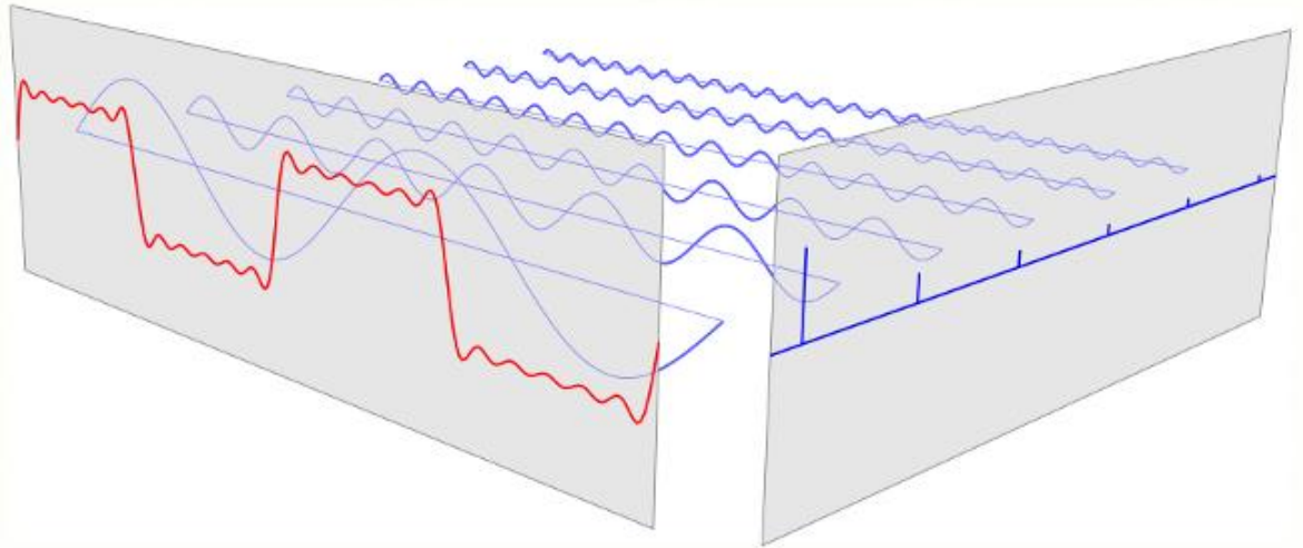
Figure 2-7 Fourier series – a linear combination of sines and cosines can produce a complex curve [127].
