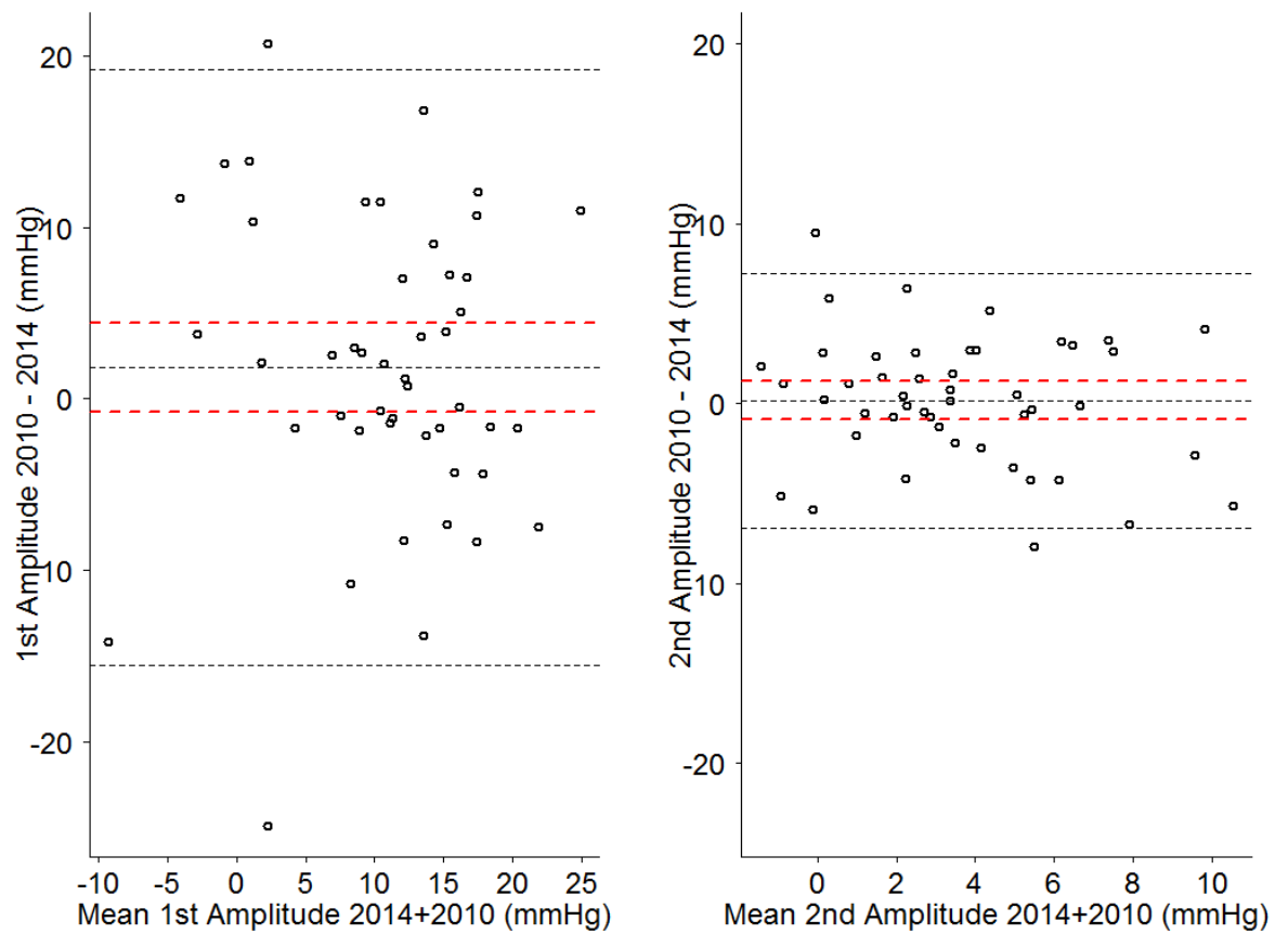
Figure 7-4 Bland-Altman scatter-plots of agreement of measurements of the first and second amplitudes four years apart. The x-axis represents the mean of the two measurements and the y-axis represents the difference between them. The black dashed lines represent the mean and limits of agreement. The dashed red lines represent the 95%CI for the differences in mean values.
