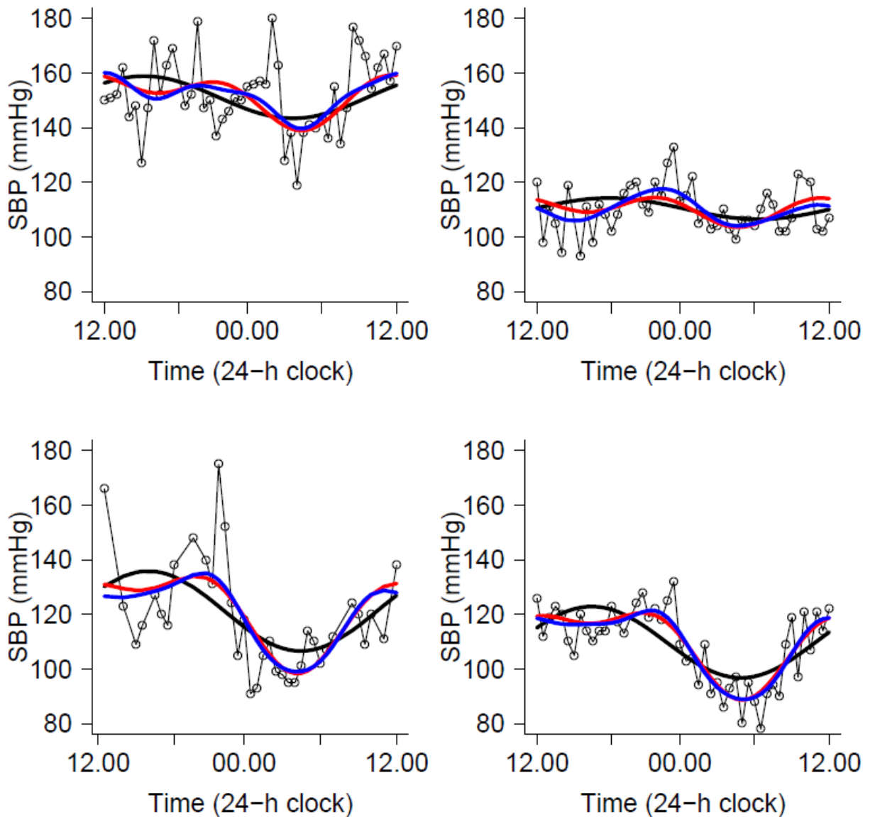
Figure 6-1 ABPM readings (circles, thin black line) of four individuals along with predicted subject-specific trajectories from a random-effects model as a function of time using (i) single cosinor (thick black line) (ii) two-component cosinor (thick red line) and (iii) three-component cosinor (thick blue line) models.
