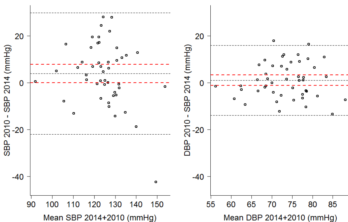
Figure 7-2 Bland-Altman scatter-plots of agreement of measurements of 24h SBP and 24h DBP four years apart. The x-axis represents the mean of the two measurements and the y-axis represents the difference between them. The black dashed lines represent the mean and limits of agreement. The dashed red lines represent the 95%CI for the differences in mean values.
