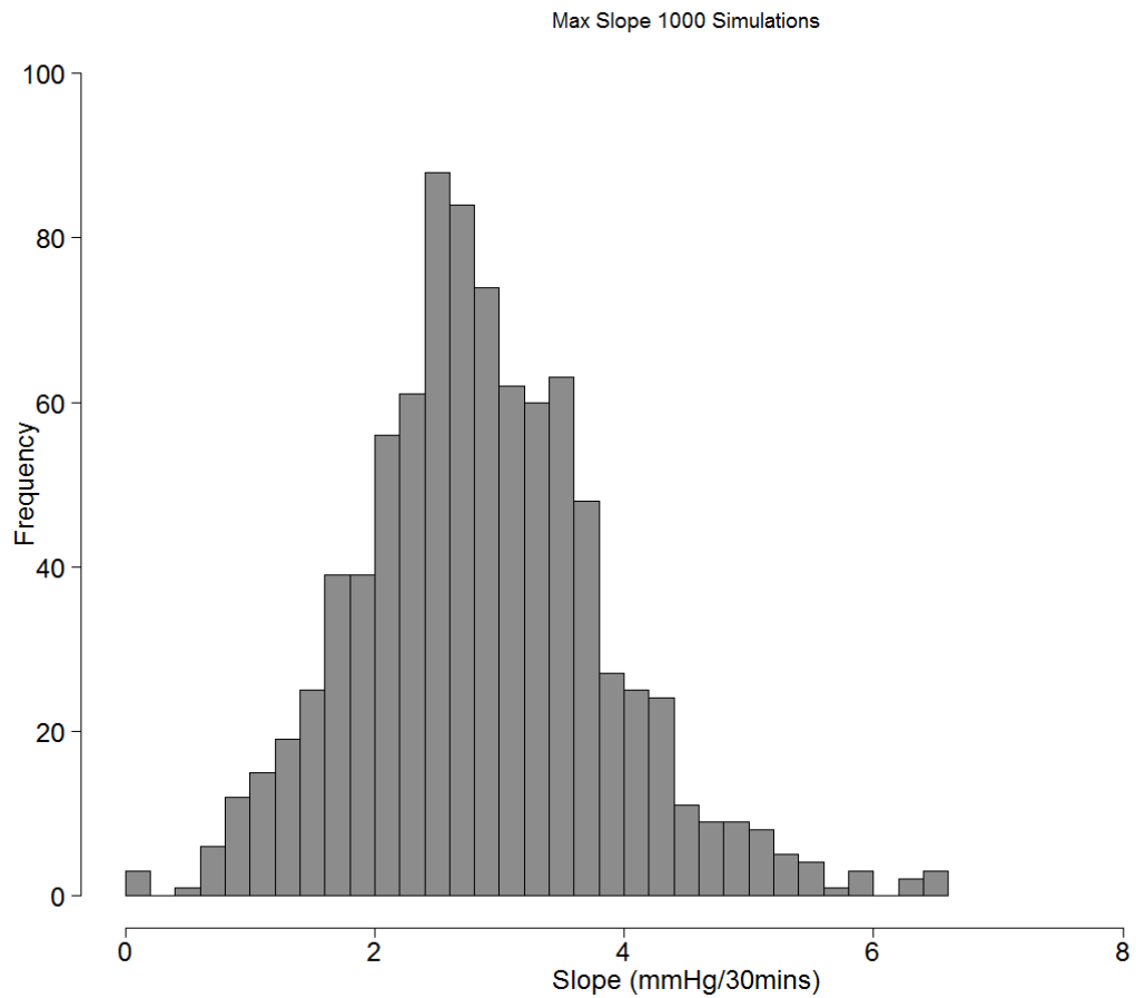
Figure 6-3 Histograms of maximum morning slope by simulations
