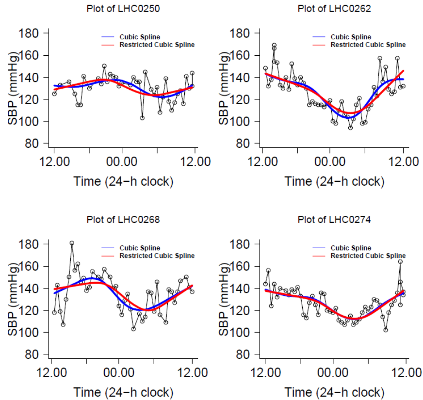
Figure 2-4 Illustration of cubic and restricted splines
