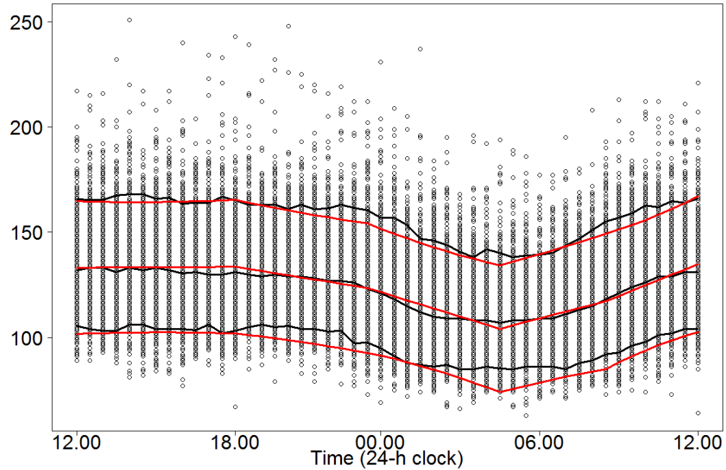
Figure 9-4 VPC (visual predictive check) plot. Black lines represent median of observed data with 90% interquartile range of observations. Red line is predicted mean along with 90% prediction interval.
