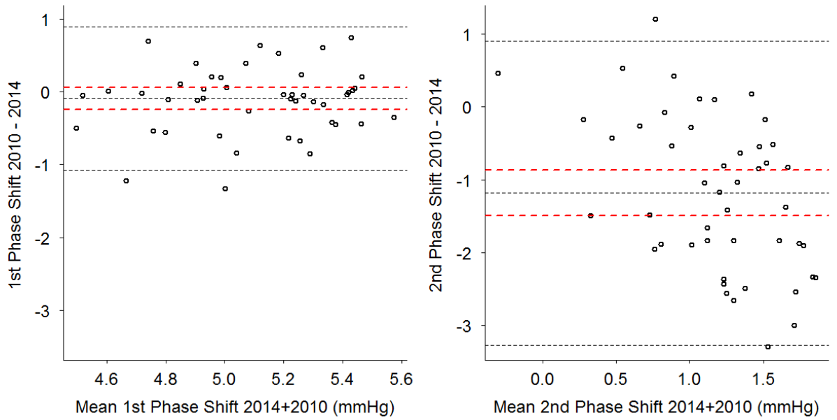
Figure 7-5 Bland-Altman scatter-plots of agreement of measurements of the first and second phase shifts four years apart. The x-axis represents the mean of the two measurements and the y-axis represents the difference between them. The black dashed lines represent the mean and limits of agreement. The dashed red lines represent the 95%CI for the differences in mean values.
