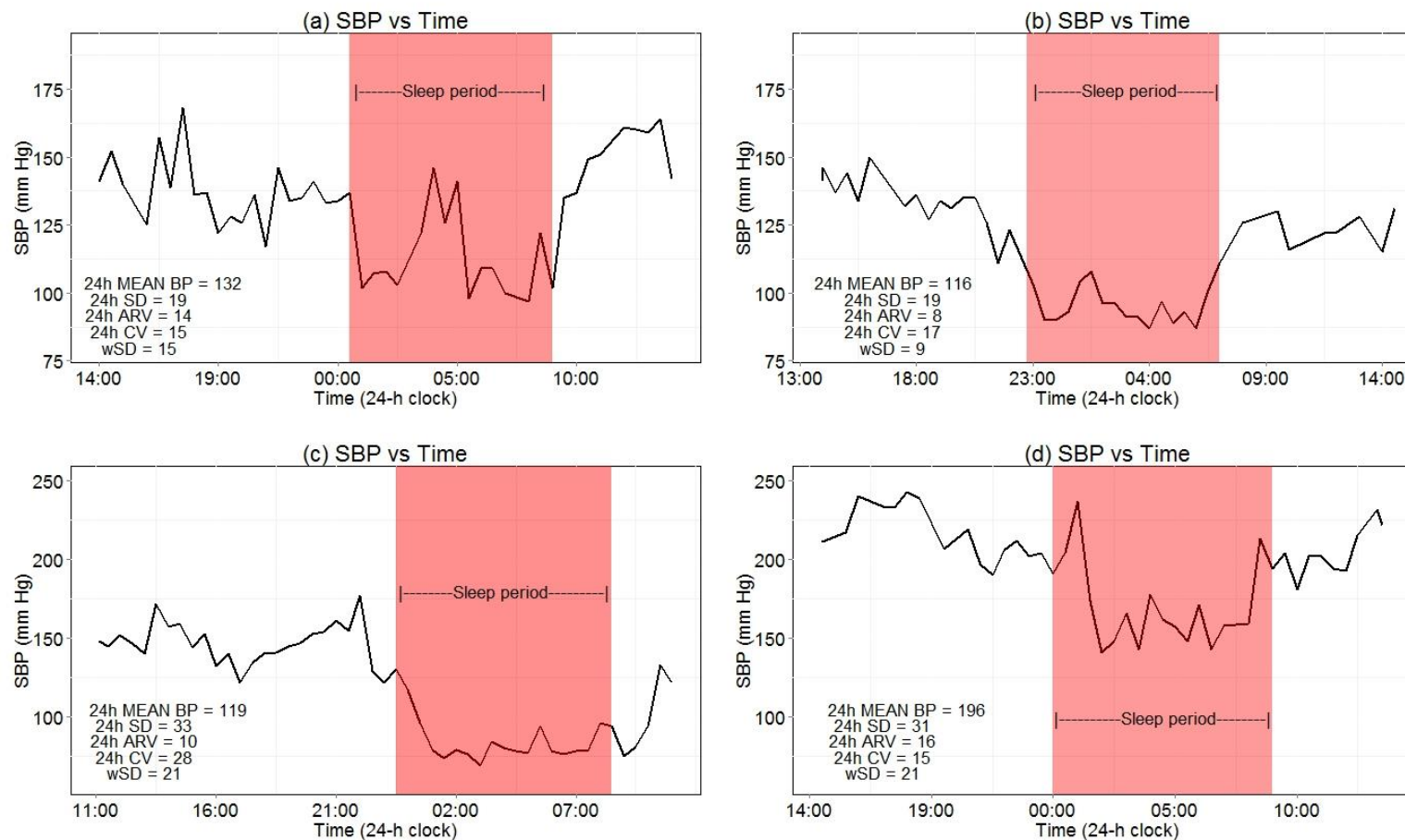
Figure 4-1 Four study participants and their 24h BP profiles. Panels (a) & (b) illustrate different patterns yet have similar 24h SD but different values based on the other indices. Both (c) & (d) demonstrate a similar issue (values rounded).
