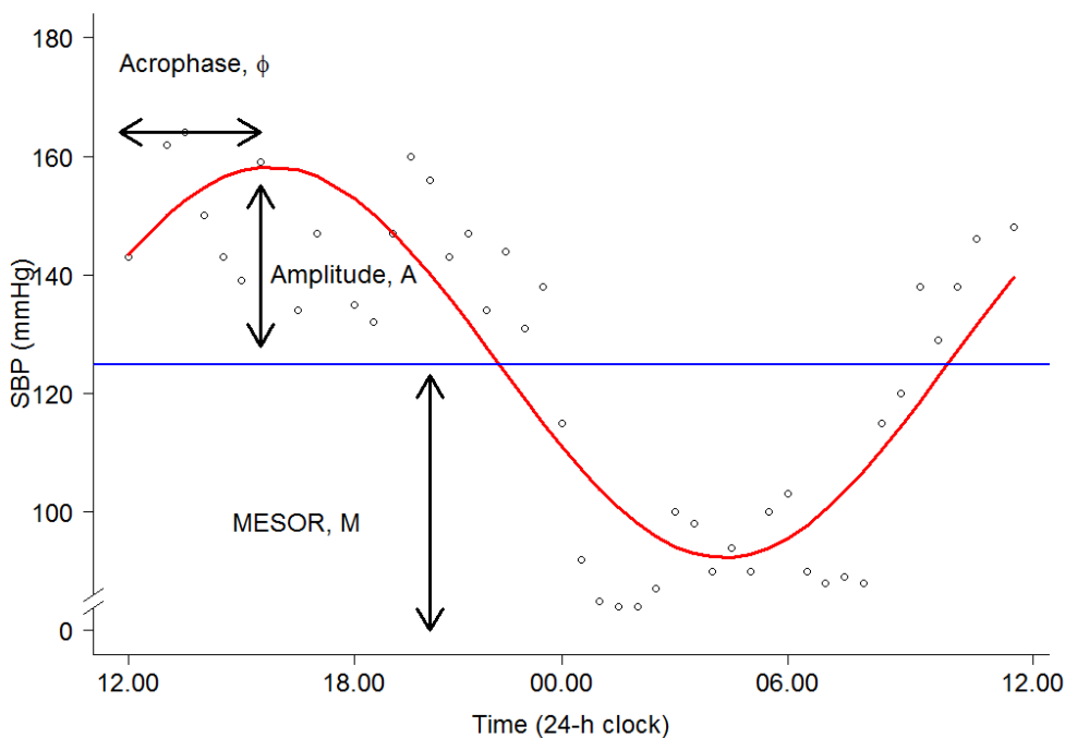
Figure 2-6 A simple cosinor fit to observed SBP readings of an individual (period=24h)
