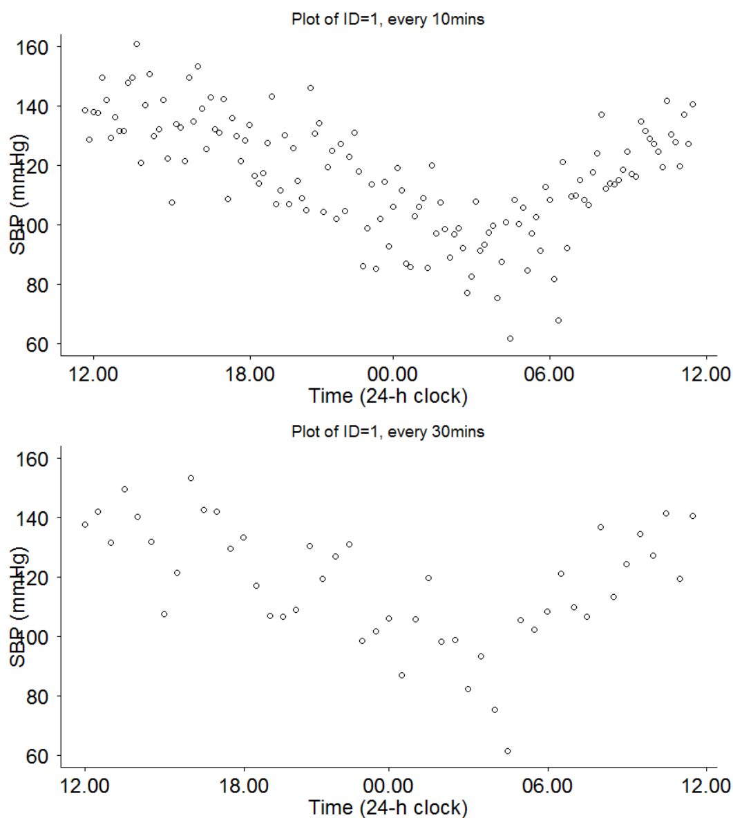
Figure 9-12 Simulated data for one individual with readings taken 1) every 30min and 2) every 10mins.
