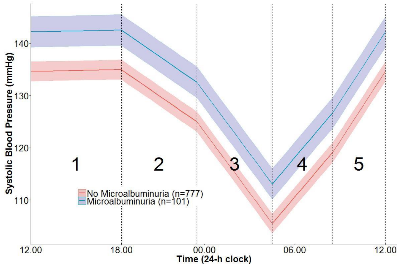
Figure 5-3 Predicted average (95% CI) piecewise linear trajectory of those with/without presence of microalbuminuria adjusted for age, sex and BMI using a linear mixed-effects model (Model 2). Each linear spline represents the rate of SBP increase or decrease (slope) for that segment and has been given a corresponding number which is referred to in Table 5-2. For the purposes of this plot we have set the sleep and wake time knots at 23.00 and 08.00 respectively.
