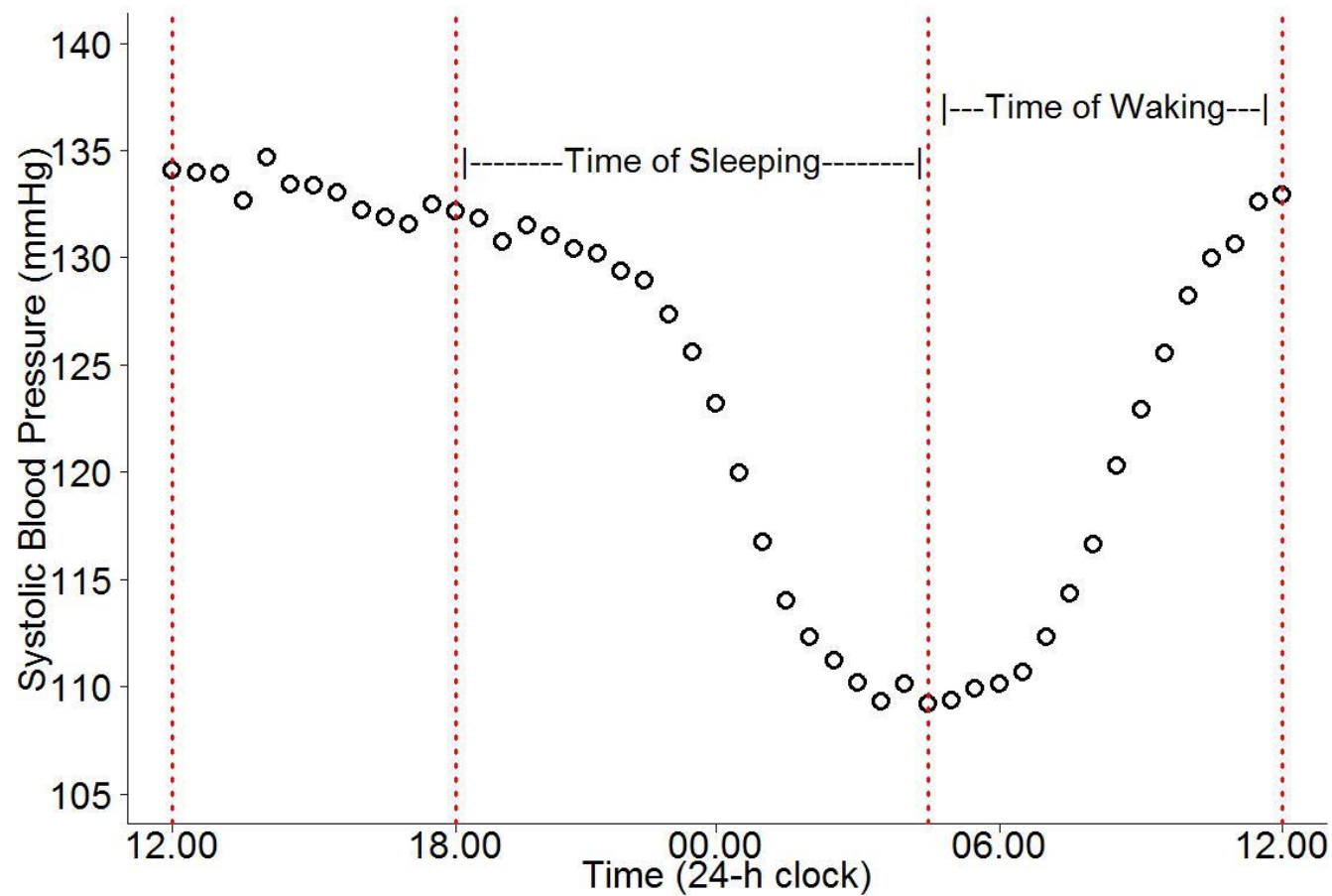
Figure 5-1 Plot of average SBP over 24h which helped identify 6pm and 4am as common knot points for all participants where there was a notable change in trajectory of BP. Also highlighted are the periods where individuals woke and went to sleep. In addition to the two common points, we were able to obtain additional (two) subject-specific knot points at wake and sleep times.
