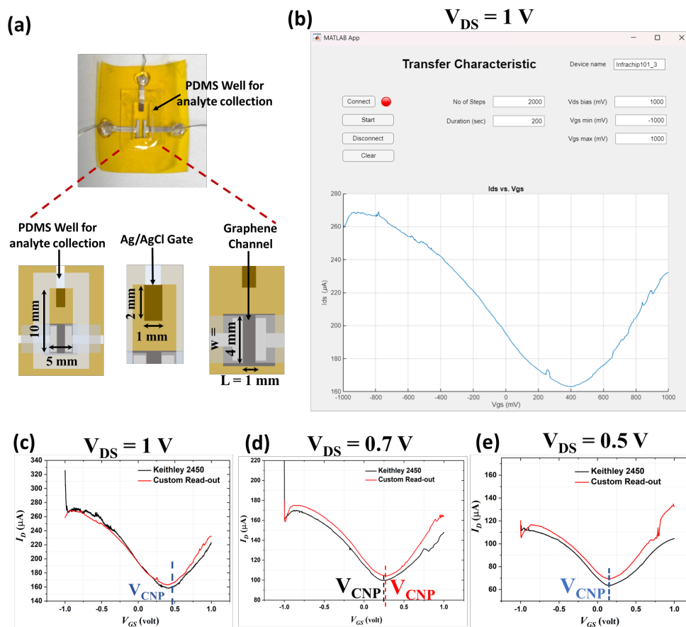
Fig. 2. (a) Fabricated Gr-FET with its geometrical dimensions (b) Screenshots of the user-interface window showing transfer characteristics ( I_D vs. V_{GS} ) of the Gr-FET device with drain voltage V_{DS} = 1 V measured using the Custom Readout Module. (c-e) Comparison of transfer characteristics obtained using a Keithley 2450 source meter (black) and the Custom Readout Module (red), with different drain voltages ( V_{DS} = 1 V, 0.7 V, and 0.5 V.).
