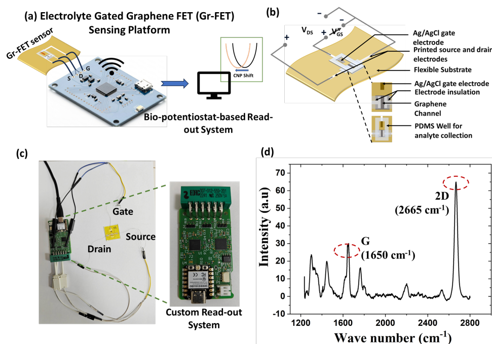
Fig. 1. (a) Schematic illustration of a wireless, miniaturized readout system for acquiring the transfer characteristics of a graphene field-effect transistor (Gr-FET), (b) Design of the flexible Gr-FET device showing source (S), drain (D), and gate (G) electrodes with applied biases, (c) Photograph of the fabricated device connected to the custom portable measurement unit for electrical characterization. (d) Raman spectrum of graphene channel at 632 nm excitation.
