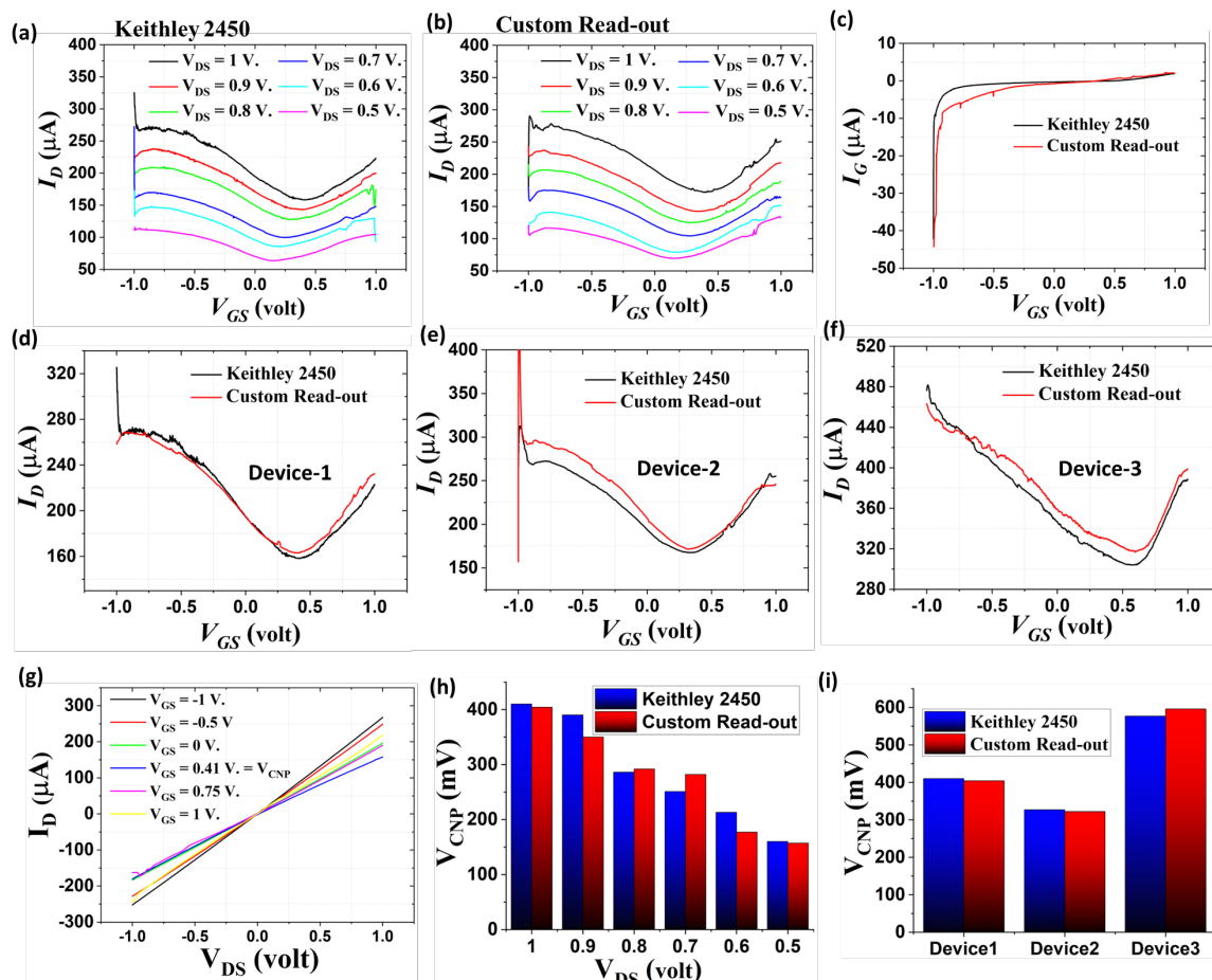
Fig. 3. (a) Transfer characteristics of a graphene FET measured at different drain biases ( V_{DS} ) using a Keithley 2450 source meters, (b) corresponding transfer characteristics measured using the Custom Readout Module under identical bias conditions, showing comparable trends, (c) comparison of gate leakage current trends for Ketley 2450 and Custom Readout Module (d–f) Direct comparison of transfer characteristics for three different devices (Device-1, Device-2, and Device-3), measured using the Keithley 2450 source meter (black) and the Custom Readout Module (red), (g) output characteristics of Device-1 with different drain to source voltages V_{DS} .
