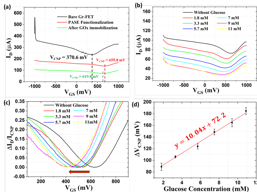
Fig. 4. (a) Transfer characteristics of the graphene FET at different functionalization stages: bare device, after PASE functionalization, and after glucose oxidase (GOx) immobilisation, (b) transfer characteristics of the functionalized Gr-FET device at varying glucose concentrations, (c) transfer characteristics with the normalised current response ( \Delta I_D/I_{CNP} vs V_{GS} ) to show the shift in V_{CNP} with varying glucose concentration, (d) calibration curve showing the shift in charge neutrality point ( \Delta V_{CNP} ) as a function of glucose concentration, exhibiting a linear response.
