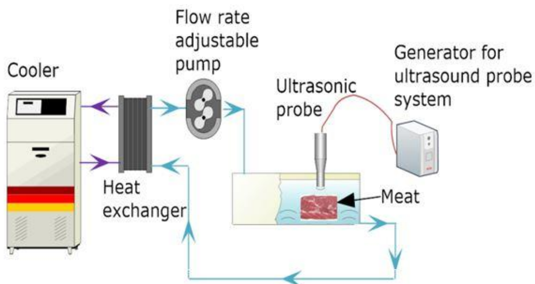
Figure 2. Schematic diagram of experimental set-up. The system used was composed of a refrigerated circulator (cooler), through which glycol coolant ( -0.5^{\circ}\text{C} ) was circulated using a heat exchanger and a pump, The meat sample was fixed horizontally onto a basket in a tank filled with 15% brine solution. Ultrasound (US) with a frequency of 20 kHz was irradiated onto the sample for 60 minutes by using an ultrasonic processor.
