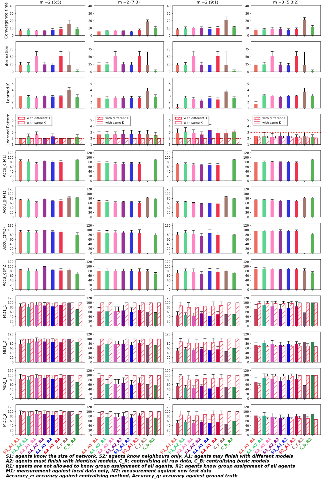
Figure 8.31: K-means on sparse network with multiple patterns and partially symmetric multi-dimensional Gaussians
