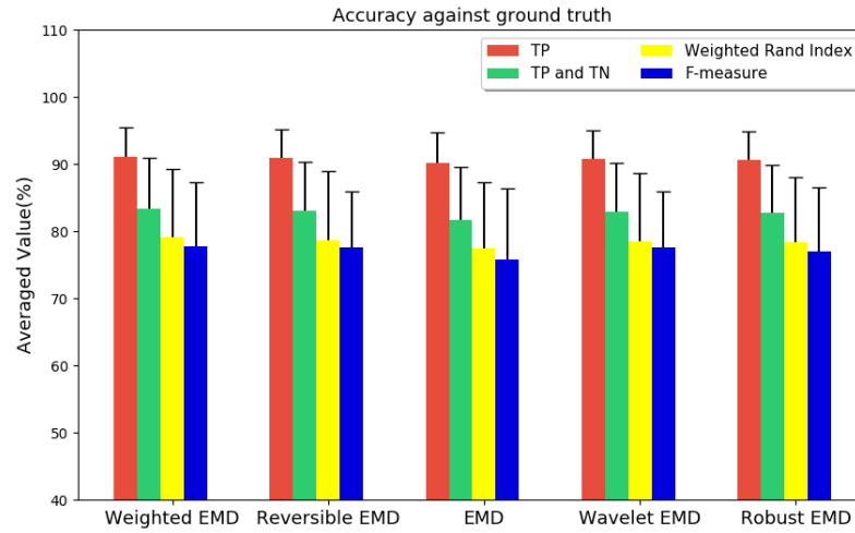
Figure 8.15: Accuracy against ground truth with fully symmetric Gaussians
