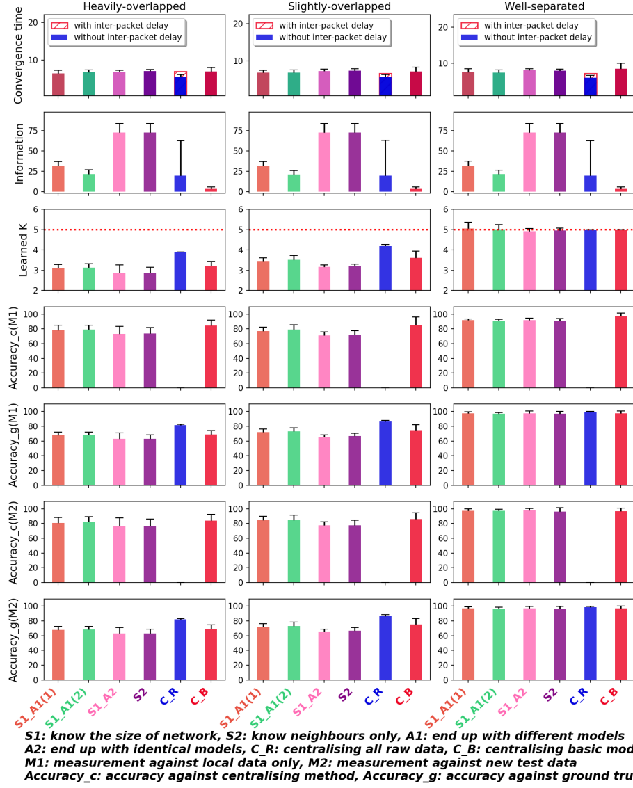
Figure 4.7: K-means on dense network with asymmetric multi-dimensional Gaussians
