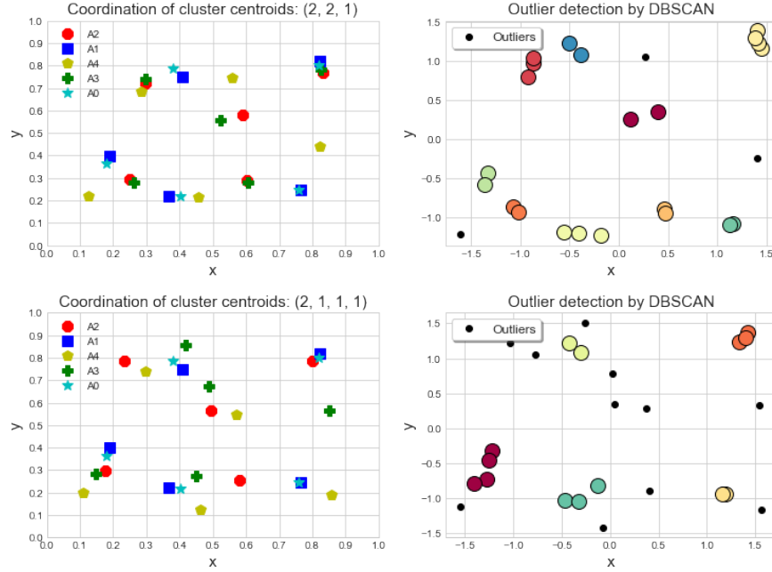
Figure 6.5: Application of DBSCAN to agents' clusters (2)
