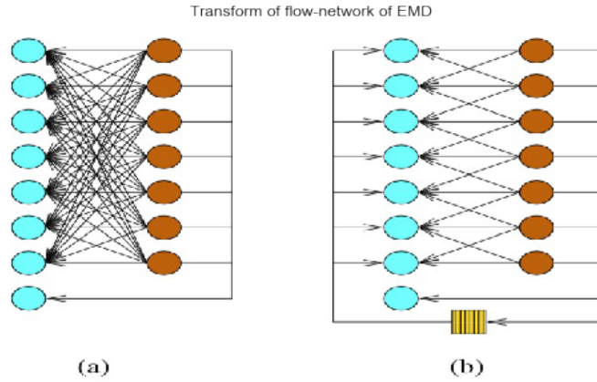
Figure 2.13: Robust EMD [Pele and Werman, 2009]
