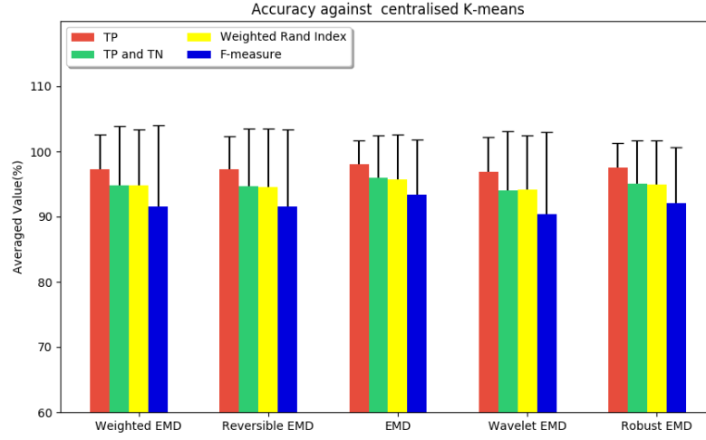
Figure 5.11: Accuracy measures against centralised k-means with symmetric Gaussians
