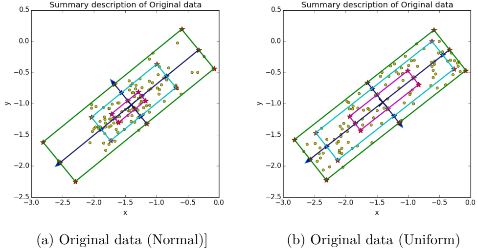
Figure 8.1: Data generated by normal and uniform in same range
