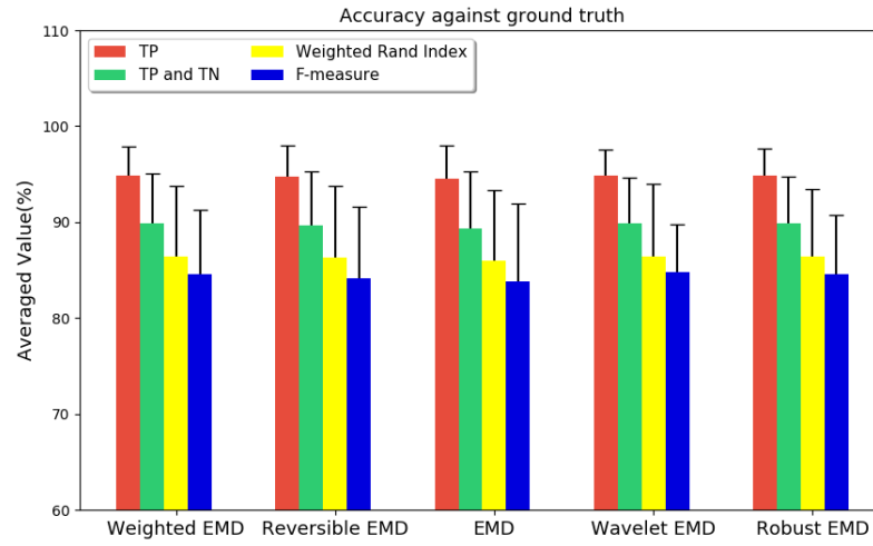
Figure 8.21: Accuracy against ground truth with fully symmetric Gaussians
