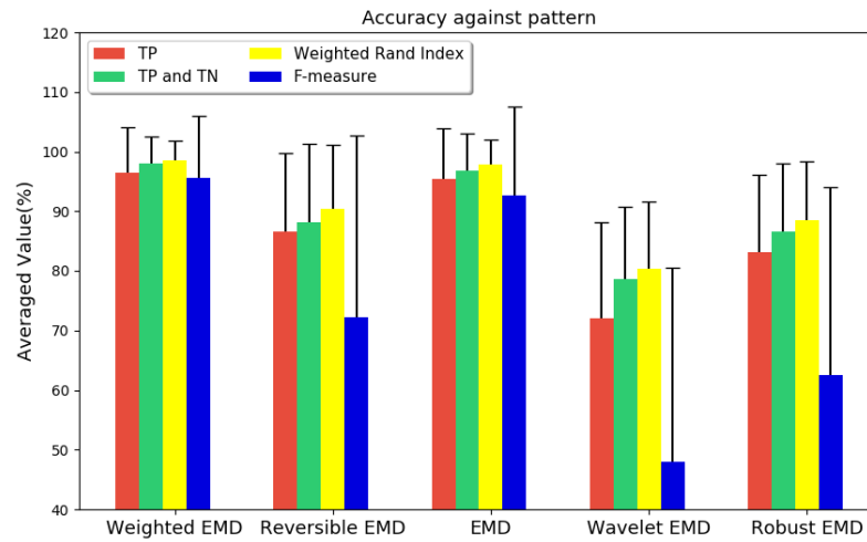
Figure 8.22: Accuracy against pattern with fully symmetric Gaussians
