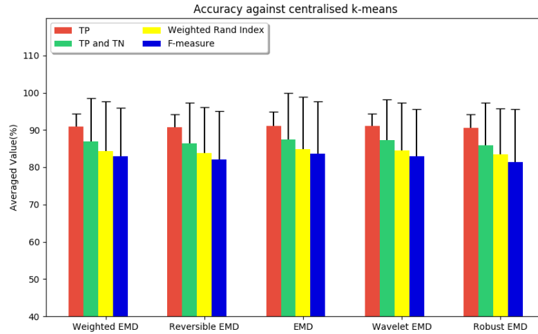
Figure 5.17: Accuracy against centralised k-means with uniformly distributed dataset
