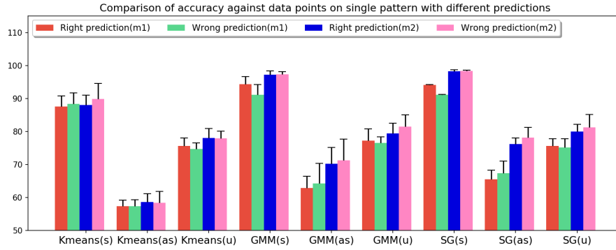
Figure 6.19: Accuracy against data points achieved by Optimised KDE when ground truth pattern is single
