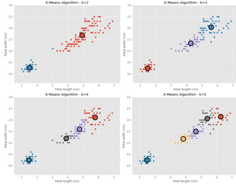
Figure 2.8: Clustering with different number of clusters on Iris dataset
