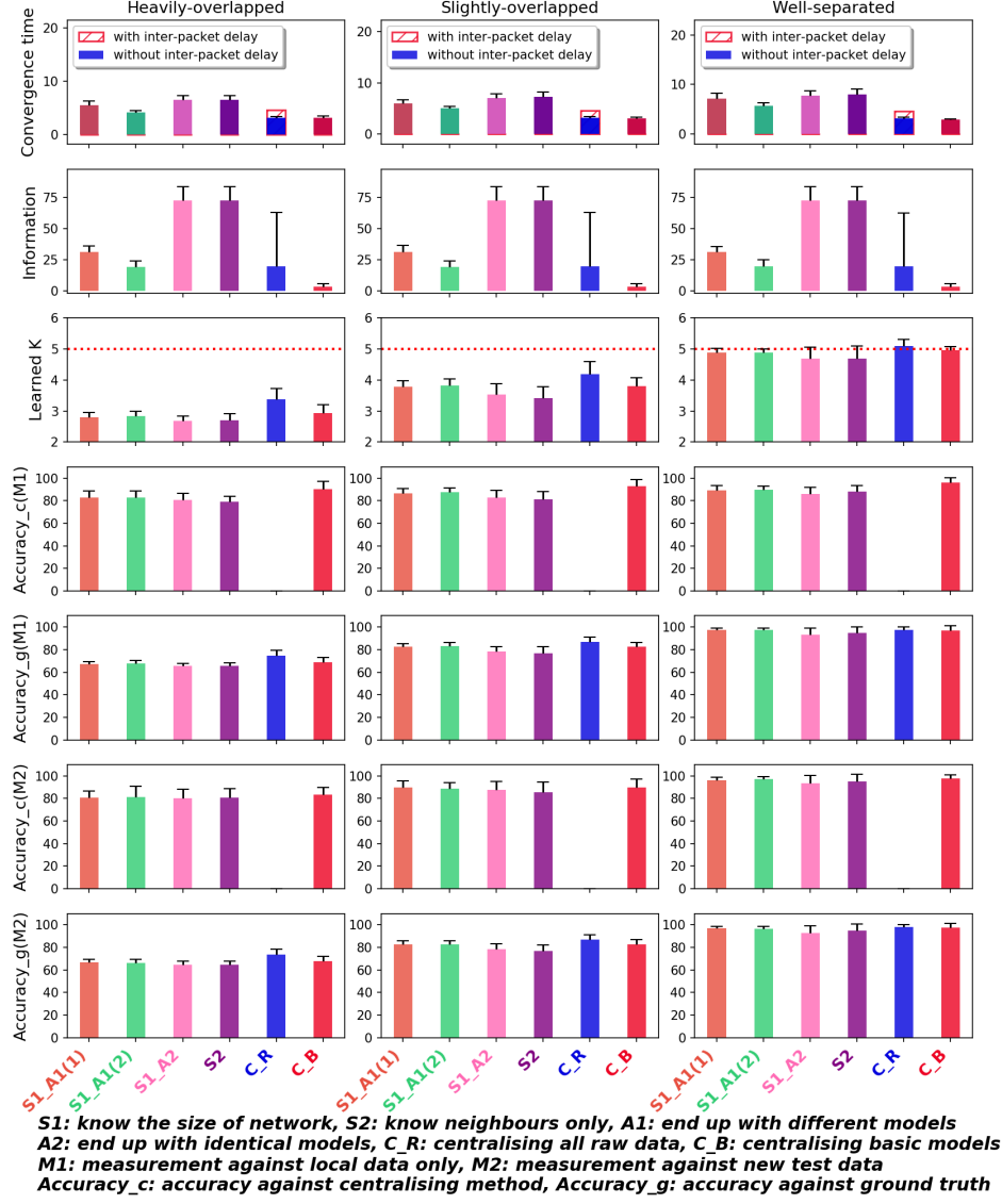
Figure 4.14: GMM on dense network with uniform distributed dataset
