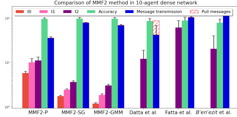
Figure 3.6: MMF2 method in 10-agent dense networks
