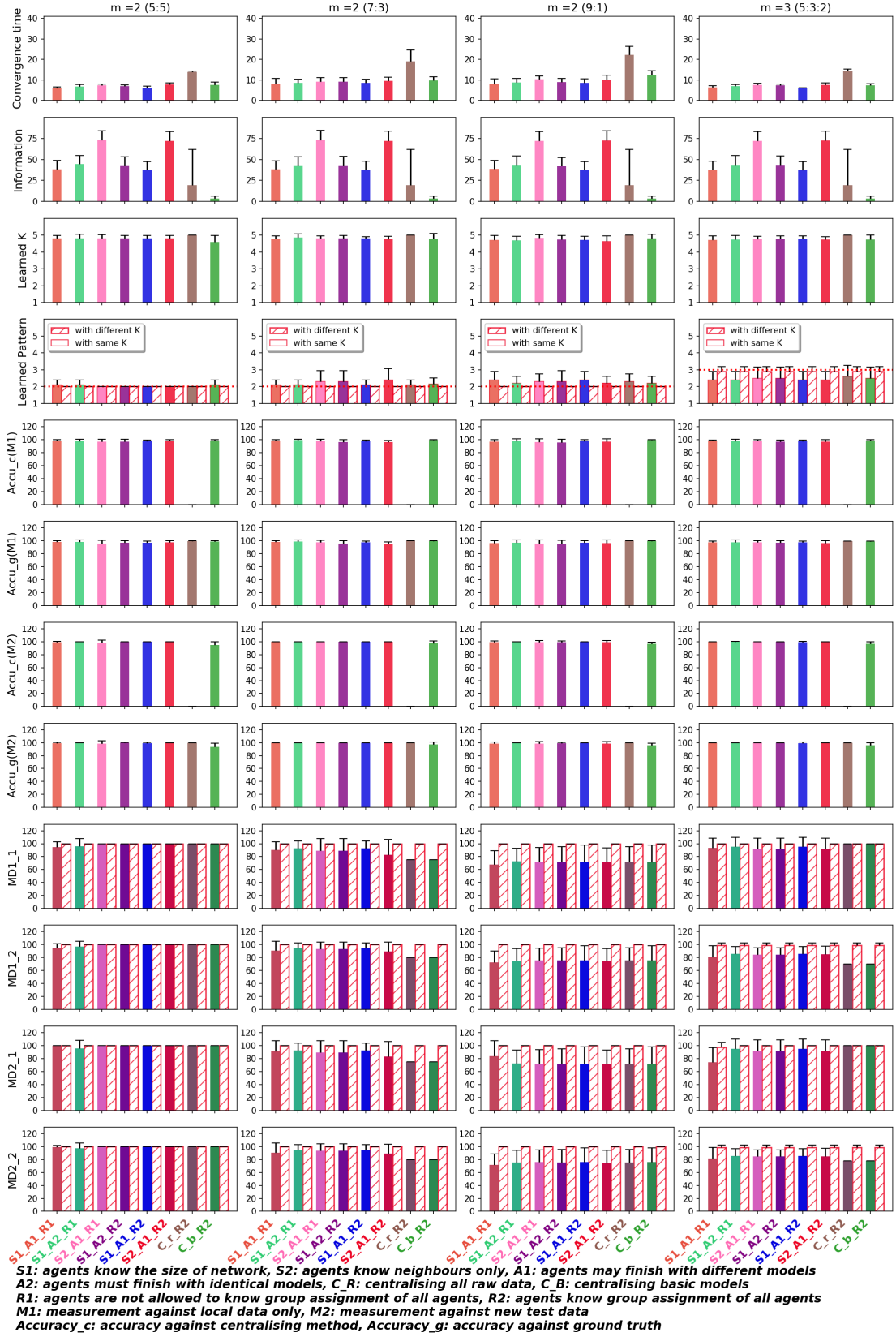
Figure 5.24: K-means on multiple patterns dense network with fully symmetric well separated clusters
