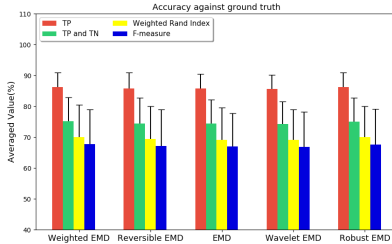
Figure 8.18: Accuracy against ground truth with uniformly distributed dataset
