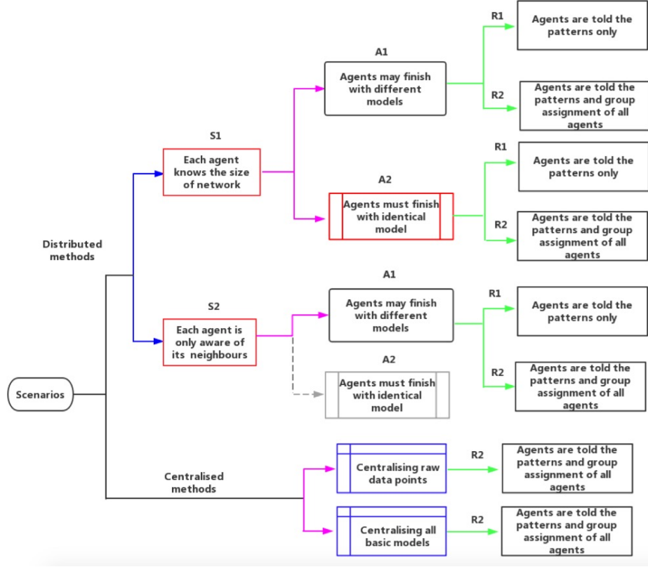
Figure 5.21: Different scenarios considered for multiple patterns
