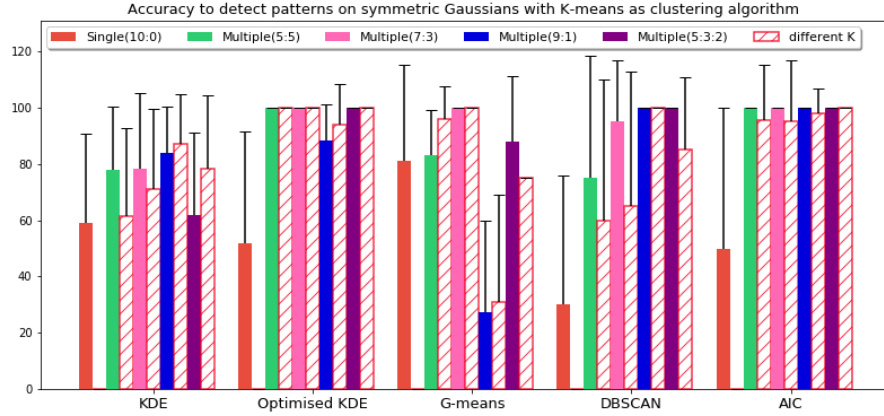
Figure 6.10: Accuracy achieved with symmetric Gaussians when K-means is used
