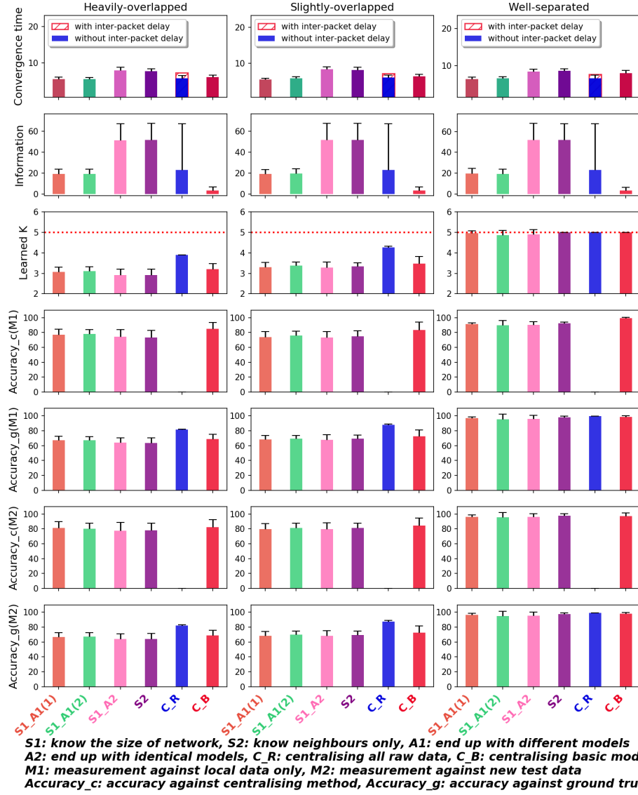
Figure 8.6: K-means on sparse network with partially symmetric Gaussians
