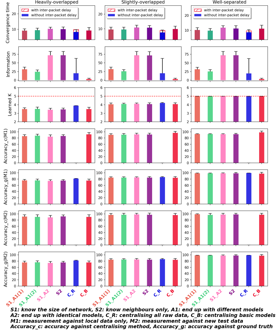
Figure 4.10: SG on dense network with asymmetric multi-dimensional Gaussians
