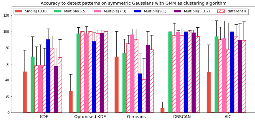
Figure 6.13: Accuracy achieved with symmetric Gaussians when GMM is used
