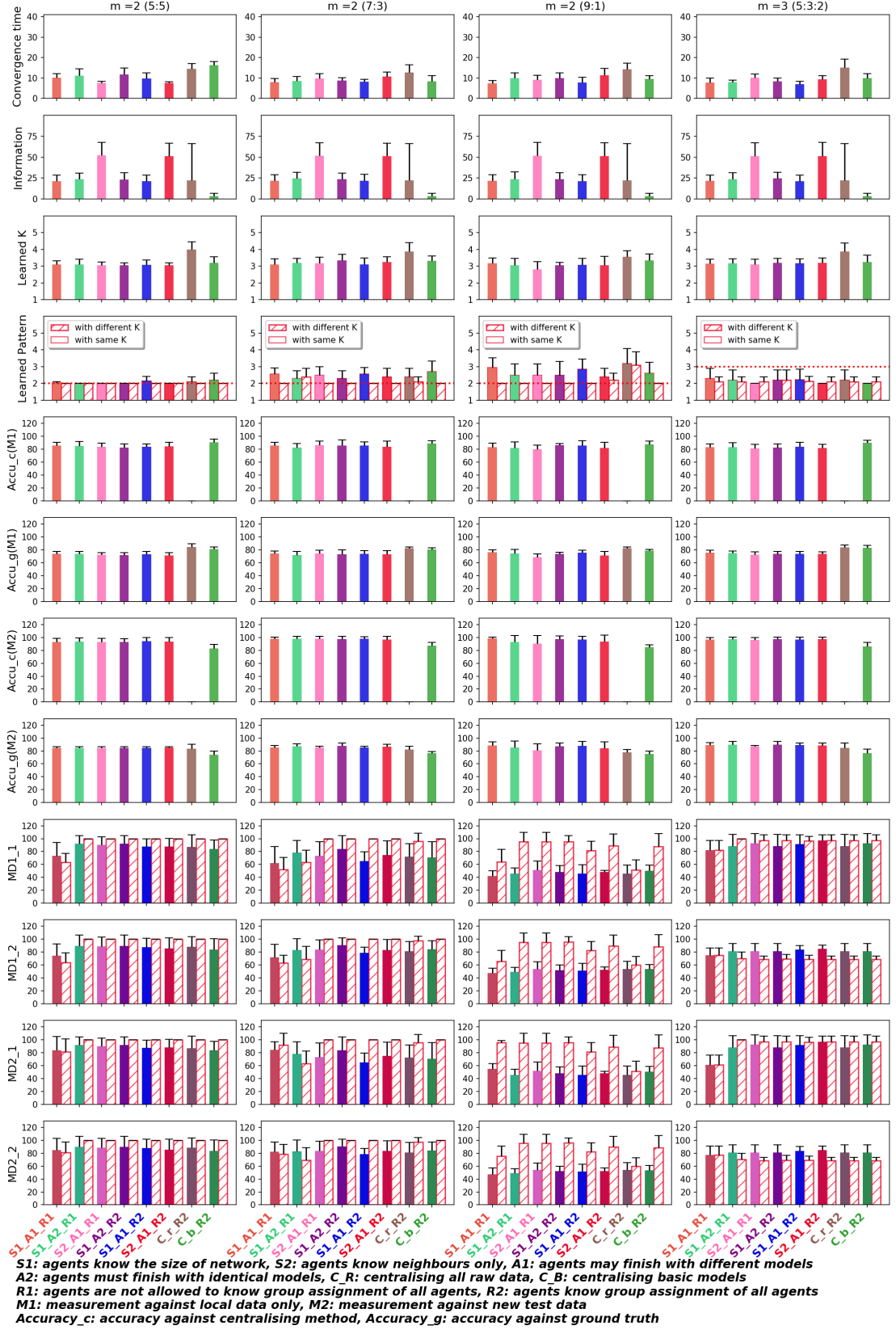
Figure 8.37: SG on sparse network with multiple patterns and partially symmetric multi-dimensional Gaussians
