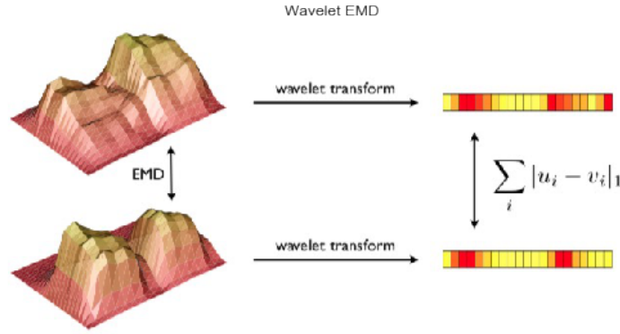
Figure 2.12: Wavelet EMD [Shirdhonkar and Jacobs, 2008]
