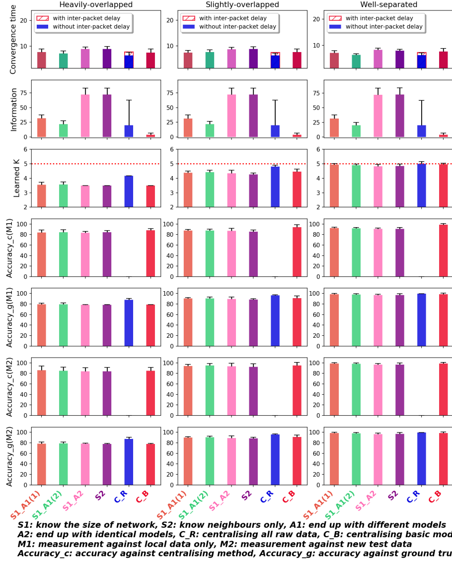
Figure 4.6: K-means with symmetric multi-dimensional Gaussians on dense network
