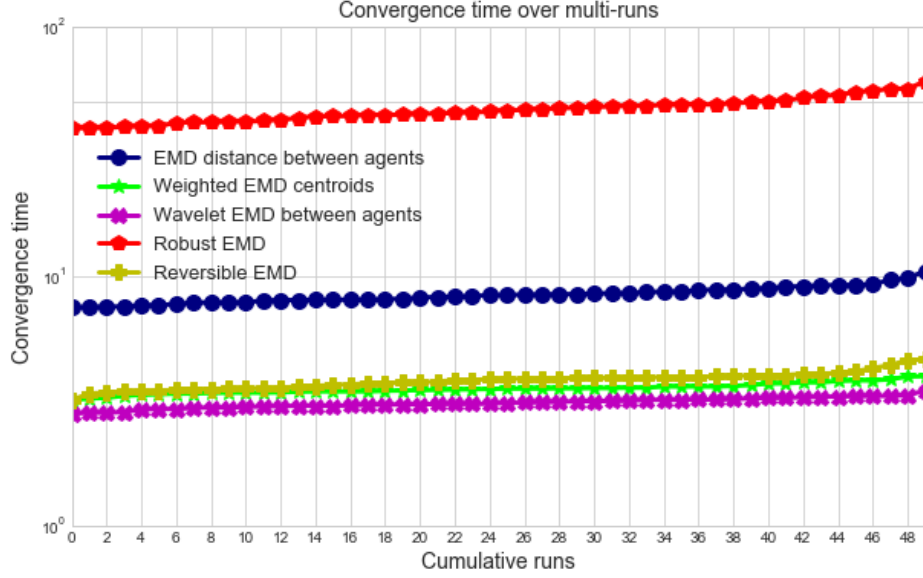
Figure 5.20: Comparison of convergence time
