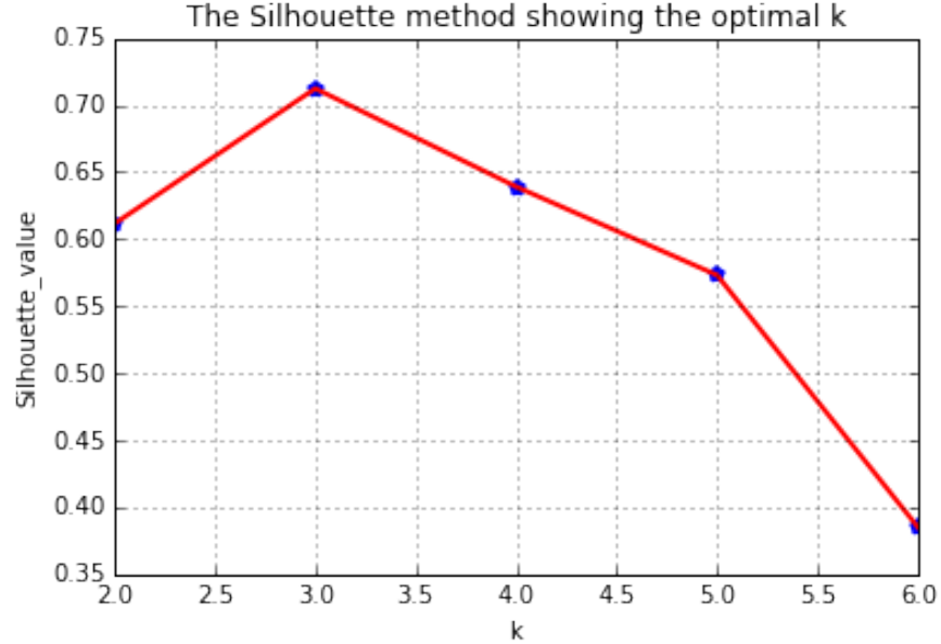
Figure 2.11: Number of clusters found by silhouette
