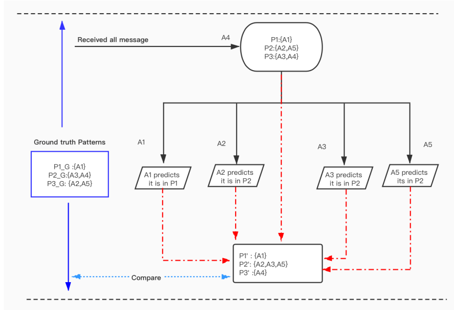
Figure 5.22: Symmetric table built by agents' prediction
