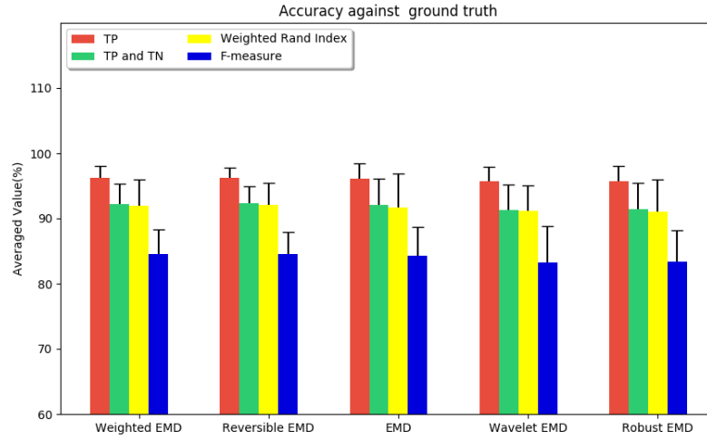
Figure 5.12: Accuracy against ground truth with symmetric Gaussians
