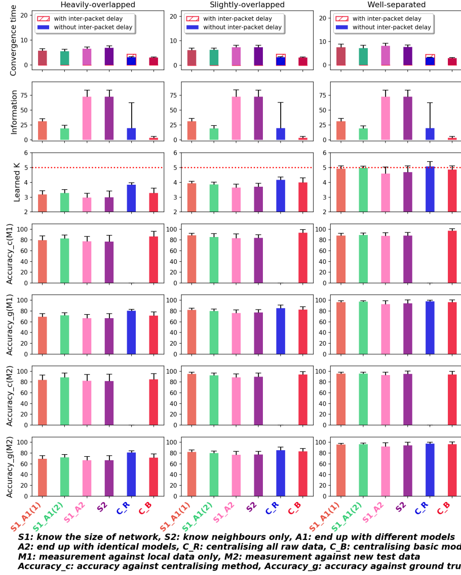
Figure 4.13: GMM on dense network with asymmetric multi-dimensional Gaussians
