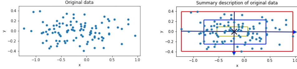
Figure 3.2: Original data and its summary description
