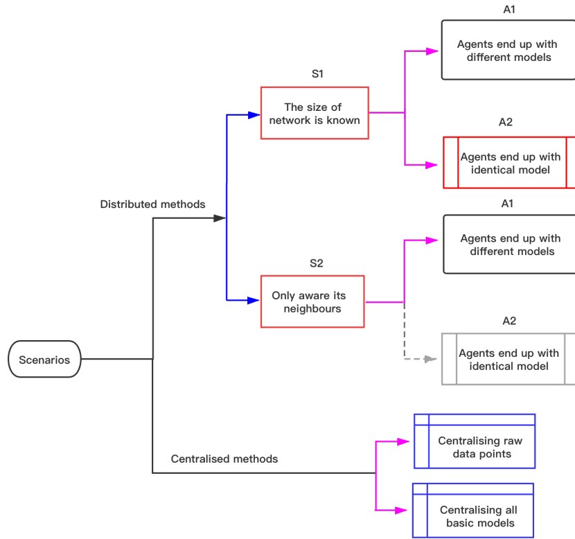
Figure 4.1: Different scenarios considered in this chapter
