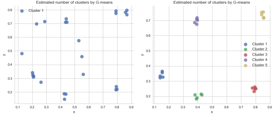
Figure 6.3: Application of G-means to agents' clusters
