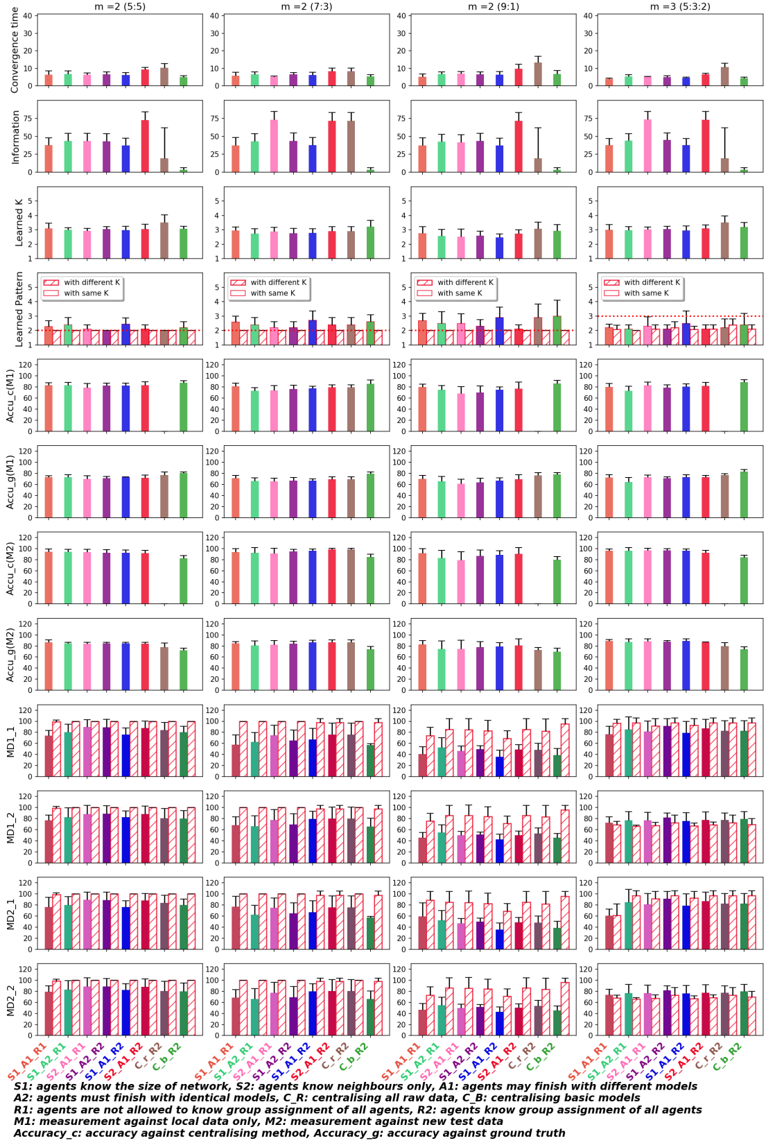
Figure 5.31: GMM on dense network with multiple patterns and asymmetric multi-dimensional Gaussians
