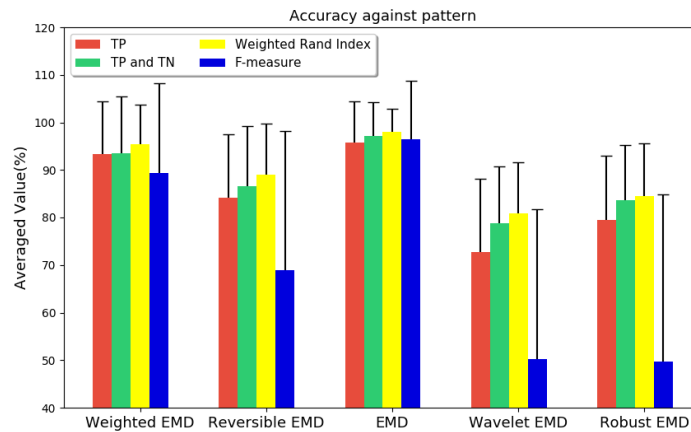
Figure 8.25: Accuracy against pattern with uniformly distributed dataset
