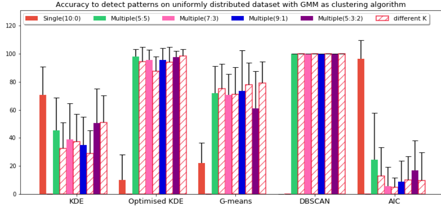
Figure 6.15: Accuracy achieved with uniformly distributed dataset when GMM is used
