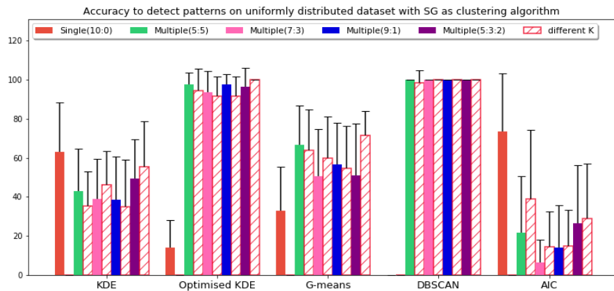
Figure 6.18: Accuracy achieved with uniformly distributed dataset when SG is used
