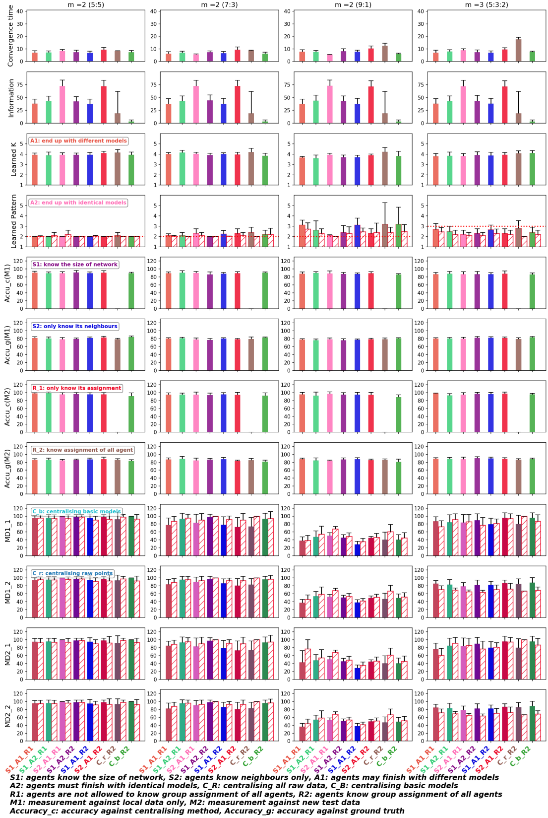
Figure 5.32: GMM on dense network with multiple patterns and uniformly distributed dataset
