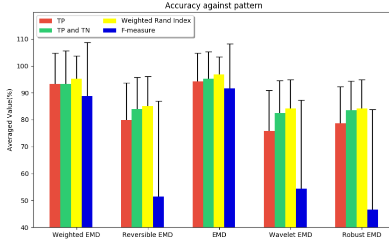
Figure 5.19: Accuracy against pattern with uniformly distributed dataset
