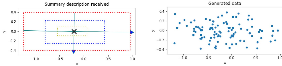
Figure 3.3: Bounding boxes received and regenerated data based on it
