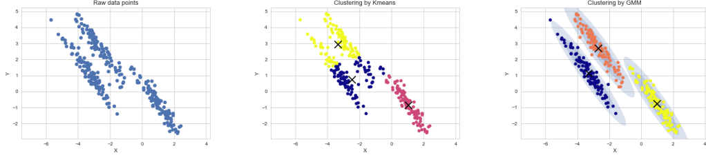
Figure 2.4: Comparison of K-means and GMM when underlying dataset is generated by asymmetric Gaussians
