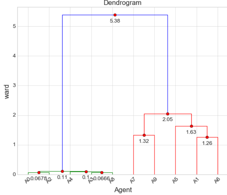
Figure 2.7: Dendrogram when ward's method is applied
