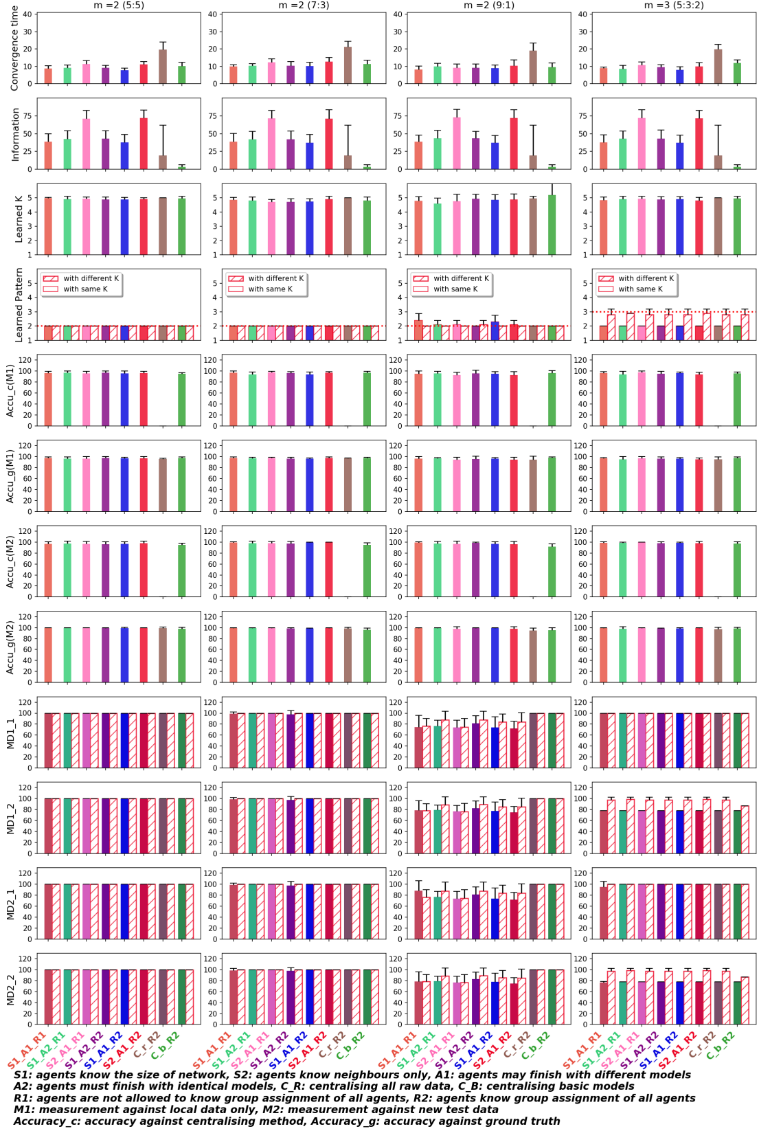
Figure 5.26: K-means on multiple patterns dense networks with uniformly well separated clusters
