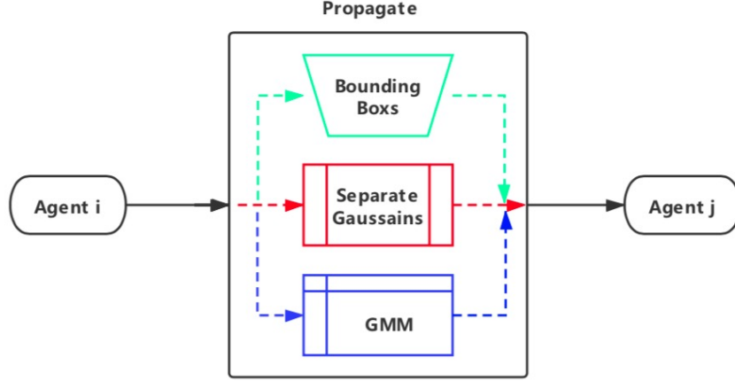
Figure 3.1: Information propagation
