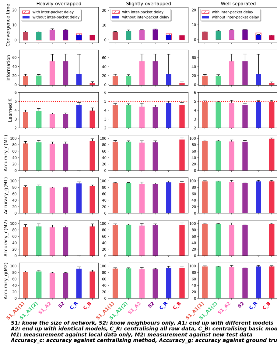
Figure 8.11: GMM on sparse network with fully symmetric Gaussians
