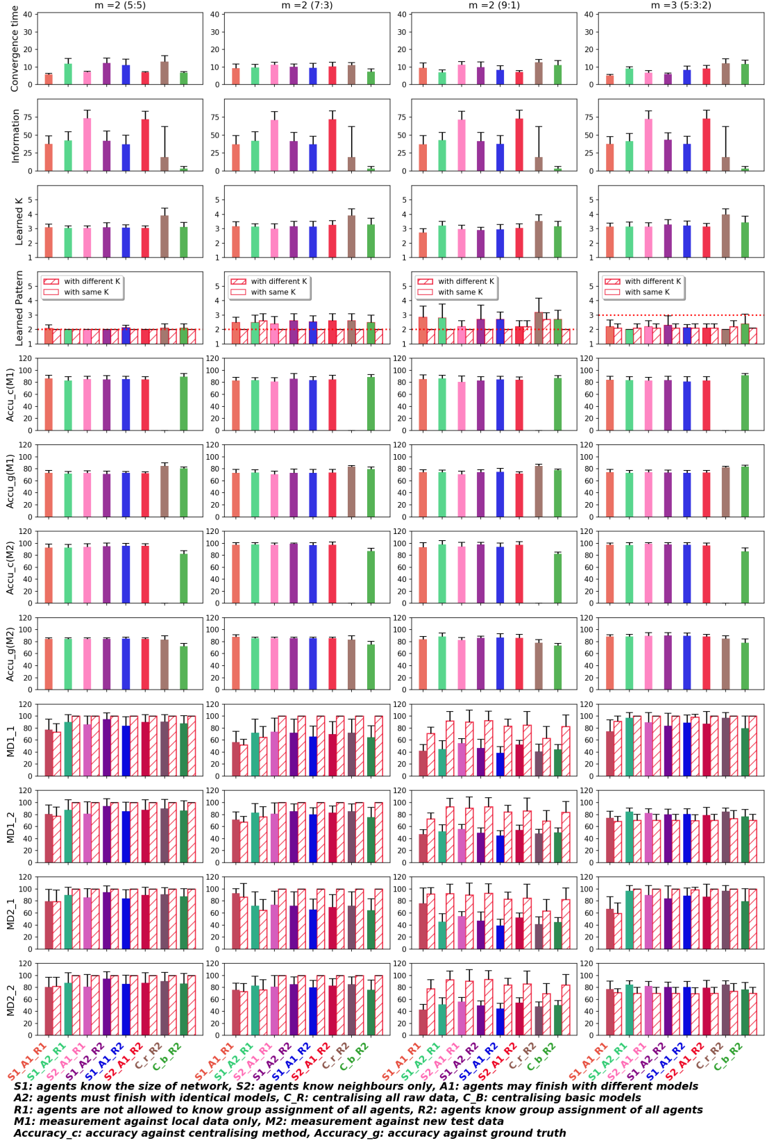
Figure 5.34: SG on dense network with multiple patterns and partially symmetric multi-dimensional Gaussians
