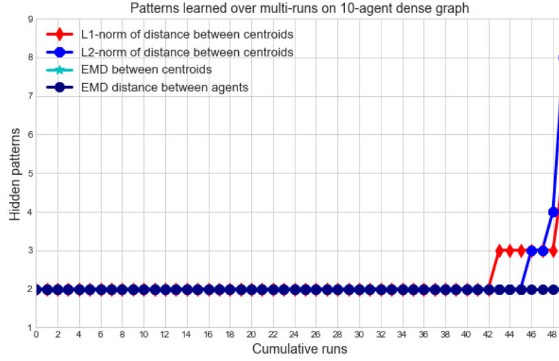
Figure 5.9: The number of estimated patterns with different similarity metrics
