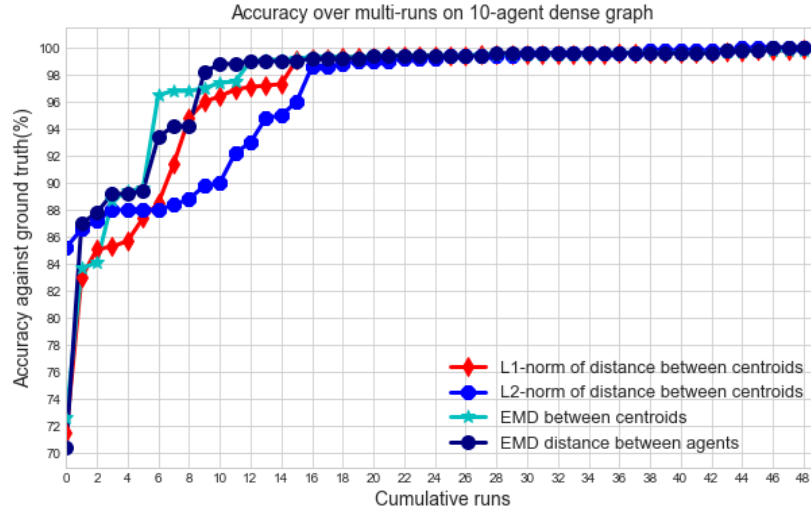
Figure 5.8: Accuracy on data points against ground truth with different similarity metrics
