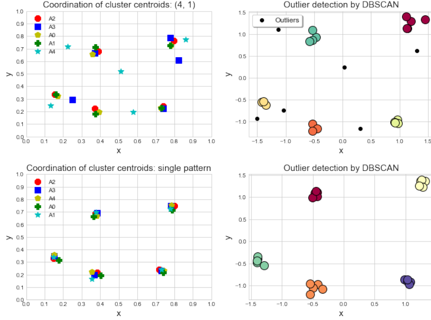
Figure 6.4: Application of DBSCAN to agents' clusters (1)
