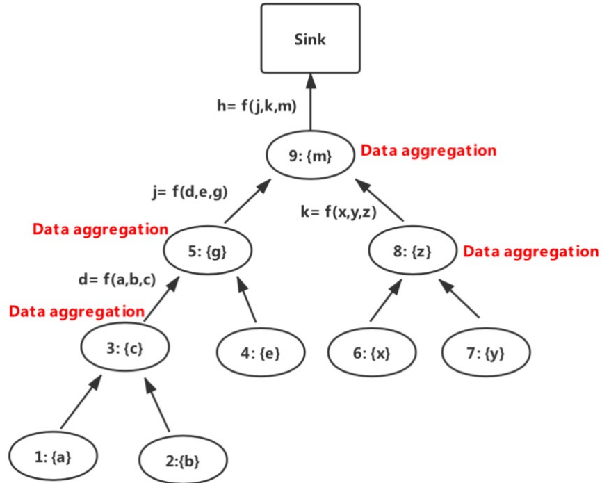
Figure 2.19: An example of tree-based aggregation process
