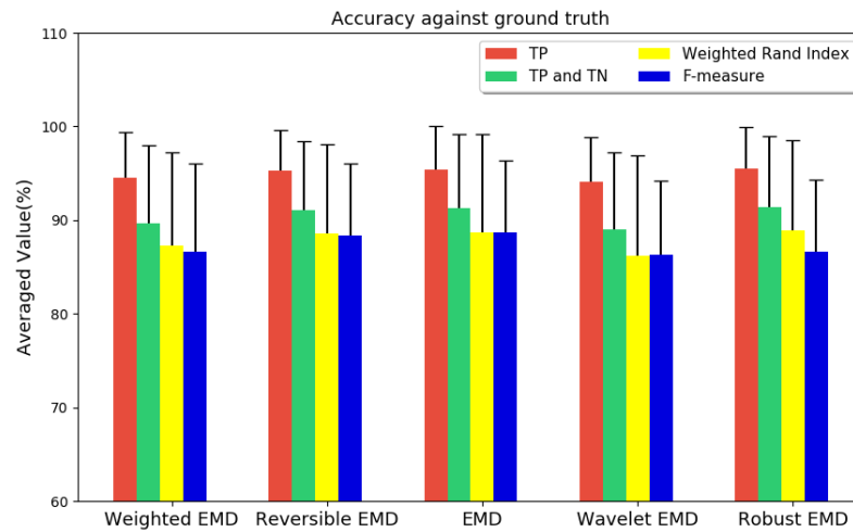
Figure 5.15: Accuracy against ground truth with asymmetric Gaussians
