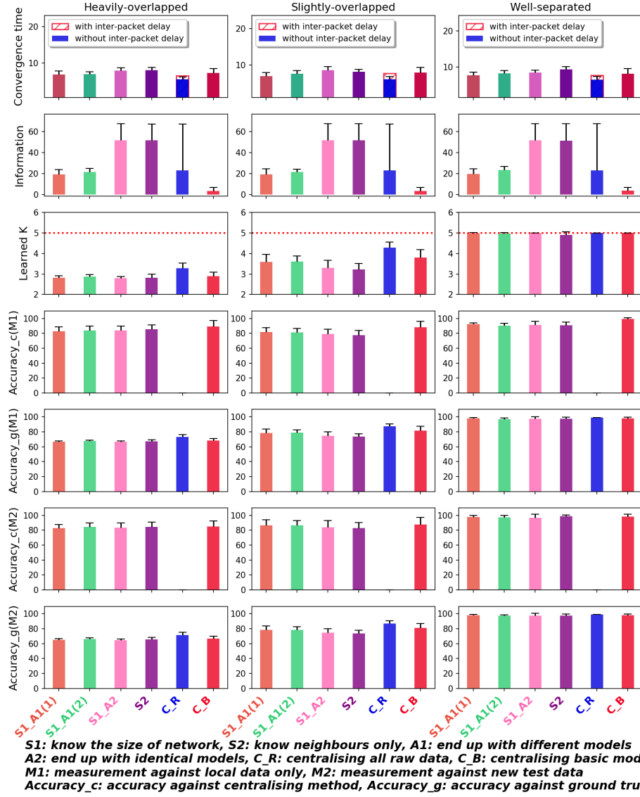
Figure 8.7: K-means on sparse network with uniform distributed dataset
