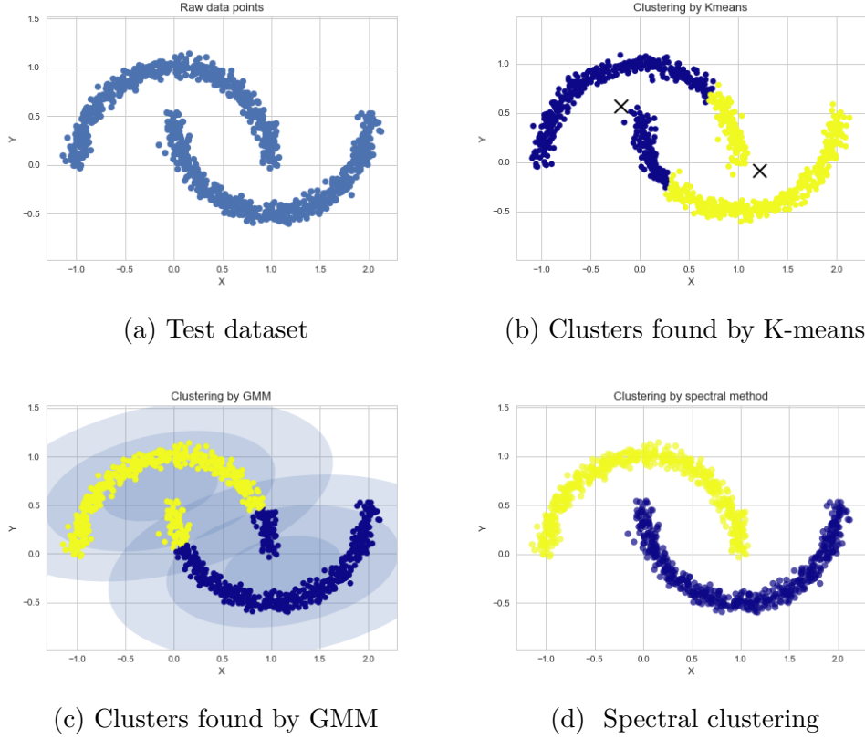
Figure 2.6: An example of K-means, GMM and Spectral clustering
