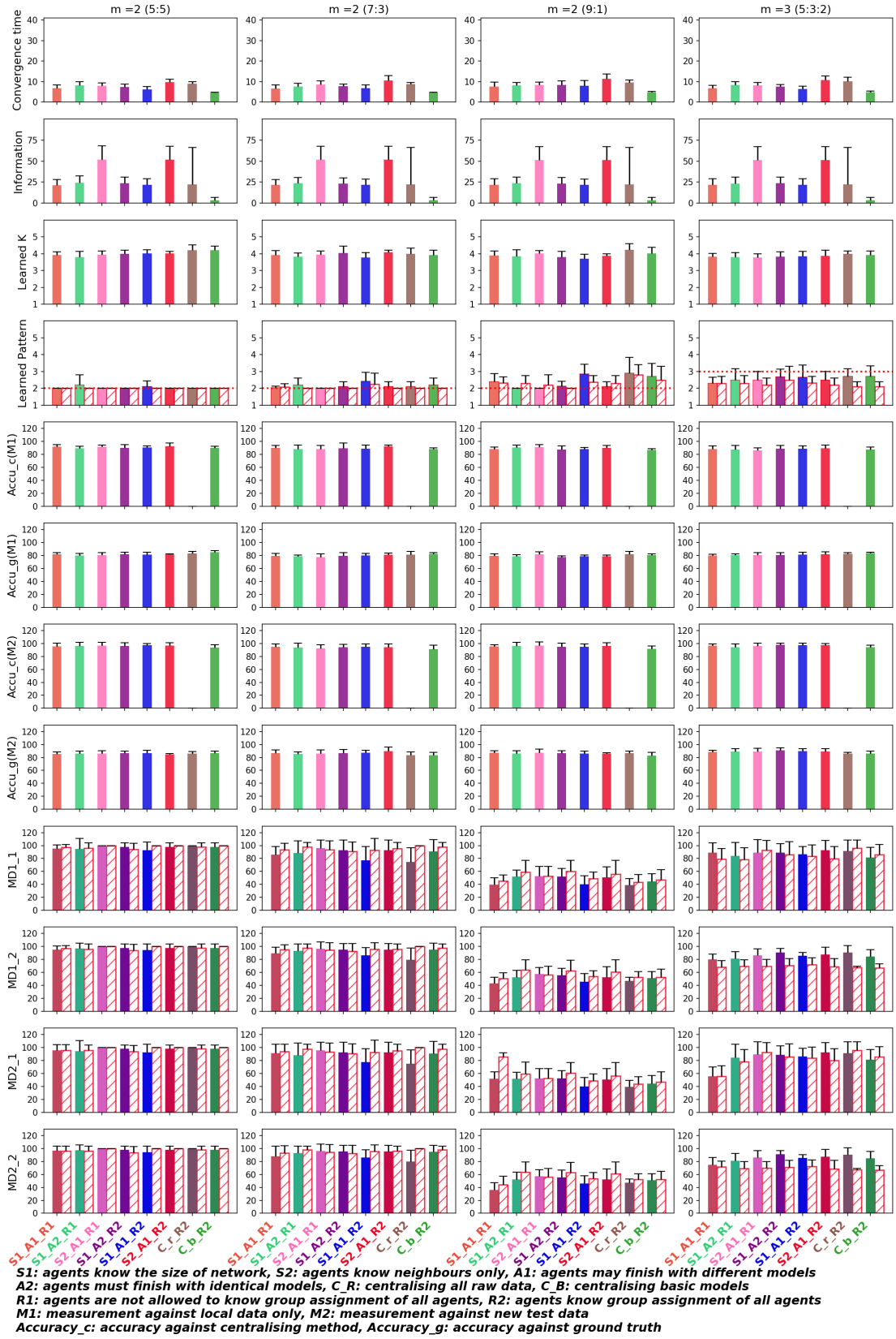
Figure 8.35: GMM on sparse network with multiple patterns and uniformly distributed dataset
