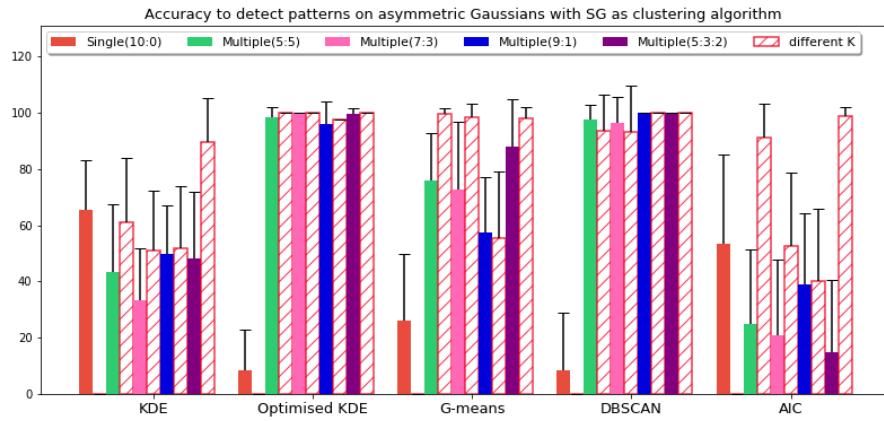
Figure 6.17: Accuracy achieved with asymmetric Gaussians when SG is used
