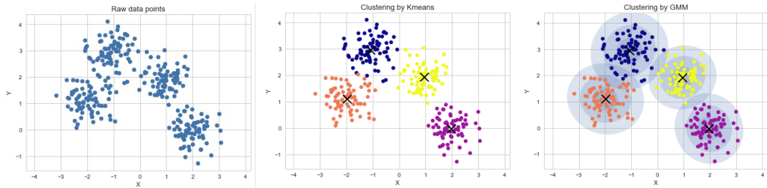
Figure 2.3: Comparison of K-means and GMM when underlying dataset is generated by symmetric Gaussians
