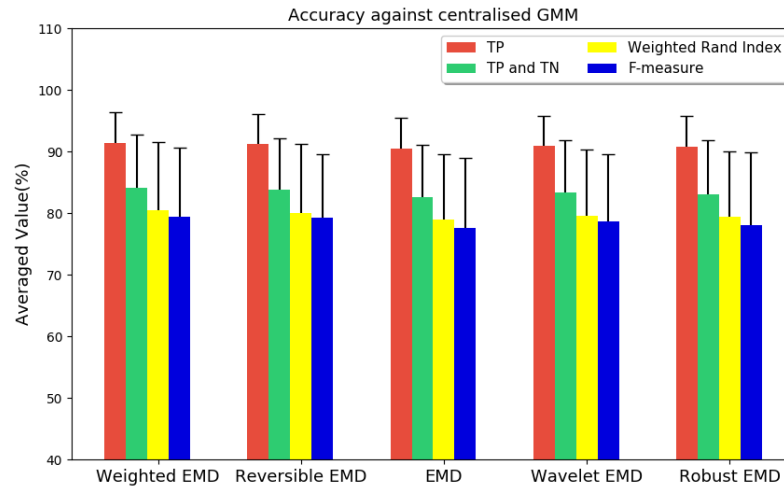
Figure 8.14: Accuracy against centralised GMM with fully symmetric Gaussians
