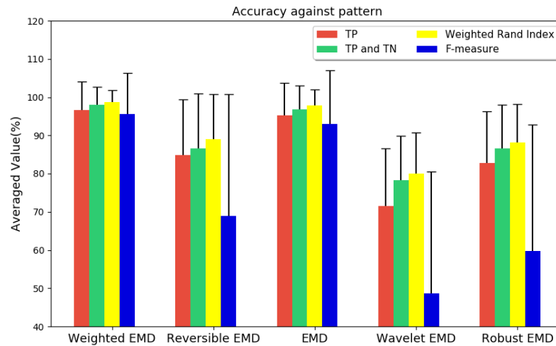
Figure 8.16: Accuracy against pattern with fully symmetric Gaussians
