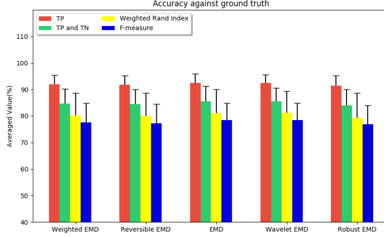
Figure 5.18: Accuracy against ground truth with uniformly distributed dataset
