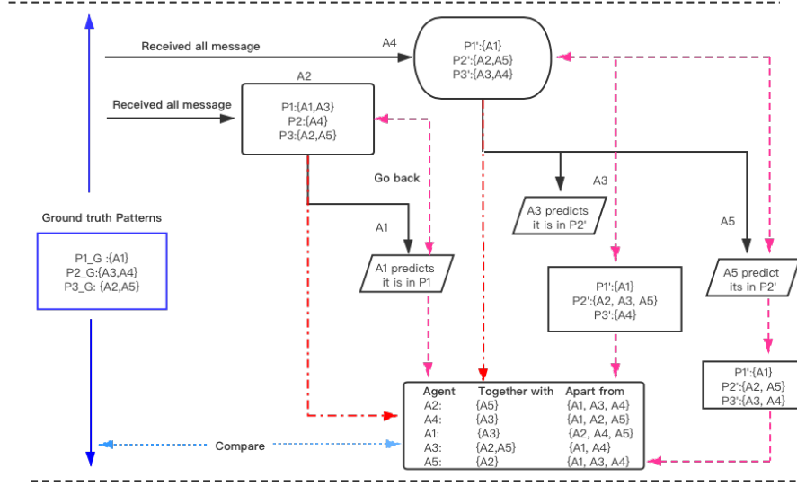
Figure 5.23: Asymmetric table built by agents' prediction
