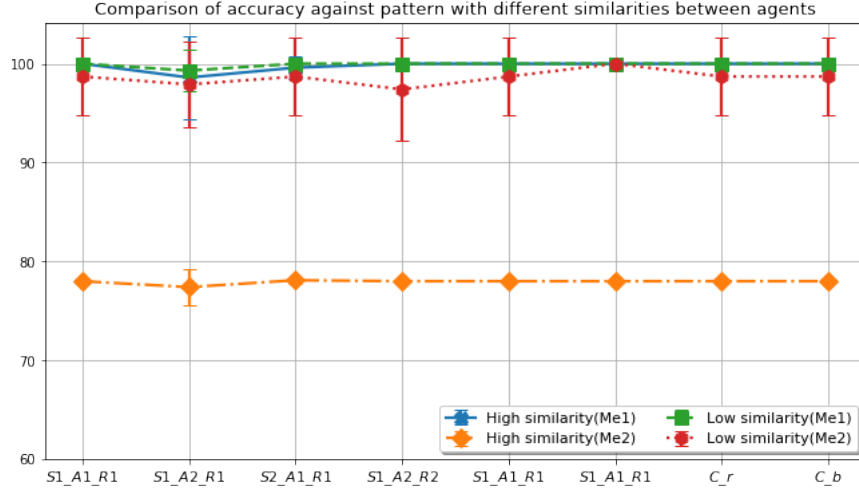
Figure 5.43: Accuracy against patterns with different similarities between agents
