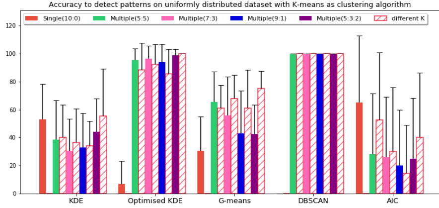
Figure 6.12: Accuracy achieved with uniformly distributed dataset when K-means is used
