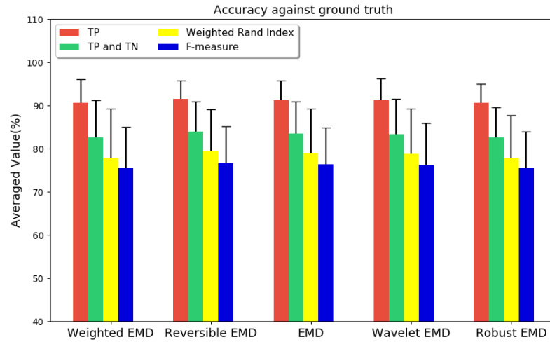
Figure 8.24: Accuracy against ground truth with uniformly distributed dataset
