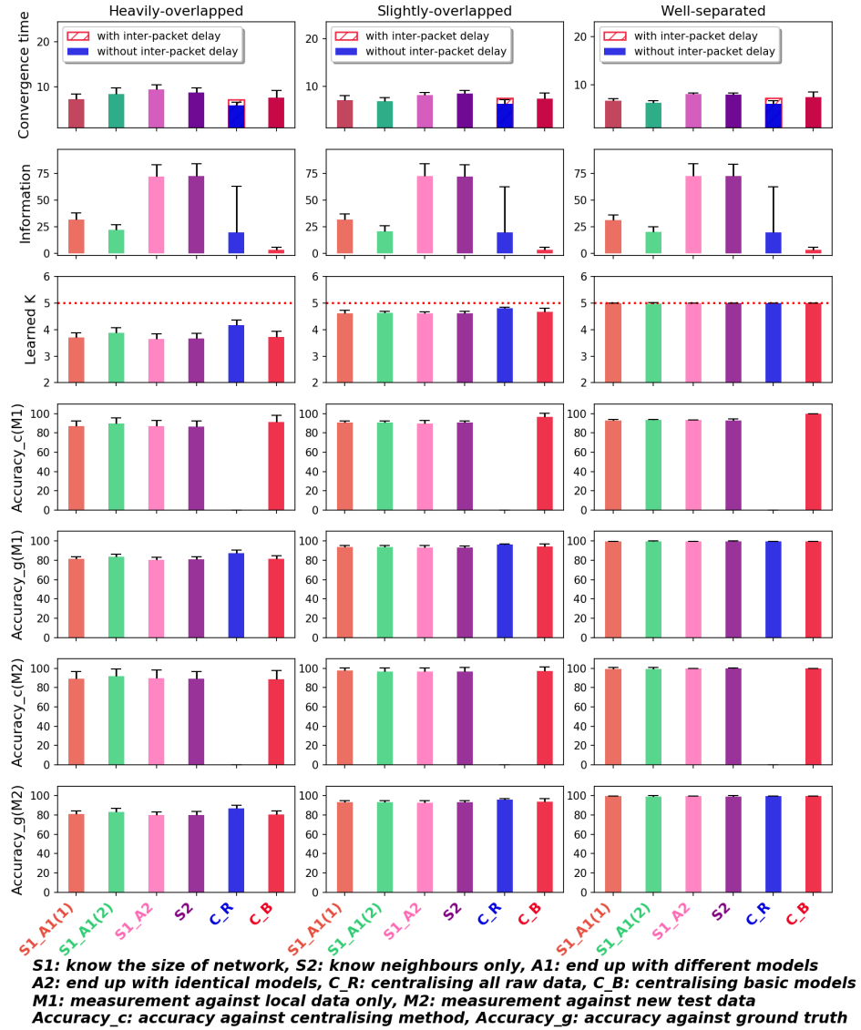
Figure 4.9: SG on dense network with symmetric multi-dimensional Gaussians
