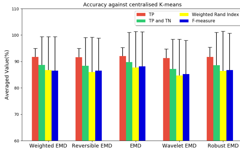
Figure 5.14: Accuracy against centralised k-means with asymmetric Gaussians
