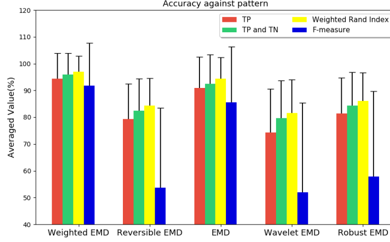
Figure 5.16: Accuracy against pattern with asymmetric Gaussians
