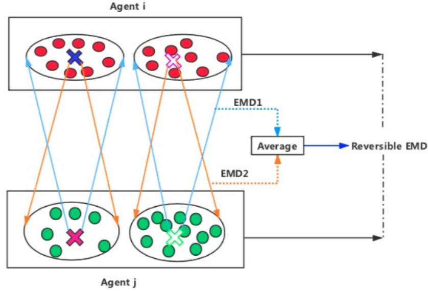
Figure 5.10: Reversible EMD between agents
