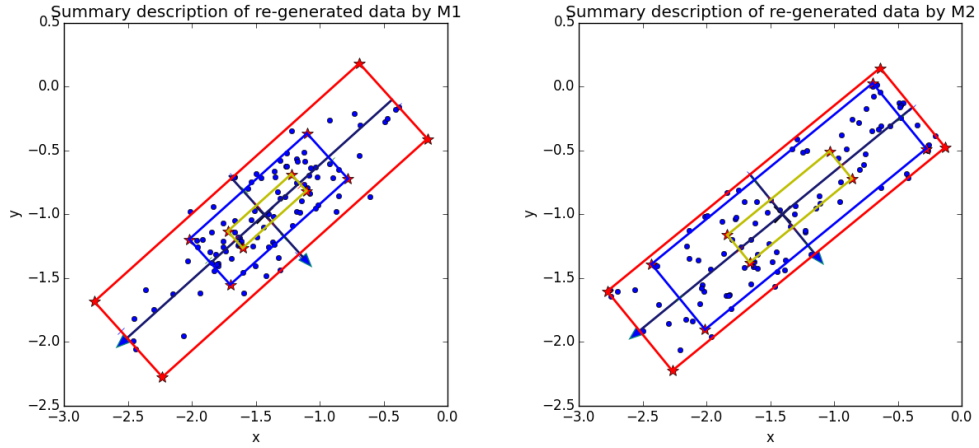
(a) re-generated data by M1 (Normal)] (b) re-generated data by M2 (Normal)
