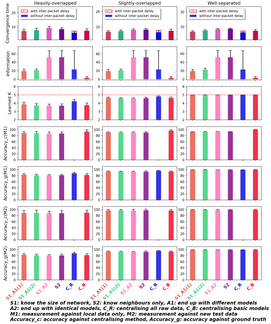
Figure 8.8: SG on sparse network with fully symmetric Gaussians
