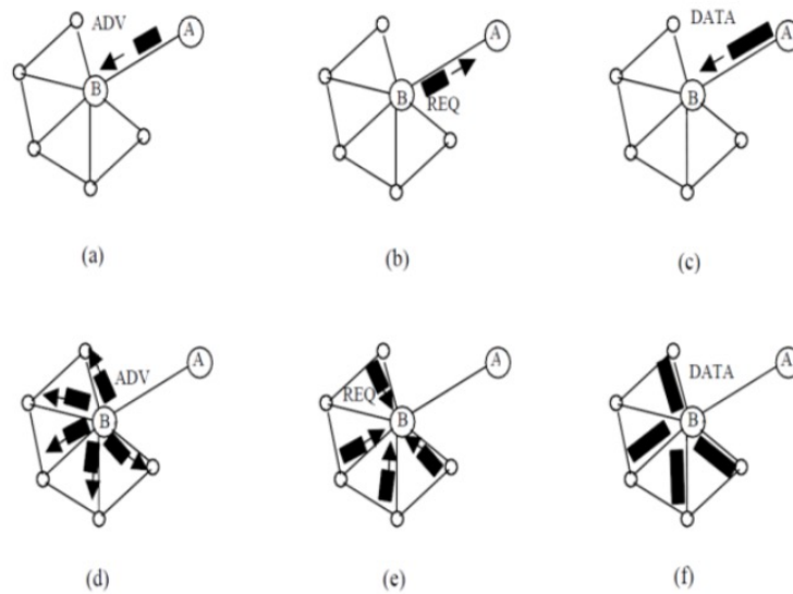
Figure 2.14: SPIN protocol [Patel and Parekh, 2014]
