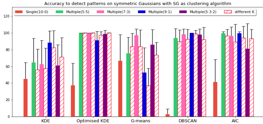
Figure 6.16: Accuracy achieved with symmetric Gaussians when SG is used
