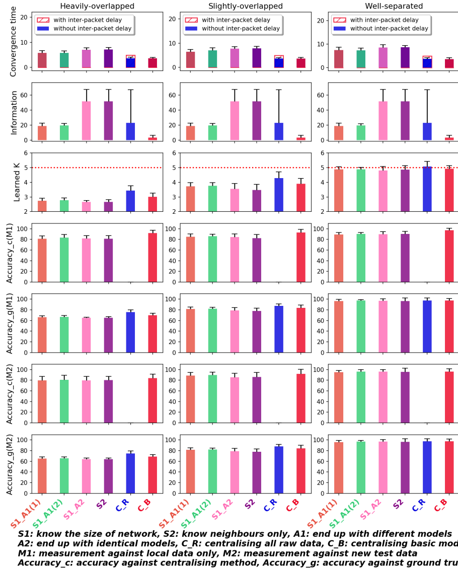
Figure 8.13: GMM on sparse network with uniform distributed dataset
