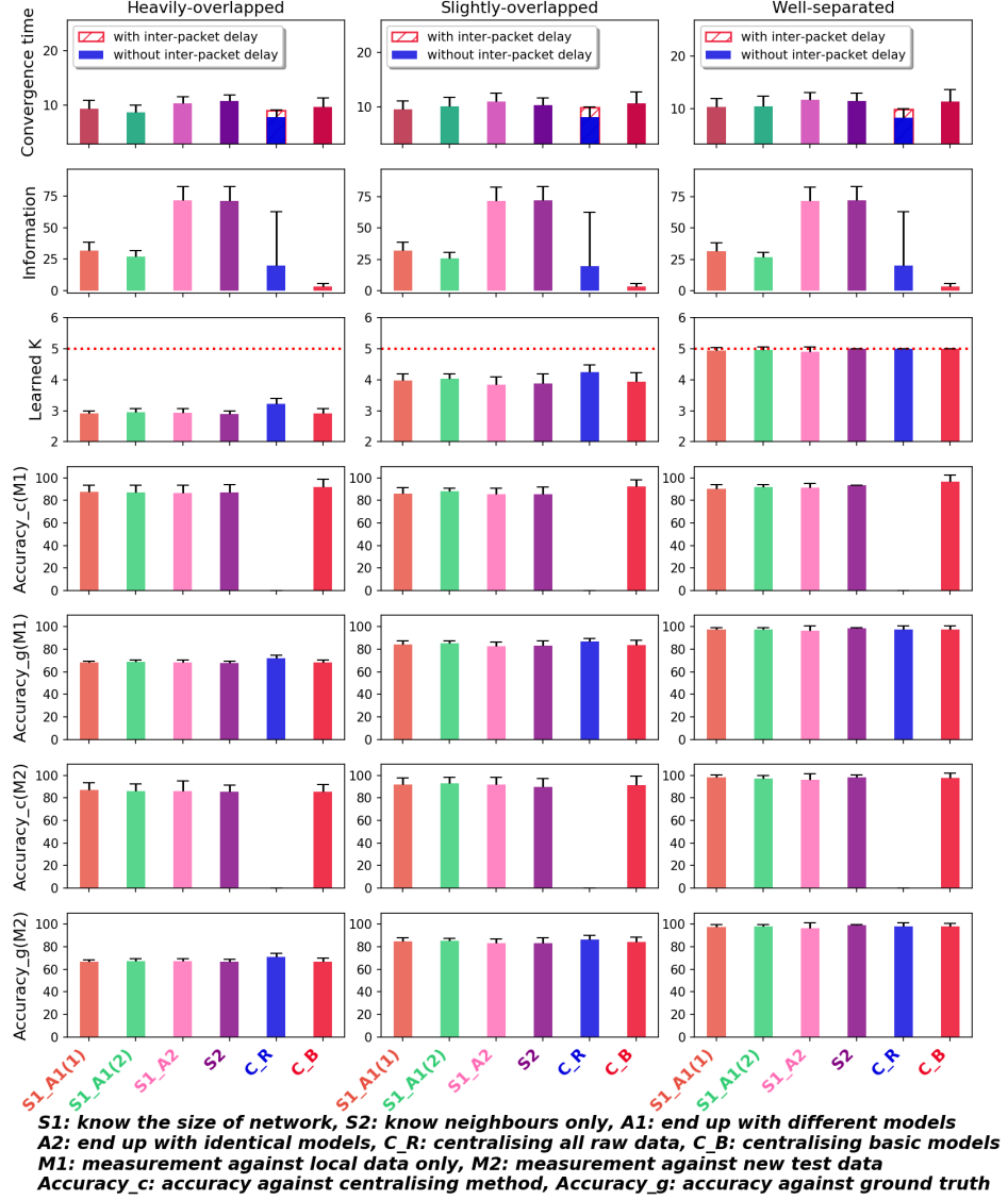
Figure 4.11: SG on dense network with uniform distributed dataset
