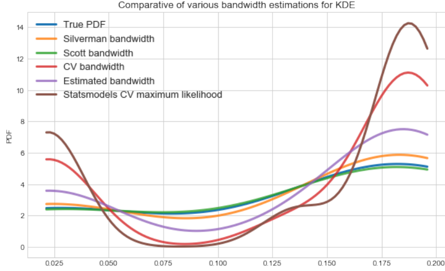
Figure 6.9: Comparative of various bandwidth estimation
