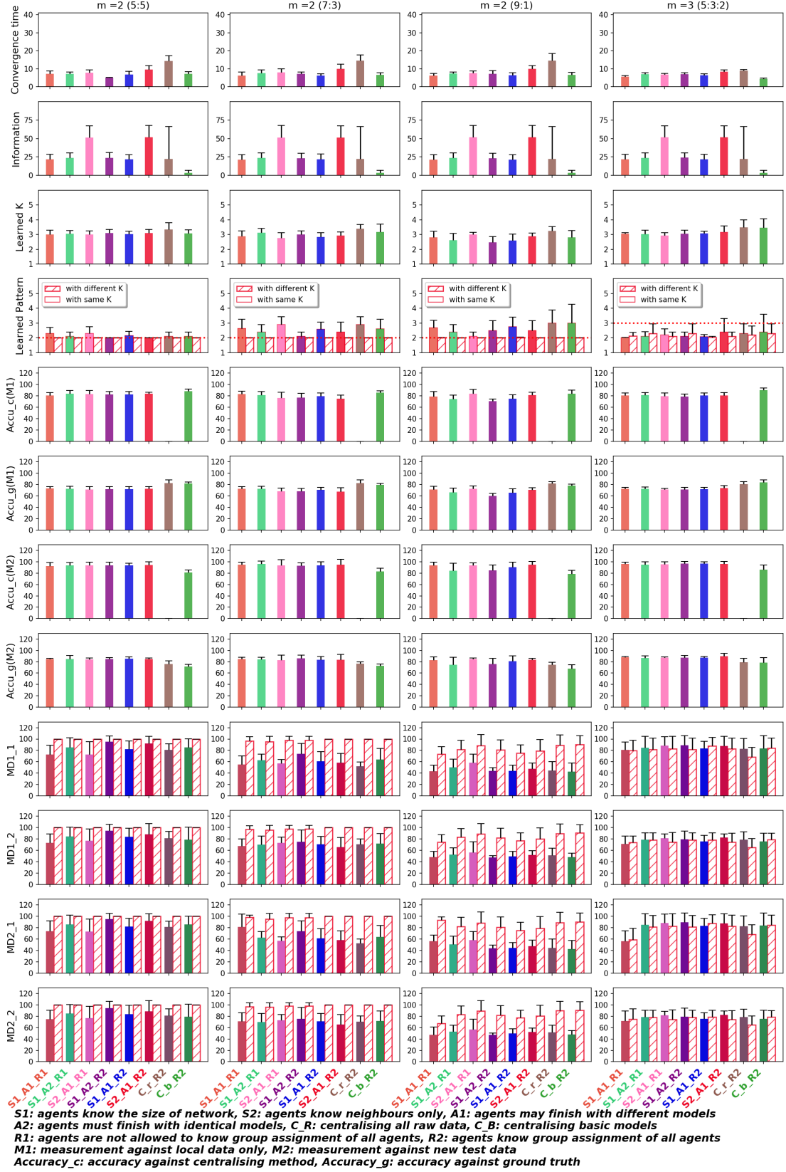
Figure 8.34: GMM on sparse network with multiple patterns and partially symmetric multi-dimensional Gaussians
