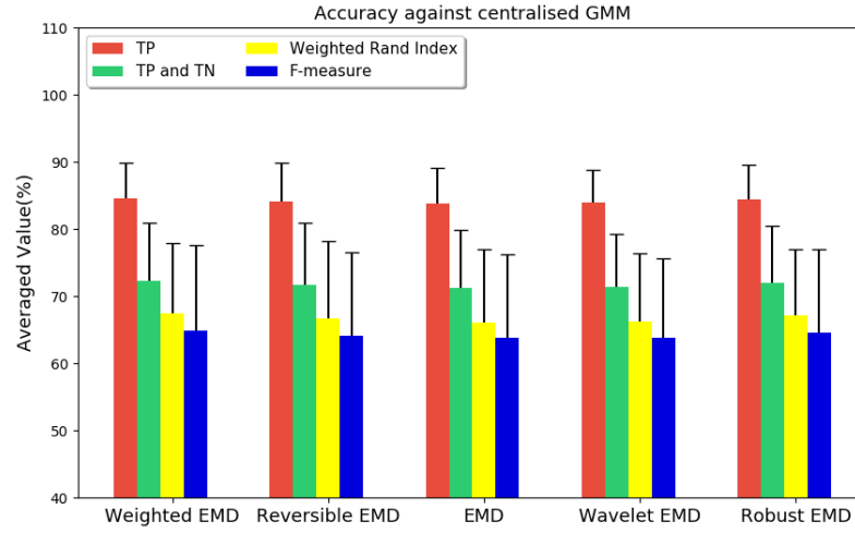
Figure 8.17: Accuracy against centralised GMM with datasets generated from uniform distributions
