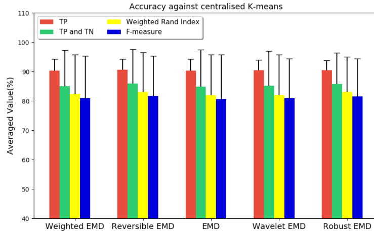
Figure 8.23: Accuracy against centralised SG with uniformly distributed dataset
