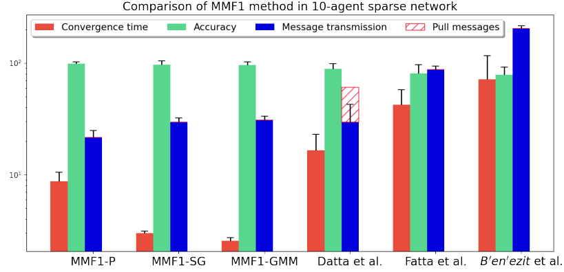
Figure 3.5: Comparison of different schemes under MMF1 method in a 10-agent sparse network, showing mean results for each measure over 50 runs.
