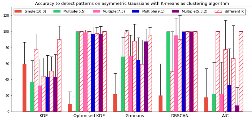
Figure 6.11: Accuracy achieved with asymmetric Gaussians when K-means is used
