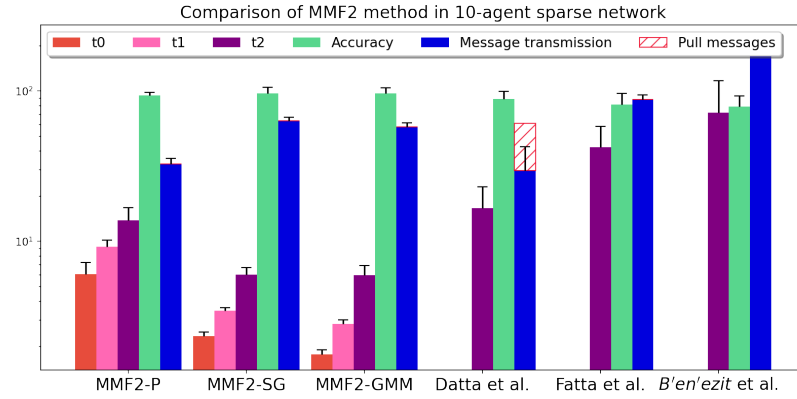
Figure 3.7: Comparison of different schemes under MMF2 method in a 10-agent sparse network
