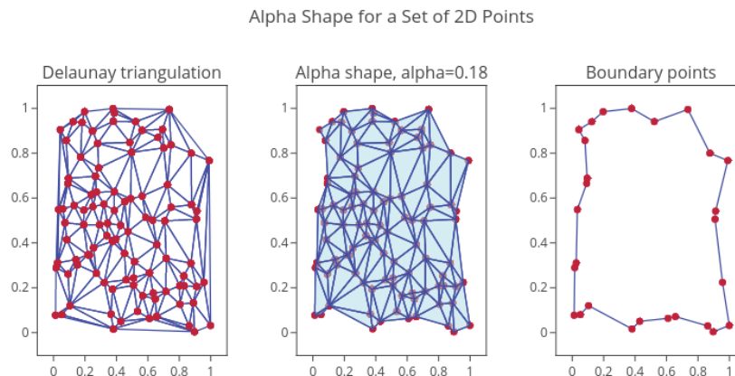
Figure 2.16: An example of obtaining boundary points of a cluster
