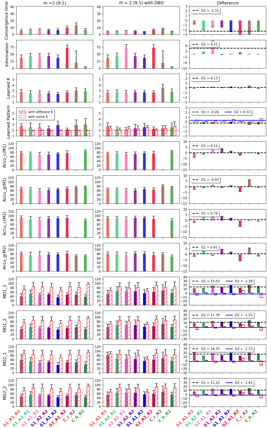
Figure 5.38: Performance achieved by DBD with GMM as clustering algorithm and asymmetric Gaussians as underlying dataset
