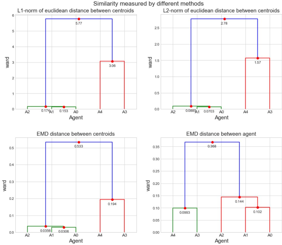
Figure 5.3: Hierarchical clustering by different methods
