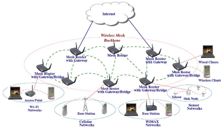
Figure 1.1: Architecture of wireless mesh network [Akyildiz et al., 2005]
