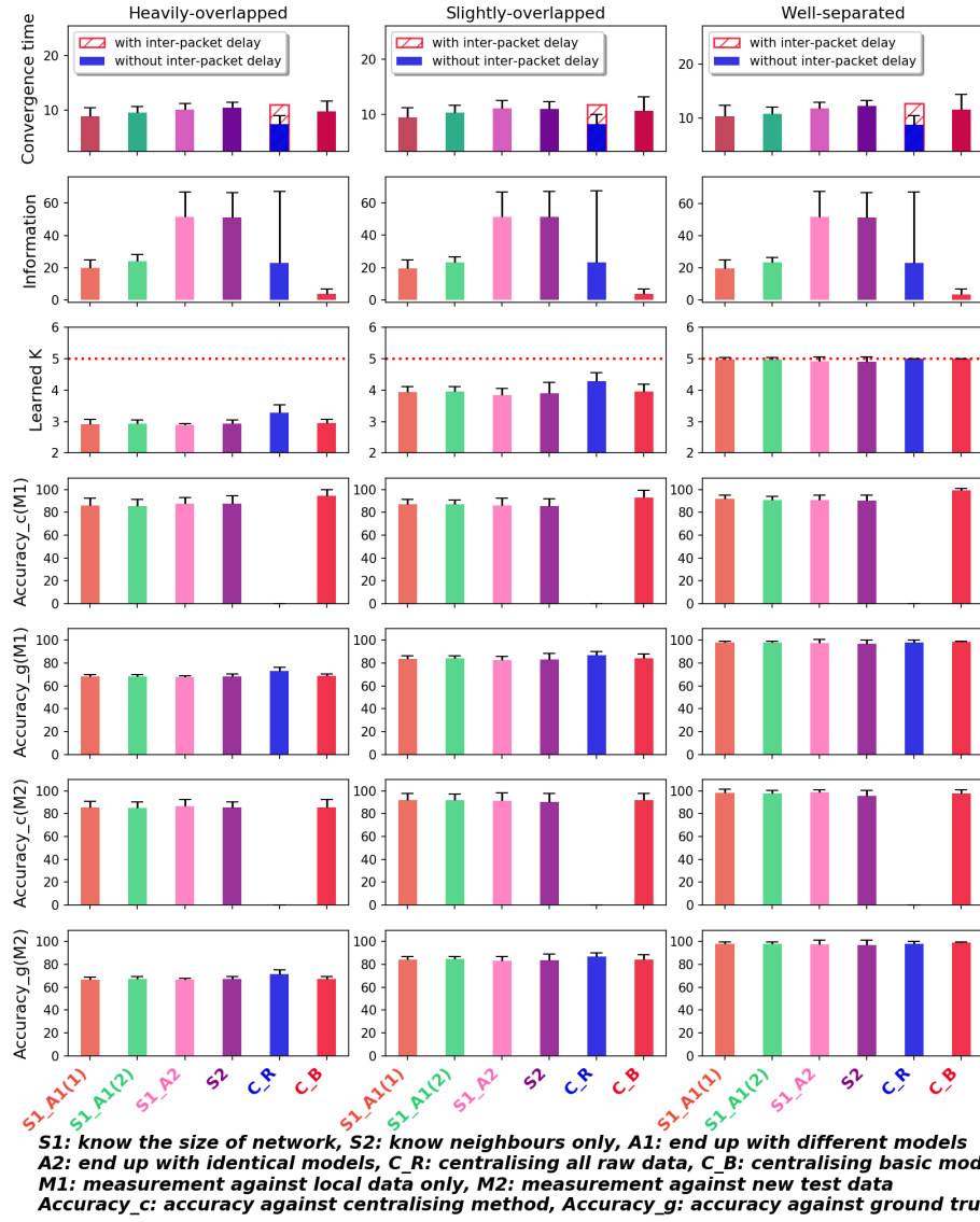
Figure 8.10: SG on sparse network with uniform distributed dataset
