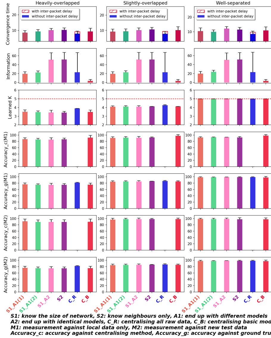
Figure 8.9: SG on sparse network with partially symmetric Gaussians
