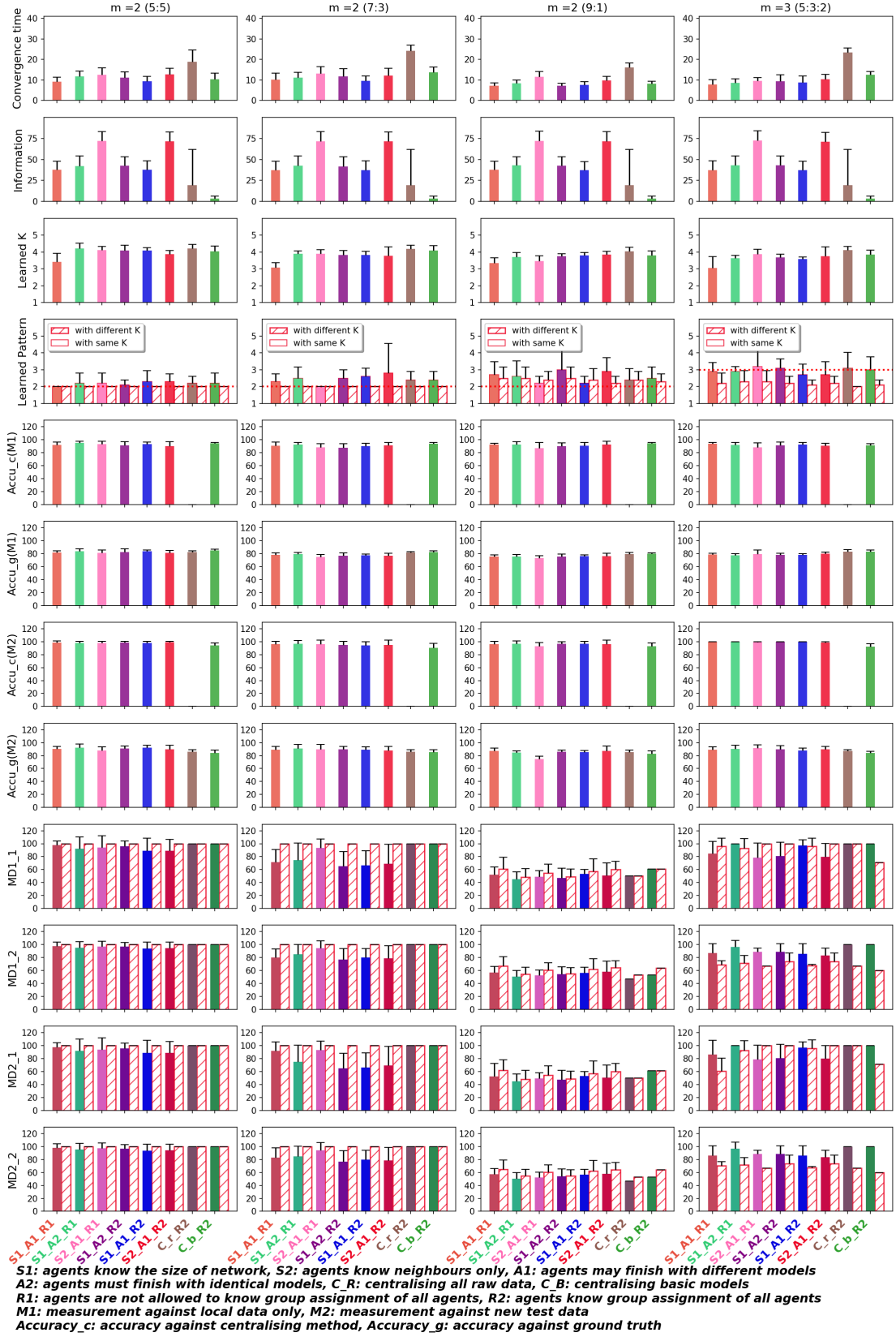
Figure 5.29: K-means on dense network with multiple patterns and uniformly distributed dataset
