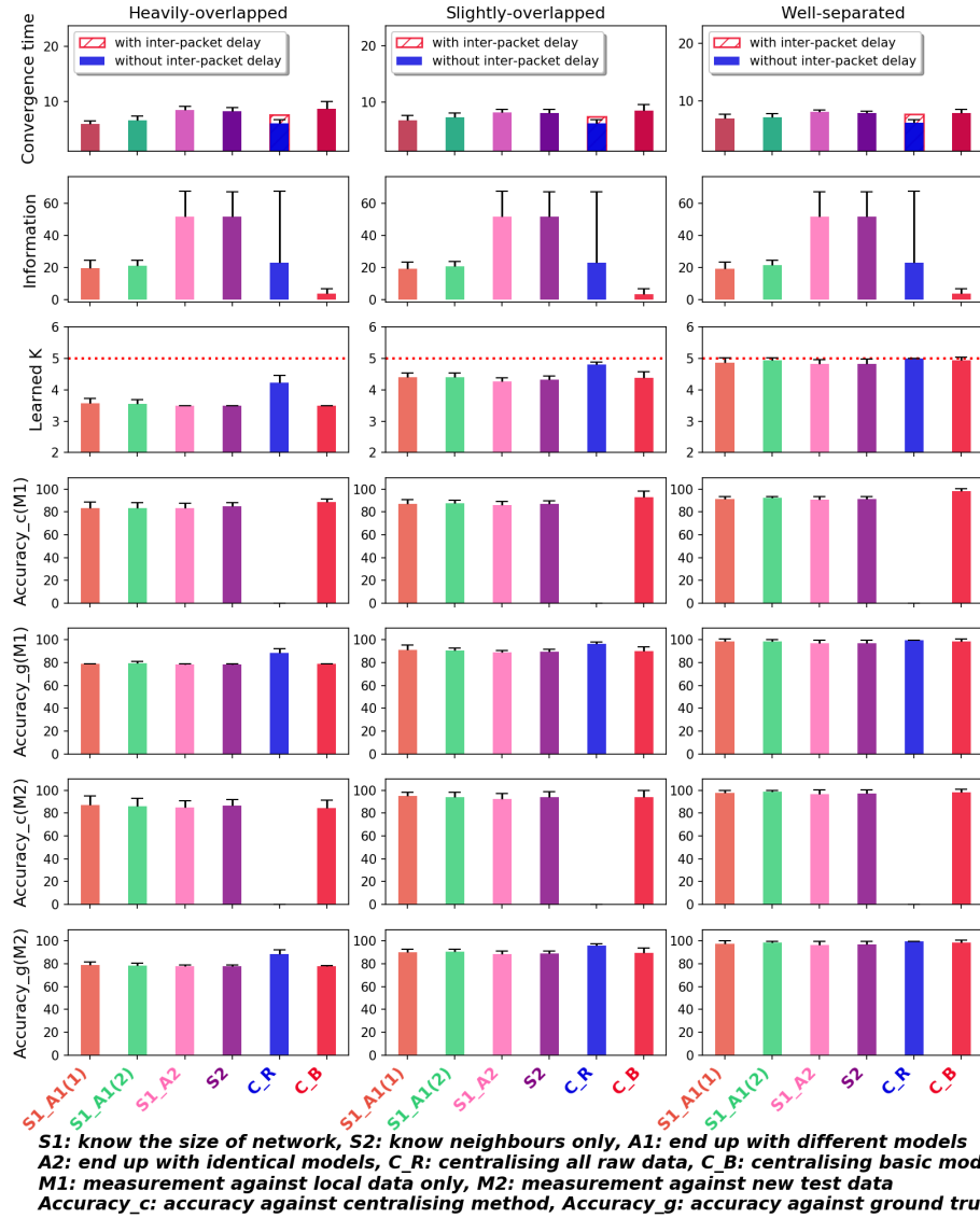
Figure 8.5: K-means with fully symmetric Gaussians on sparse network
