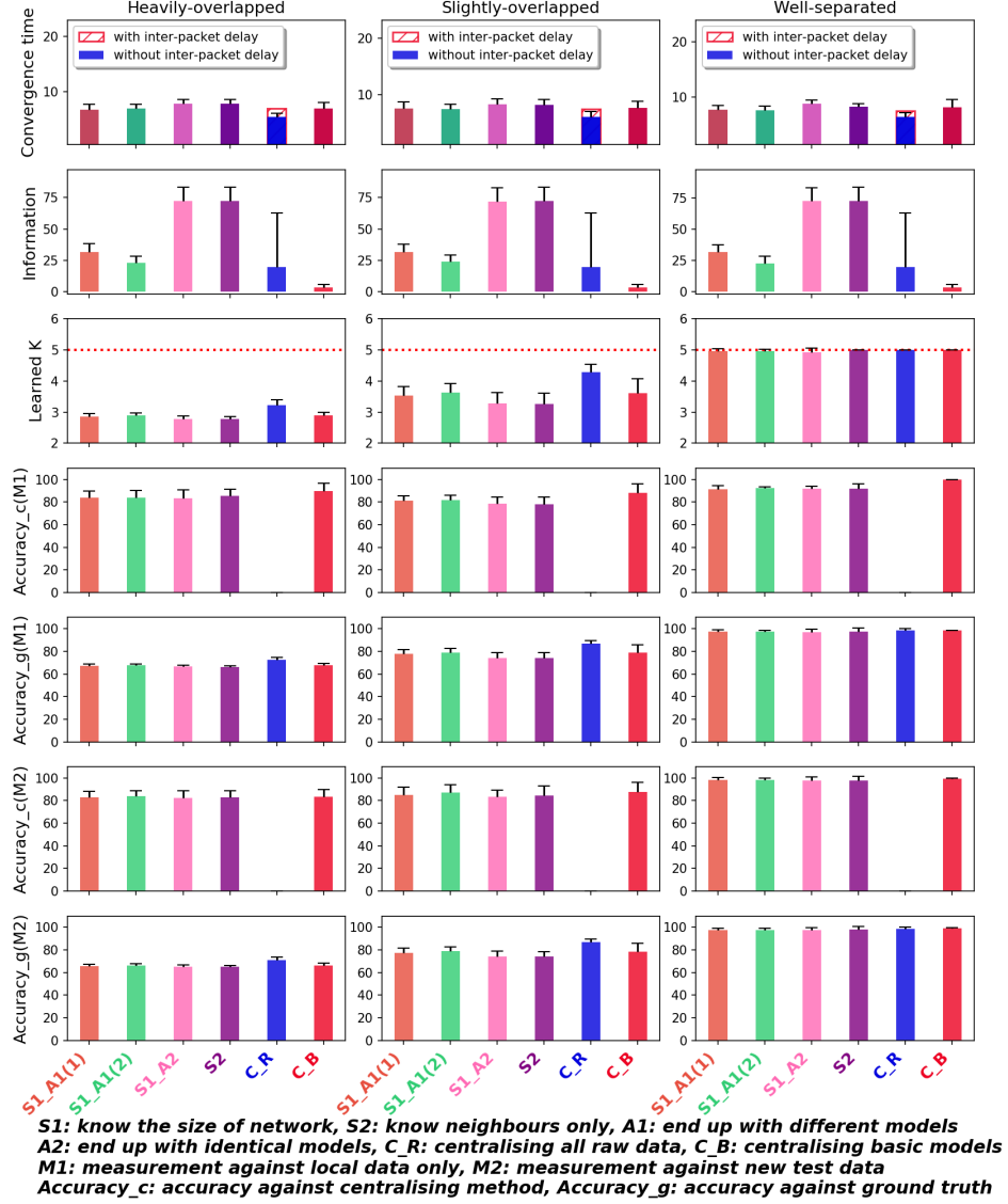
Figure 4.8: K-means on dense network with uniform distributed datasets
