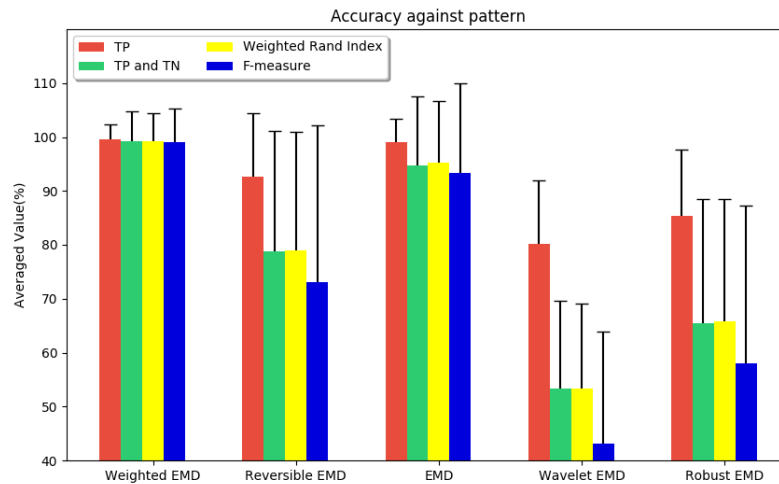
Figure 5.13: Accuracy against pattern with symmetric Gaussians
