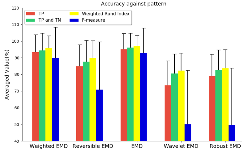
Figure 8.19: Accuracy against pattern with uniformly distributed dataset
