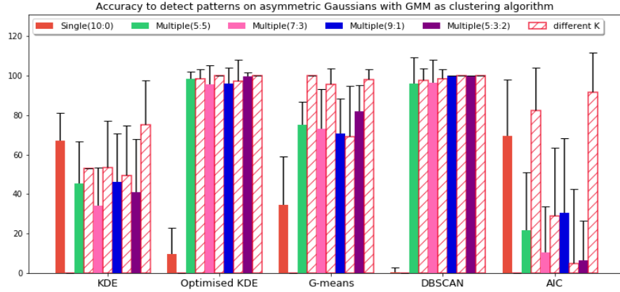
Figure 6.14: Accuracy achieved with asymmetric Gaussians when GMM is used
