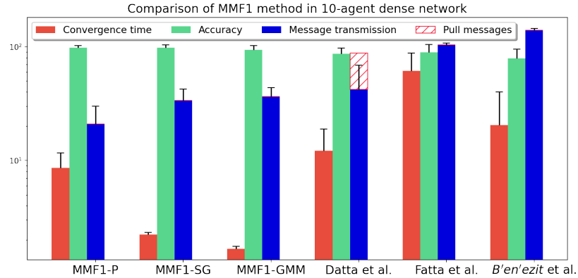
Figure 3.4: Comparison of MMF1 method in 10-agent dense network, showing mean results for each measure over 50 runs.
