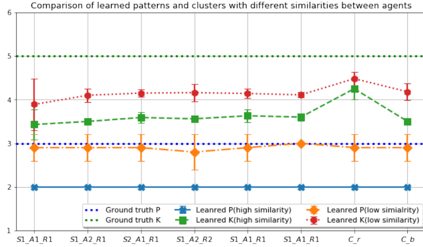
Figure 5.44: Accuracy against patterns with different similarities between agents
