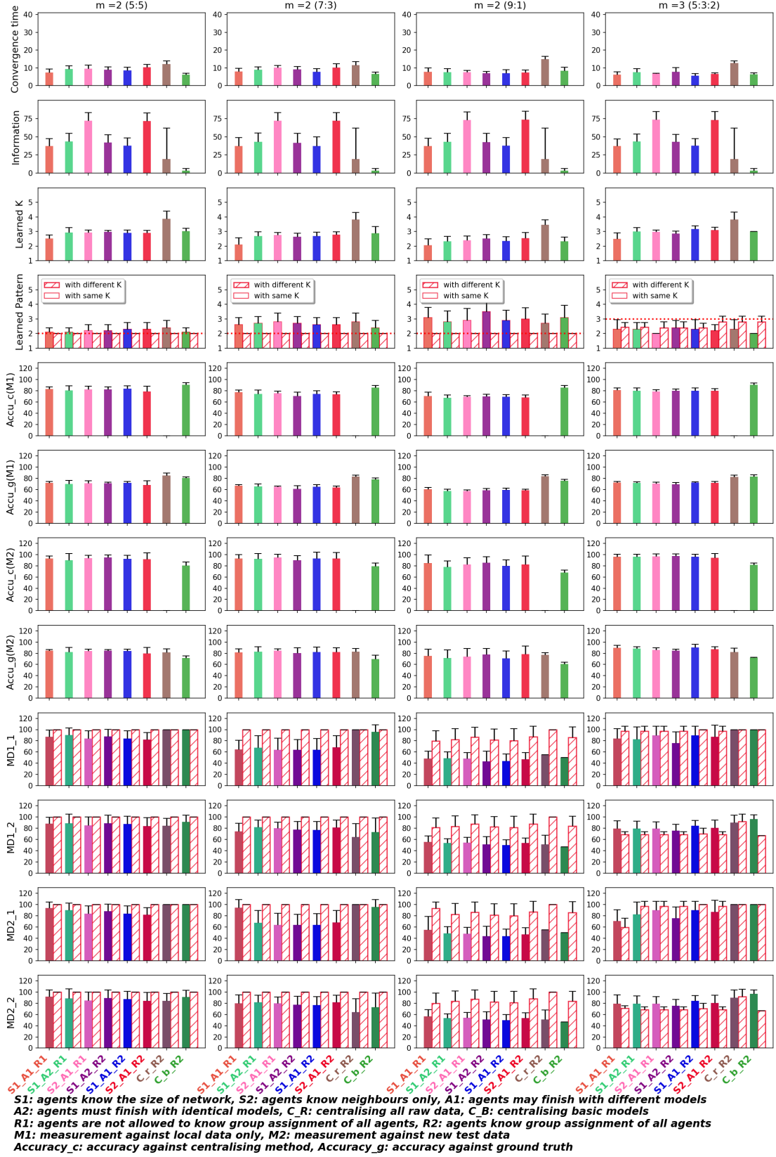
Figure 5.28: K-means on dense network with multiple patterns and asymmetric multi-dimensional Gaussians
