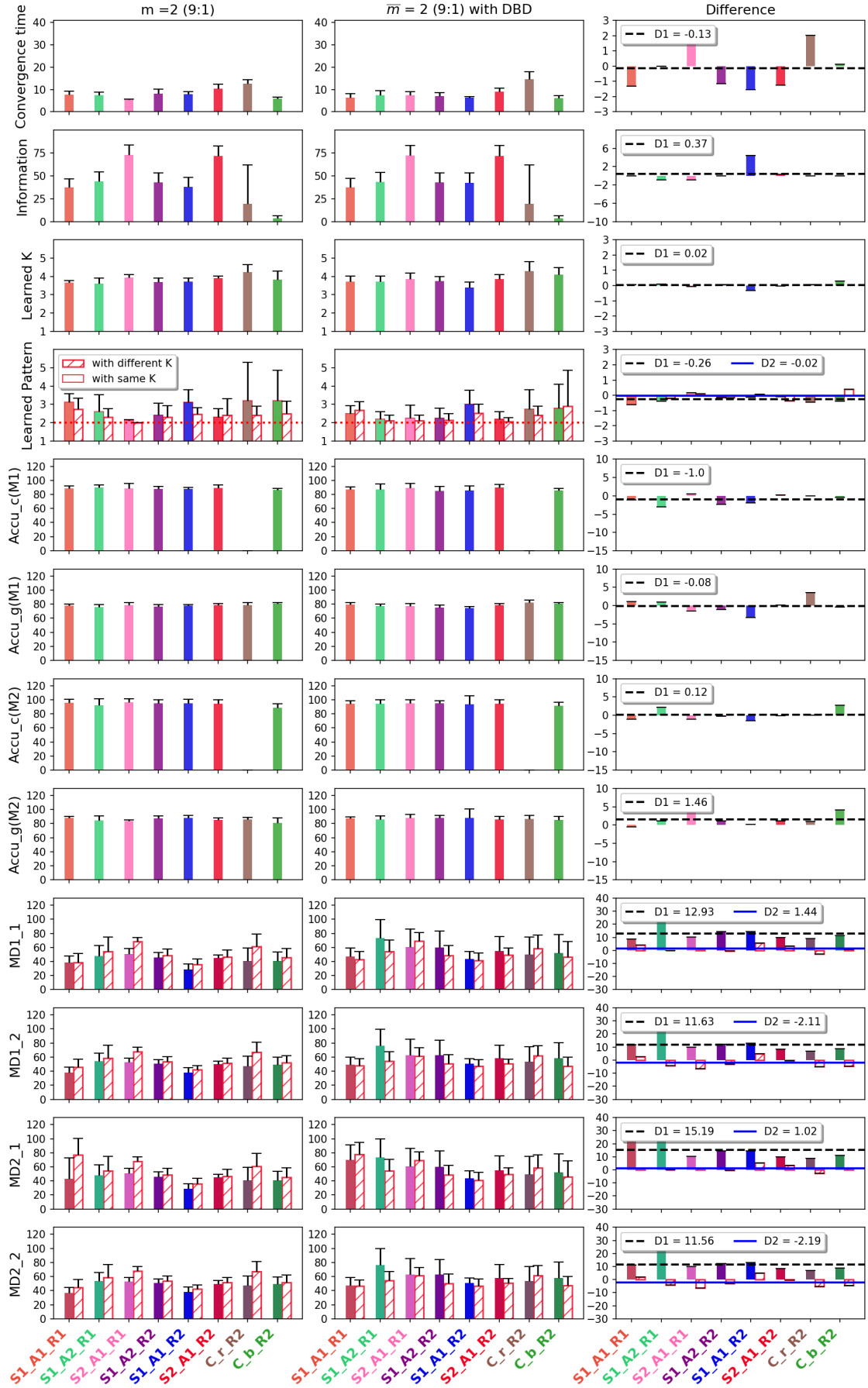
Figure 5.39: Performance achieved by DBD with GMM as clustering algorithm and uniformly distributed datasets as underlying dataset
