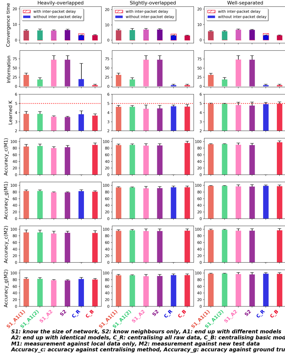
Figure 4.12: GMM on dense network with symmetric multi-dimensional Gaussians
