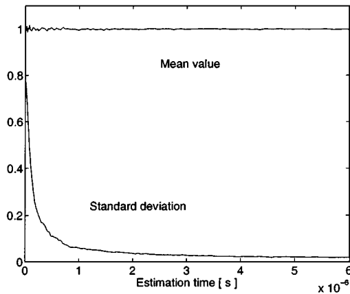
Fig. 4. Mean and standard deviation of the estimation of \int_0^T g_1^2(t) dt versus the estimation time.
