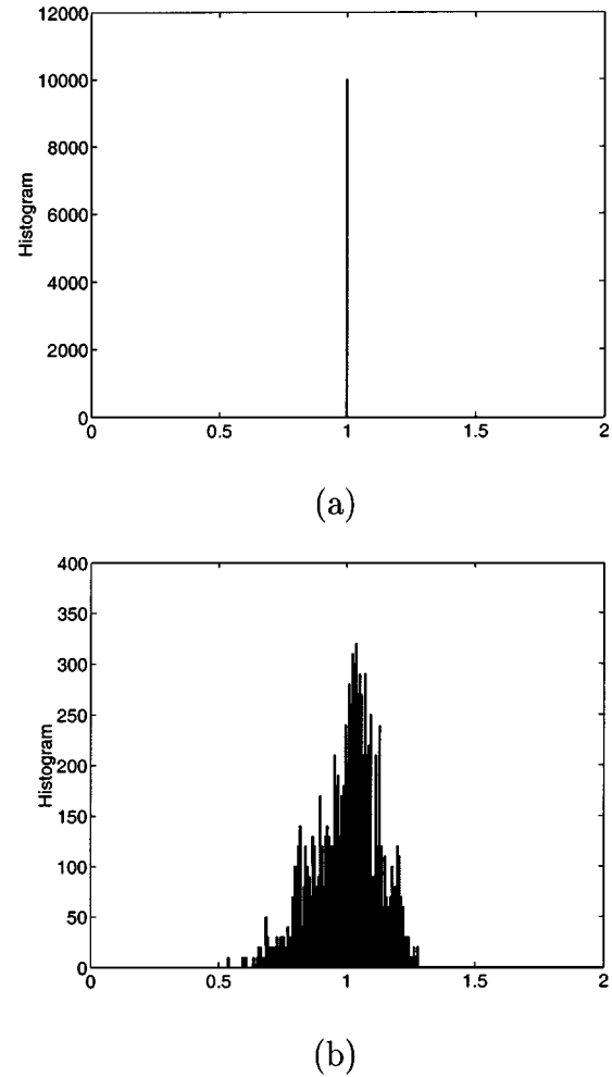
Fig. 3. Samples of \int_0^T g_j^2(t) dt for (a) periodic and (b) chaotic basis functions g_j(t) .
