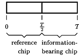
Fig. 6. A DCSK basis function g_j(t) consists of two segments called the reference and information-bearing chips.
