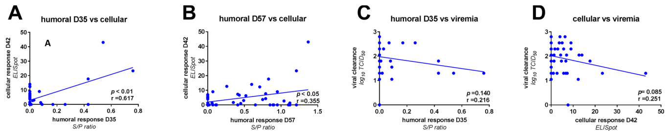
Fig. 8. Association between PRRSV specific humoral and cellular immune response and viral clearance. Scatter plots of humoral immune response on D35 (one week after booster vaccination) and D57 (one week after challenge) versus cellular immune response on D42 (two weeks after booster vaccination) (A and B); Scatter plots of viral clearance on D63 (15 days after challenge) versus cellular and humoral immune response (C and D). All animals independent of vaccination and administration route, were included in this association.
