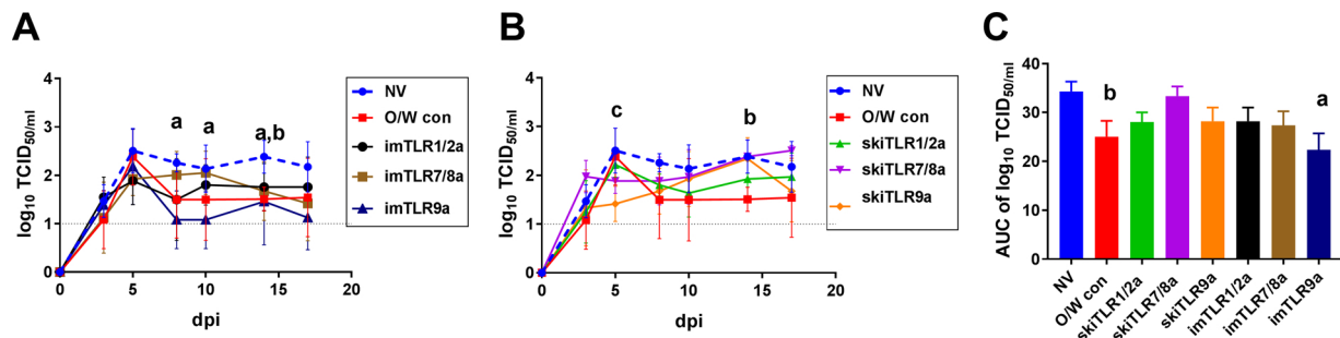
Fig. 6. Clearance of PRRSV in serum after challenge. Virus titers in serum (log 10 TCID 50 /ml) determined by virus titration. (A) serum virus titers of i.m. vaccinated Toll-like receptor (imTLRa) groups compared to non-vaccinated (NV) group and oil-in-water control (O/W con) group (B); serum virus titers of skin vaccinated skiTLRa groups compared to non-NV group and O/W con group. Each data point represents the average of 6 animals \pm S.D. The dotted line marks the detection limit for virus titration; (C) Area under the curve (AUC) calculated for the whole group with the S.D. “a” indicates a significant difference ( p < 0.05 ) between imTLR9a group and NV group; “b” between O/W con group and NV group and “c” between the skiTLR9a group and the NV group.
