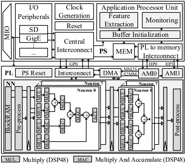
Fig. 5. Neural network inference acceleration on Zynq-7000 SoC architecture.
