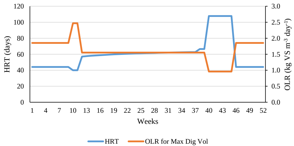
Figure B-12: Scenario PB-S HRT and OLR.
