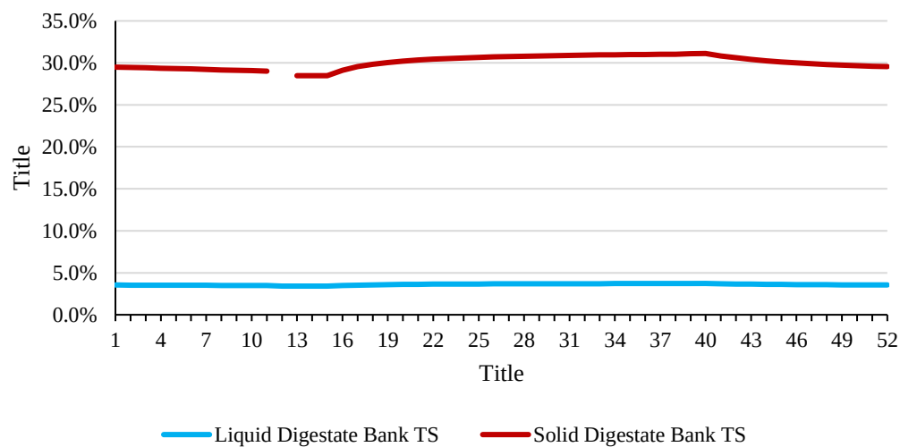
Figure B-3: Scenario ZG-W digestate bank solids content.
