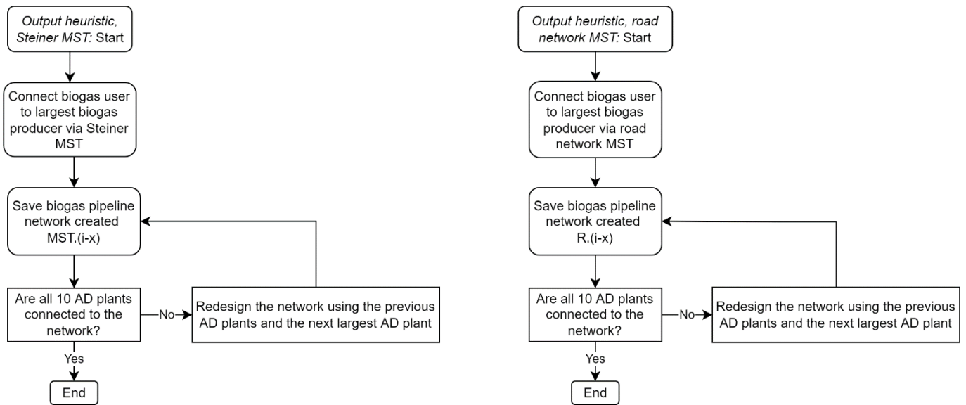
Figure 6-3: Flowchart methodology for output heuristic.
