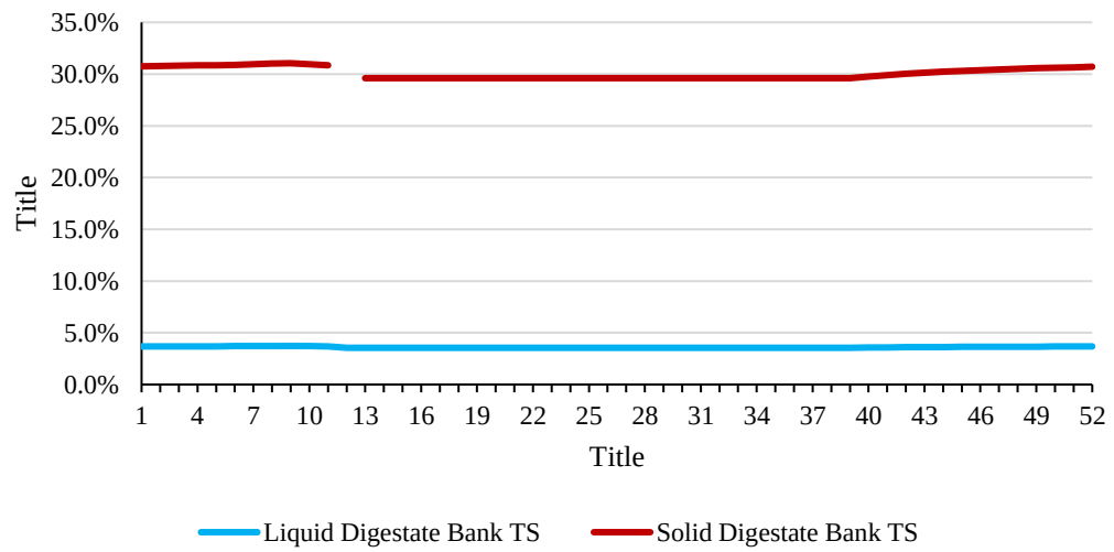
Figure B-5: Scenario ZG-S digestate bank solids content.
