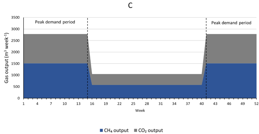
Figure 4-3: Scenario ZG-W, A) Weekly digester inputs, B) Digester solids content, C) Weekly digester gas output, D) Cumulative digestate bank.
