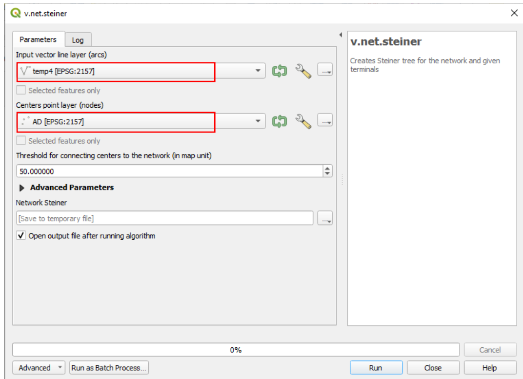
Figure D-10: v.net.steiner dialog window.
