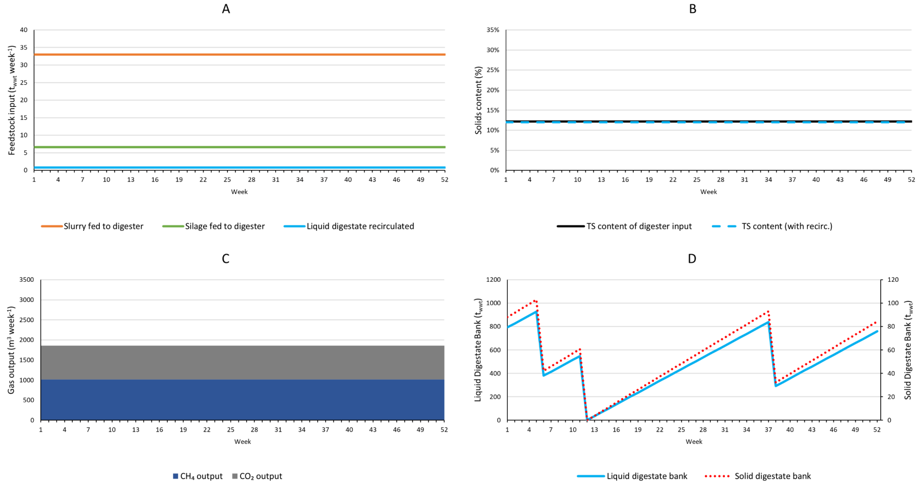
Figure 4-1: Scenario ZG-C, A) Weekly digester inputs, B) Digester solids content, C) Weekly digester gas output, D) Cumulative digestate bank.
