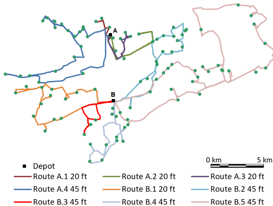
Figure 5-5: Routing requirement for scenario 6 (multi capacity, multi depot, on-site upgrading).
