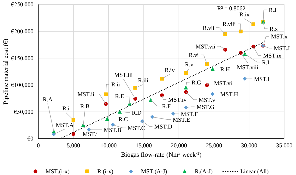
Figure 6-7: Scenario pipeline material cost vs. biogas flow-rate.
