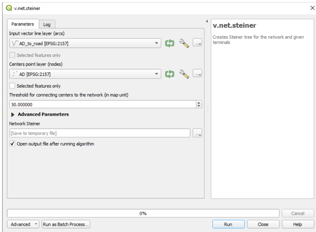
Figure D-19: v.net.steiner dialog window.
