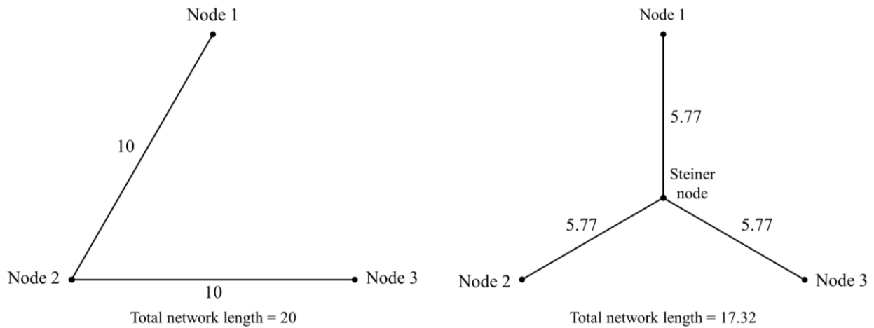
Figure 6-1: Comparison of standard MST (left) and Steiner MST (right).
