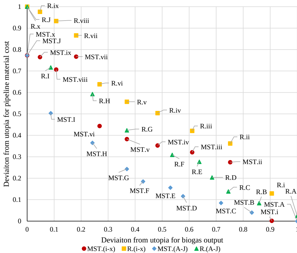
Figure 6-9: MCDA chart of deviation from utopia, for scenario pipeline material cost vs. scenario biogas output.
