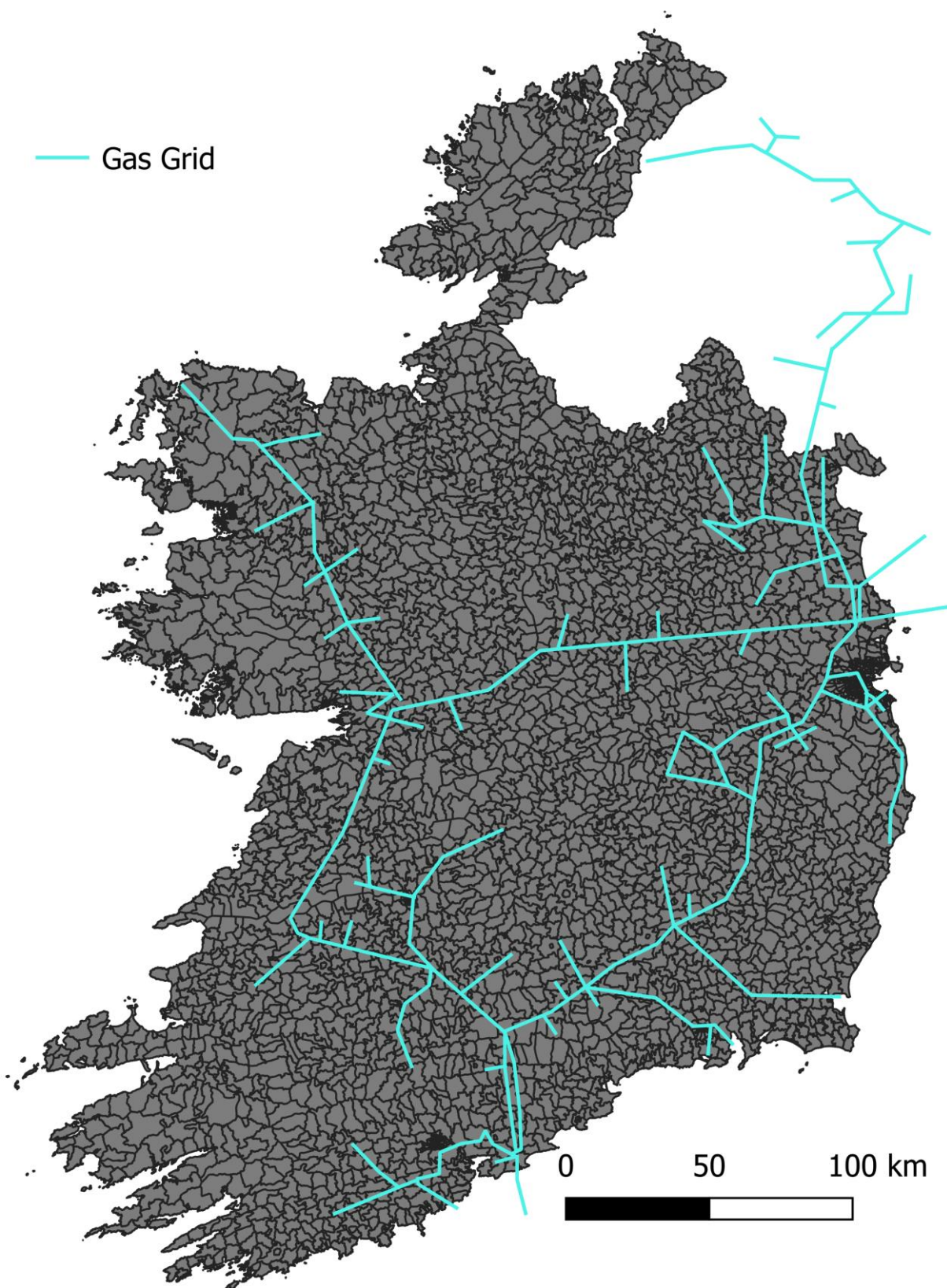
Figure 3-2: Existing gas grid network.
