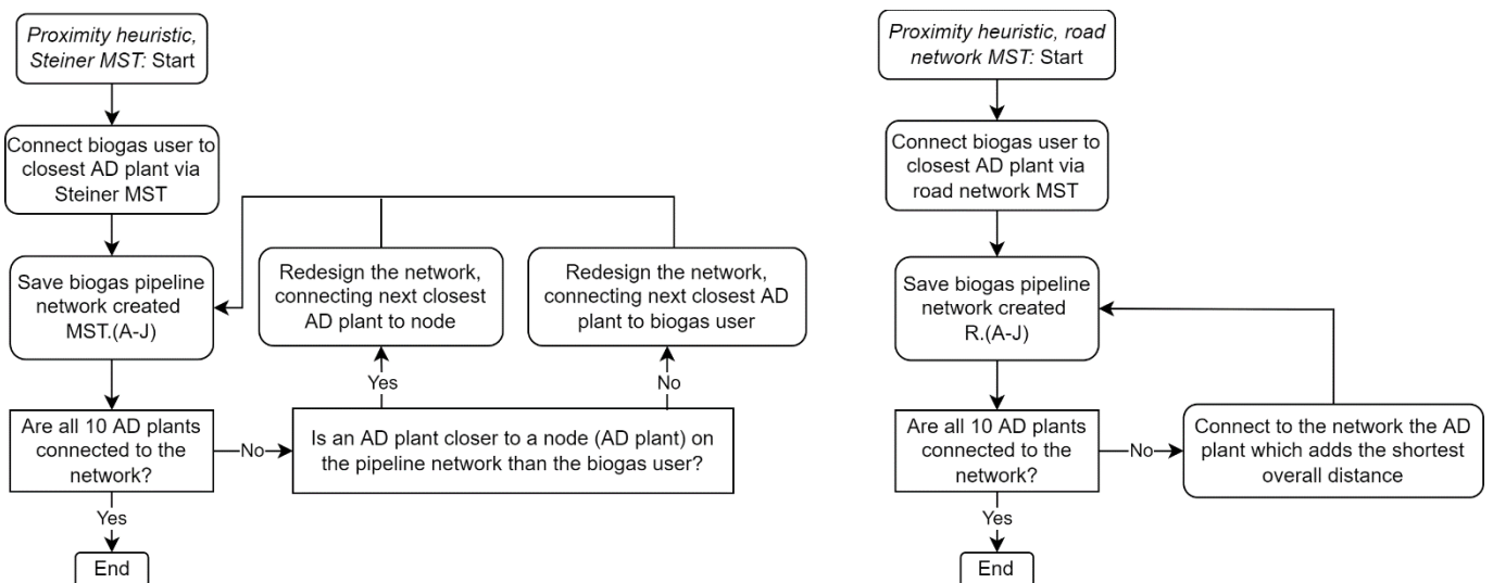
Figure 6-4: Flowchart methodology for proximity heuristic.
