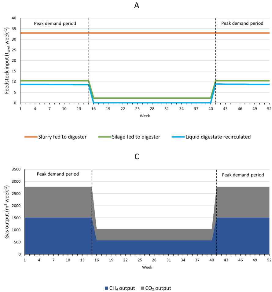
Figure 4-3: Scenario ZG-W, A) Weekly digester inputs, B) Digester solids content, C) Weekly digester gas output, D) Cumulative digestate bank.
