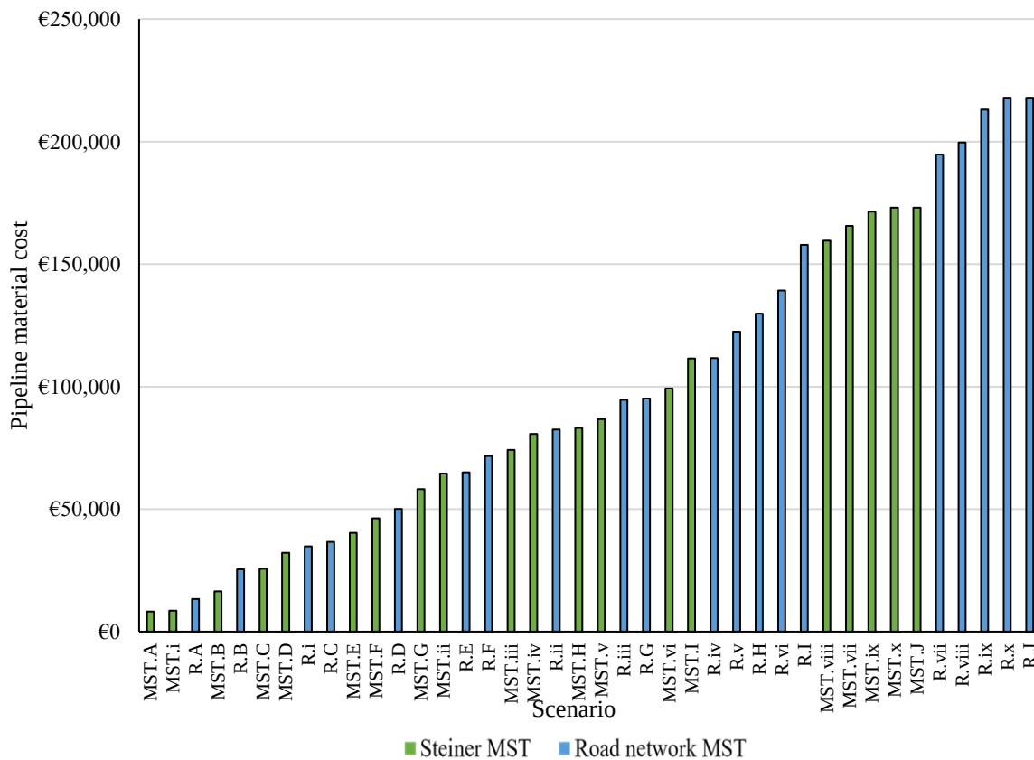
Figure 6-6: Scenarios ranked by pipeline material cost, from lowest to highest.
