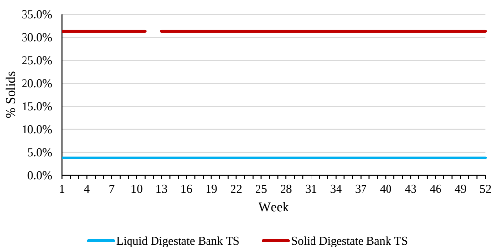
Figure B-1: Scenario ZG-C digestate bank solids content.
