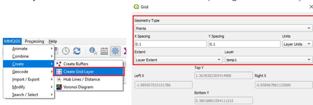
Figure D-2: MMQGIS grid of points creation.
