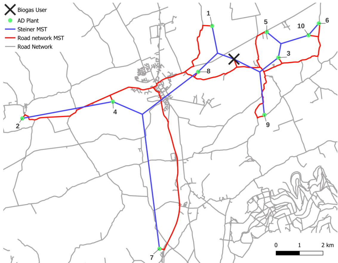
Figure 6-5: Biogas pipeline layouts connecting all AD plants either via Steiner MST or road network MST.
