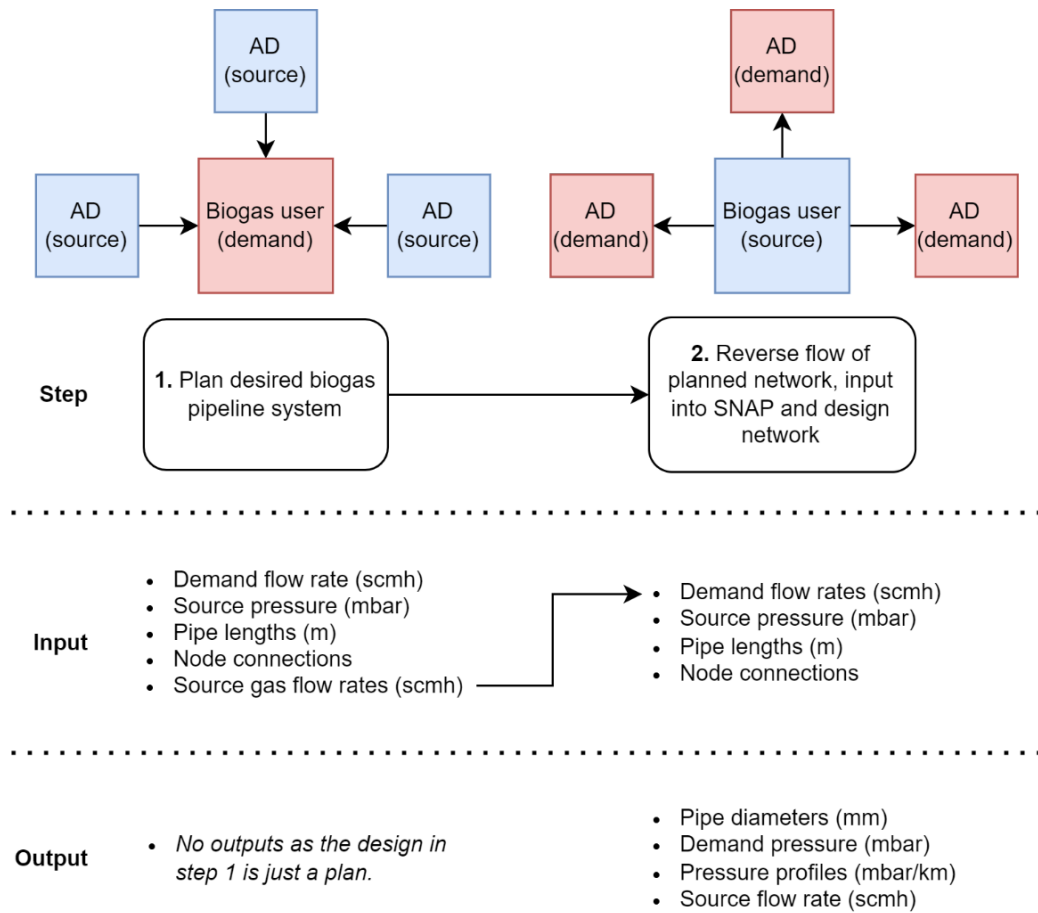
Figure D-21: SNAP methodology flowchart.
