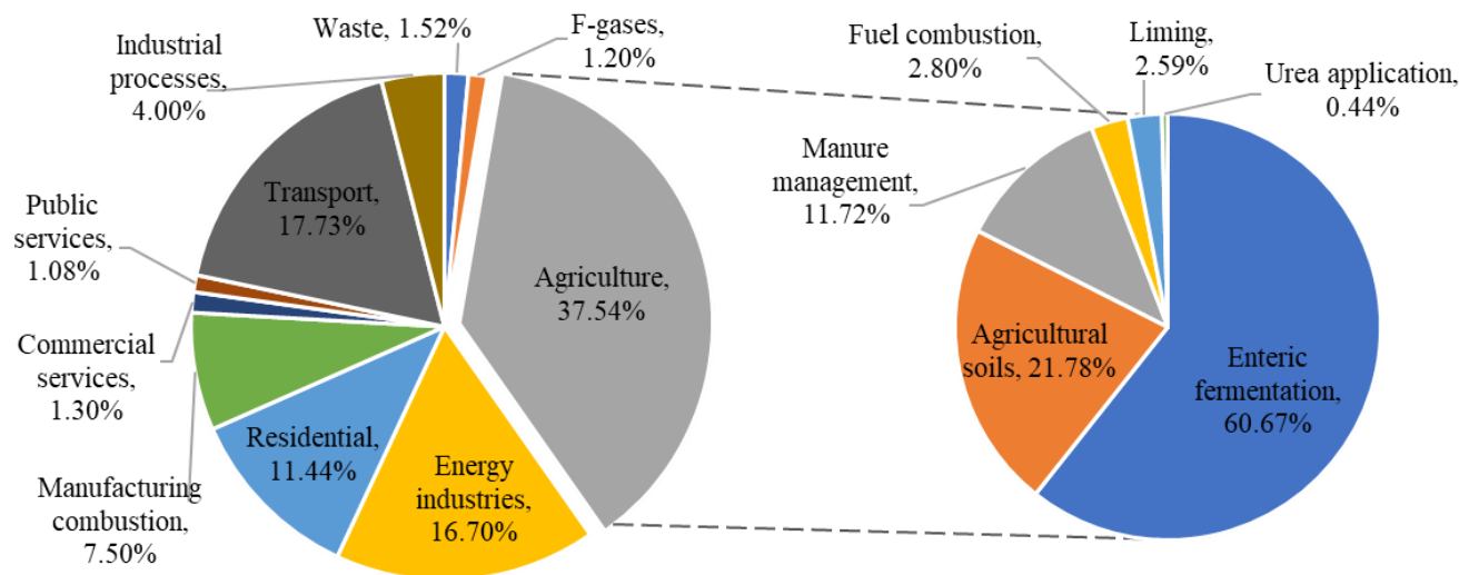
Figure 1-1: Ireland's GHG emissions by sector, and agricultural emissions (Environmental Protection Agency, 2022).
