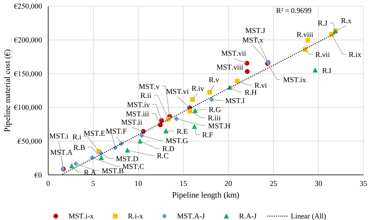
Figure 6-8: Scenario pipeline material cost vs. pipeline length.
