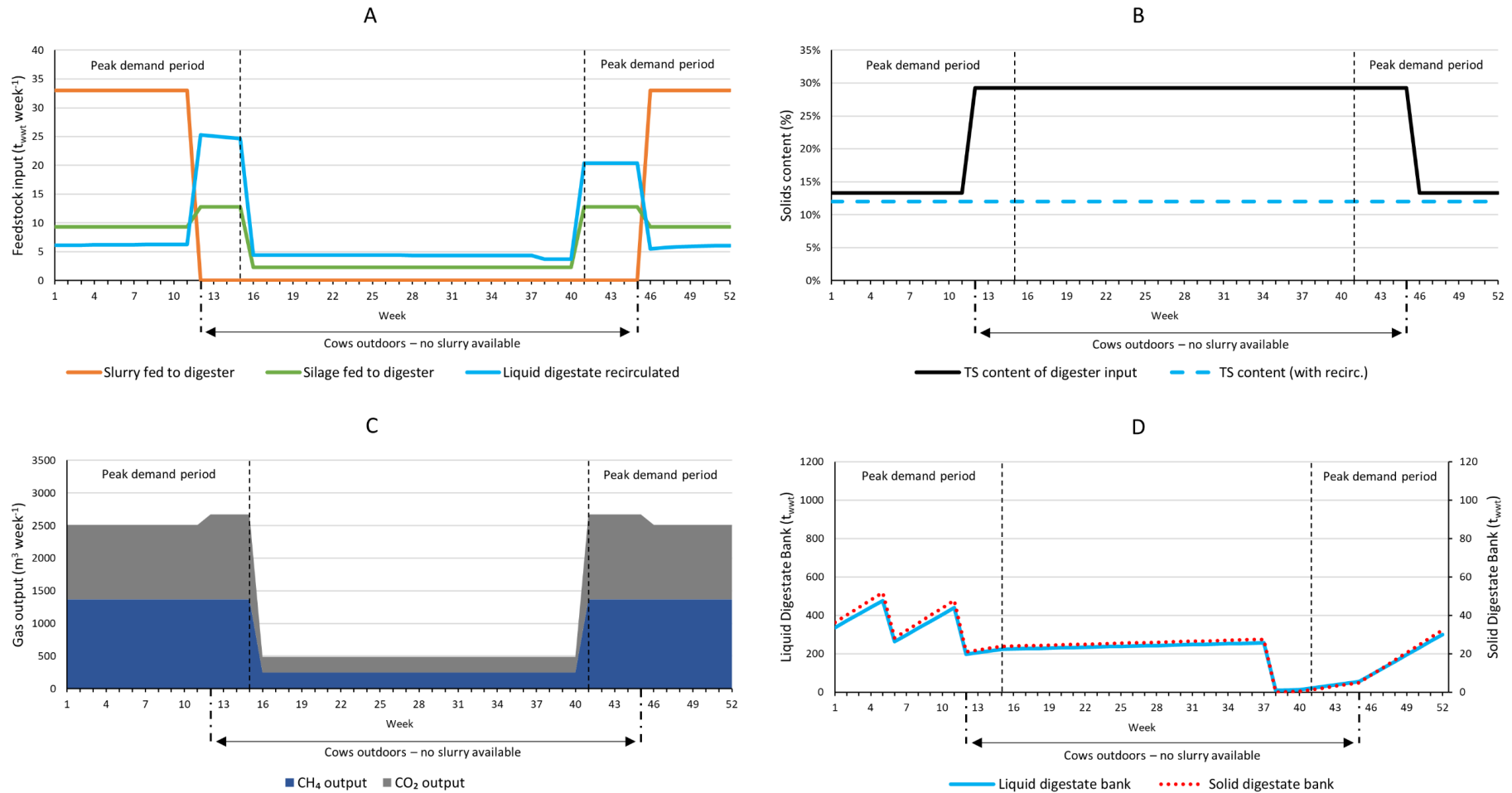
Figure 4-4: Scenario PB-W, A) Weekly digester inputs, B) Digester solids content, C) Weekly digester gas output, D) Cumulative digestate bank.
