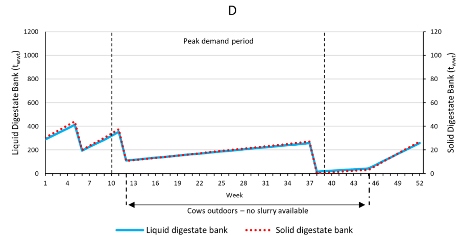
Figure 4-6: Scenario PB-S, A) Weekly digester inputs, B) Digester solids content, C) Weekly digester gas output, D) Cumulative digestate bank.
