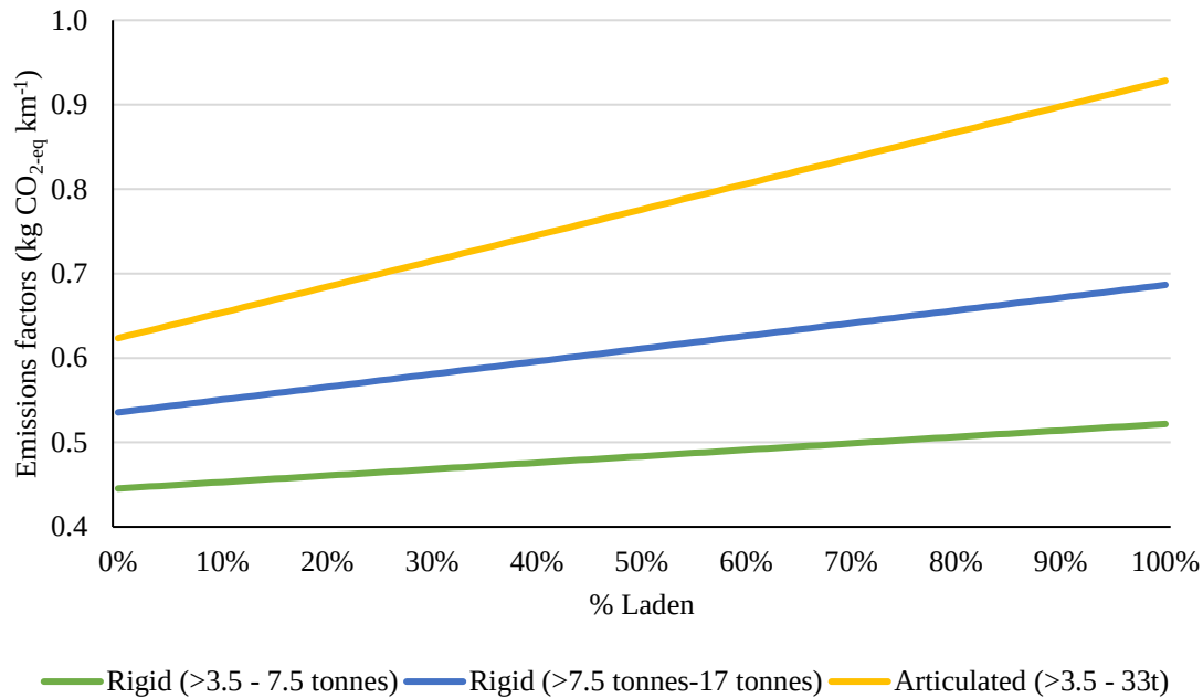
Figure 5-2: Emissions factors for different vehicle types (Department for Environment Food and Rural Affairs, 2021).
