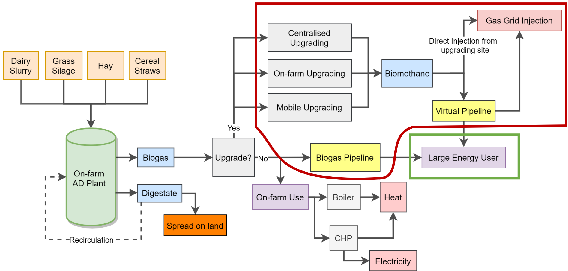
Figure 3-1: Flow diagram of on-farm AD logistical considerations.
