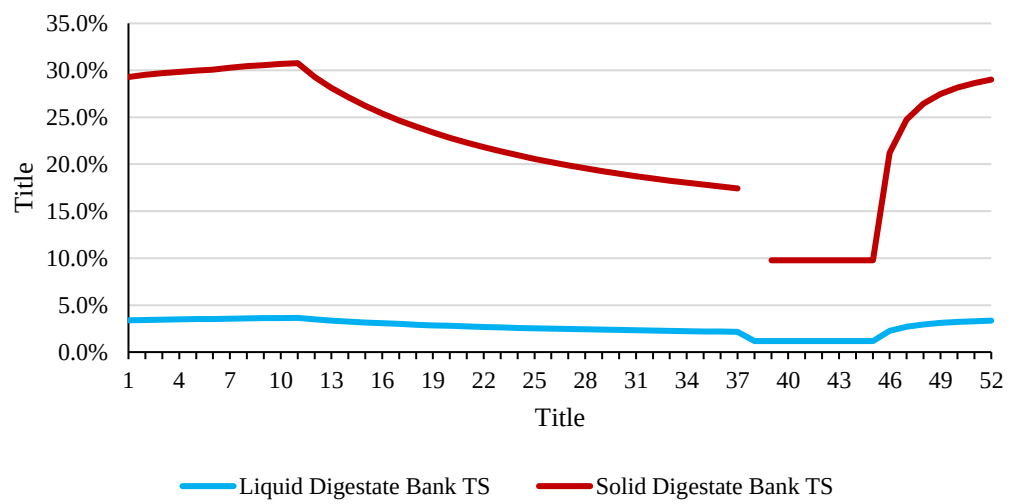
Figure B-6: Scenario PB-S digestate bank solids content.
