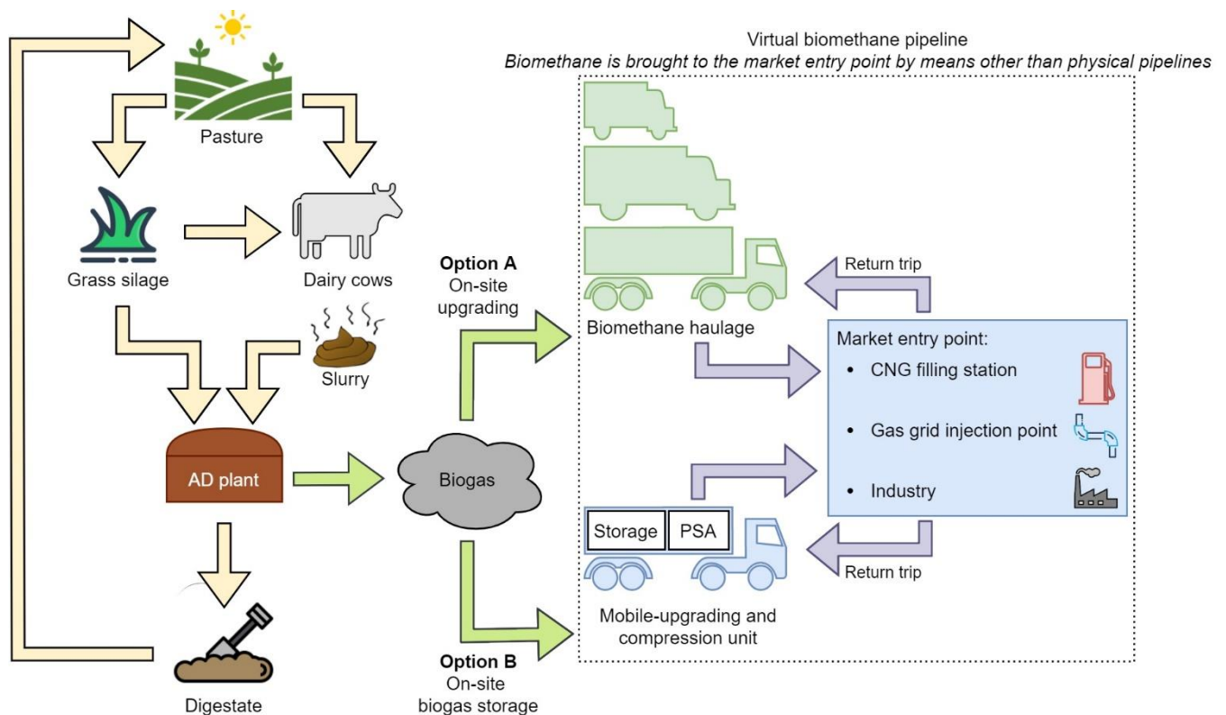
Figure 5-1: A virtual biomethane pipeline process supply chain, where biomethane is moved via haulage to the market entry point.
