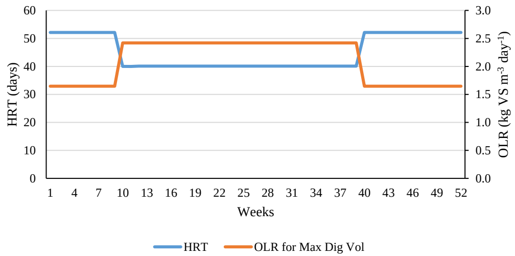
Figure B-11: Scenario ZG-S HRT and OLR.
