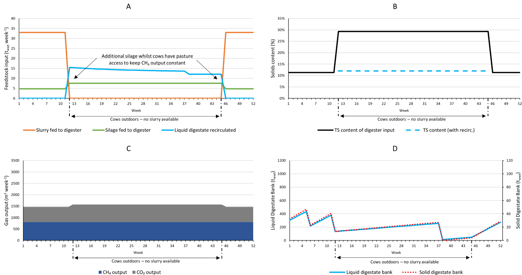
Figure 4-2: Scenario PB-C, A) Weekly digester inputs, B) Digester solids content, C) Weekly digester gas output, D) Cumulative digestate bank.
