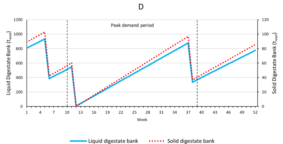
Figure 4-5: Scenario ZG-S, A) Weekly digester inputs, B) Digester solids content, C) Weekly digester gas output, D) Cumulative digestate bank.
