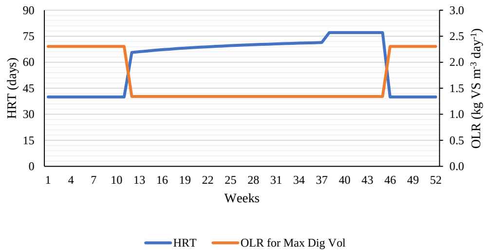
Figure B-8: Scenario PB-C HRT and OLR.
