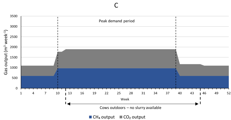
Figure 4-6: Scenario PB-S, A) Weekly digester inputs, B) Digester solids content, C) Weekly digester gas output, D) Cumulative digestate bank.
