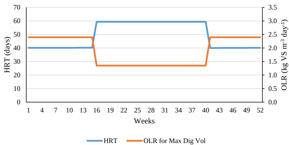
Figure B-9: Scenario ZG-W HRT and OLR.
