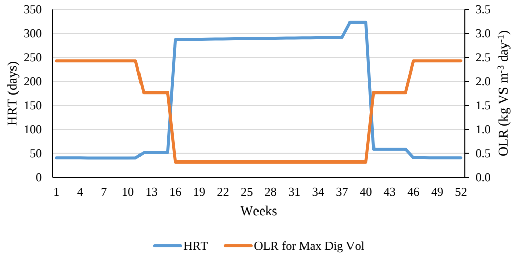
Figure B-10: Scenario PB-W HRT and OLR.
