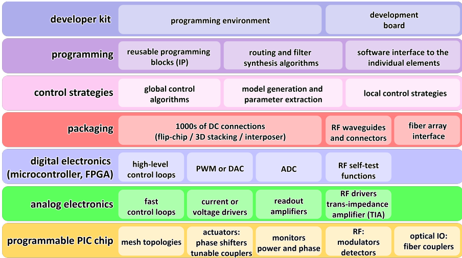
Figure 3. Technology stack for programmable photonics. 4,6 To realize a programmable photonics system, one needs to combine the photonic chip with analog and digital driver electronics and software layers.
