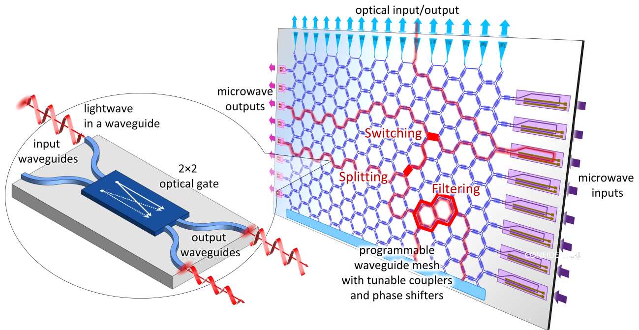
Figure 1. General-purpose programmable photonic processor: A waveguide mesh consisting of optical gates (containing phase shifters and/or tunable couplers) connects functional building blocks and waveguide ports. Optical signals can be routed, distributed, or filtered by tuning the coupling and phase delay in the optical gates. High-speed microwave signals can be converted into optical signals through modulators and back into microwave signals through high-speed photodetectors.
