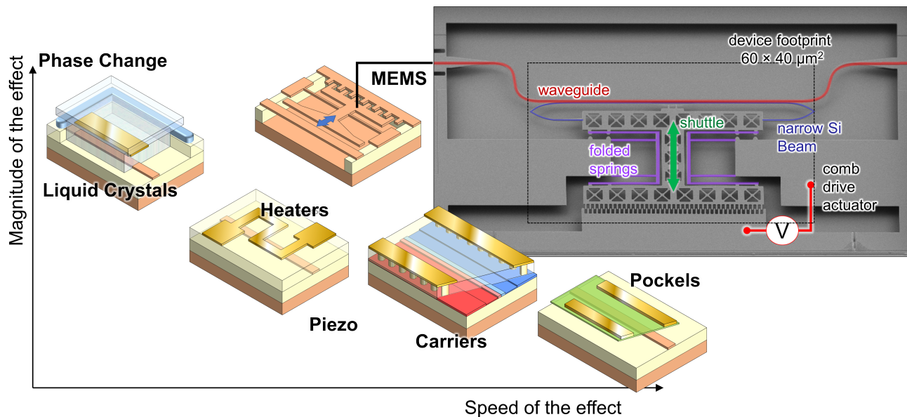
Figure 4. Electro-optic actuation mechanisms, classified by the speed of the effect and the magnitude. The stronger the effect, the shorter and more compact the phase shifter can be implemented. Inset: A MEMS Phase shifter developed in the MORPHIC project. 23
