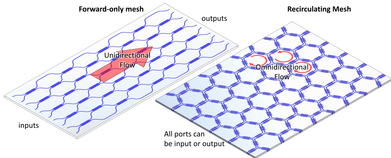
Figure 2. Waveguide mesh architectures. Left: a forward-only mesh, where light flows in one direction from a set of input ports to a set of output ports. Right: a recirculating mesh, where light is coupled from one unit cell to the next and can travel between any pair of ports.
