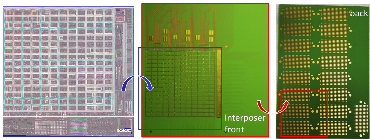
Figure 5. Interposer technology developed in the MORPHIC project. 46 The silicon photonics chip can have up to 3305 electrical connections on a fixed grid. A ceramic interposer breaks out these bond pads to a much wider pitch compatible with standard printed circuit board technology. The interposer also supports up to 24 high-speed connections for modulators and photodetectors.
