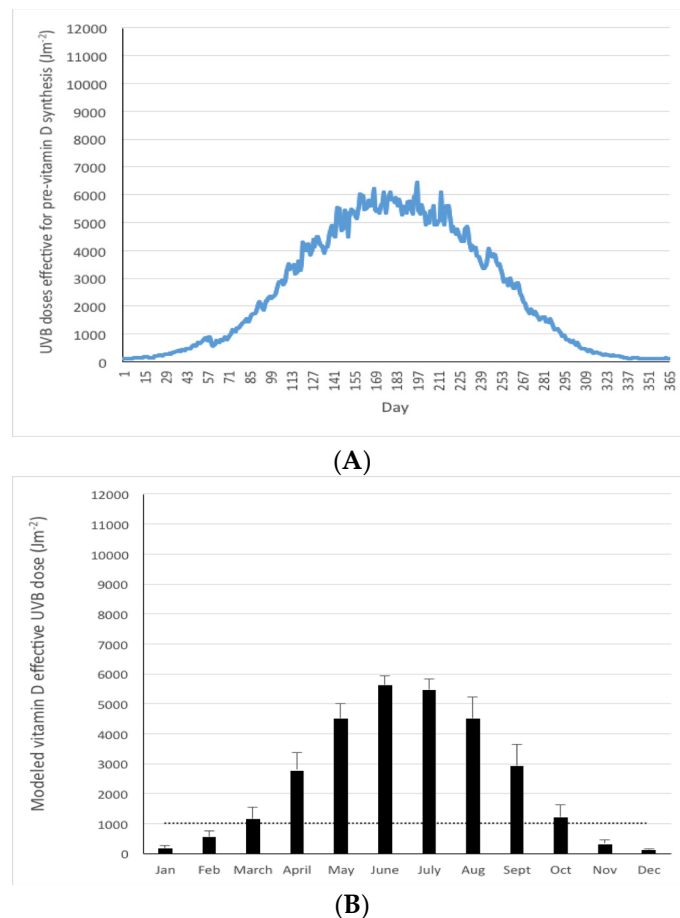
Figure 1. Mean modeled UVB doses effective for pre-vitamin D 3 synthesis ( \text{Jm}^{-2} ) in Germany (47–55° N) on a daily (A) and monthly (B) basis in a typical year (mean of 2003–2012). Dotted line in panel B reflects a threshold of 1000 \text{ Jm}^{-2} as a guide to a dose below which dermal synthesis of pre-vitamin D 3 is relatively low.
