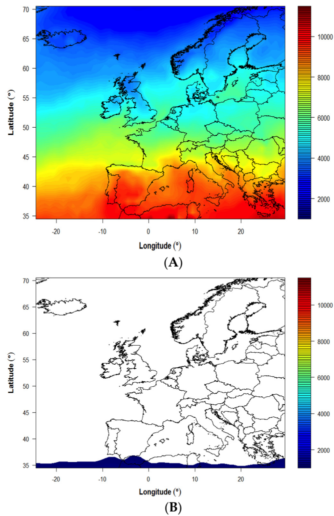
Figure 3. Mean monthly modeled UVB doses effective for pre-vitamin D 3 synthesis ( \text{Jm}^{-2} ) across Europe for June (A) and December (B), based on average of data from years 2003–2012. Scale begins 1000 \text{ Jm}^{-2} .
