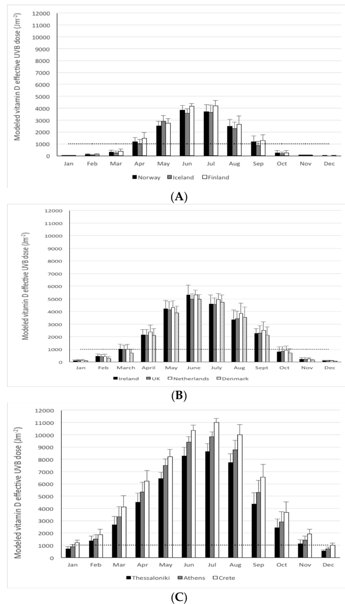
Figure 2. Mean modeled UVB doses effective for pre-vitamin D 3 synthesis (Jm -2 ) in Norway (mean of Oslo (60° N) and Tromsø (69° N)), Iceland (Reykjavik (64° N)) and Finland (60–70° N) (A); Ireland (51–54° N), the UK (50–59° N), Netherlands (Amsterdam, (52° N)), and Denmark (mean of Copenhagen and Aarhus (56° N)) (B); and Thessaloniki (40° N), Athens (37° N) and Crete (35° N) (C) on a monthly basis in a typical year (mean of 2003–2012). Dotted line reflects a threshold of 1000 Jm -2 as a guide to a dose below which dermal synthesis of pre-vitamin D 3 is relatively low.
