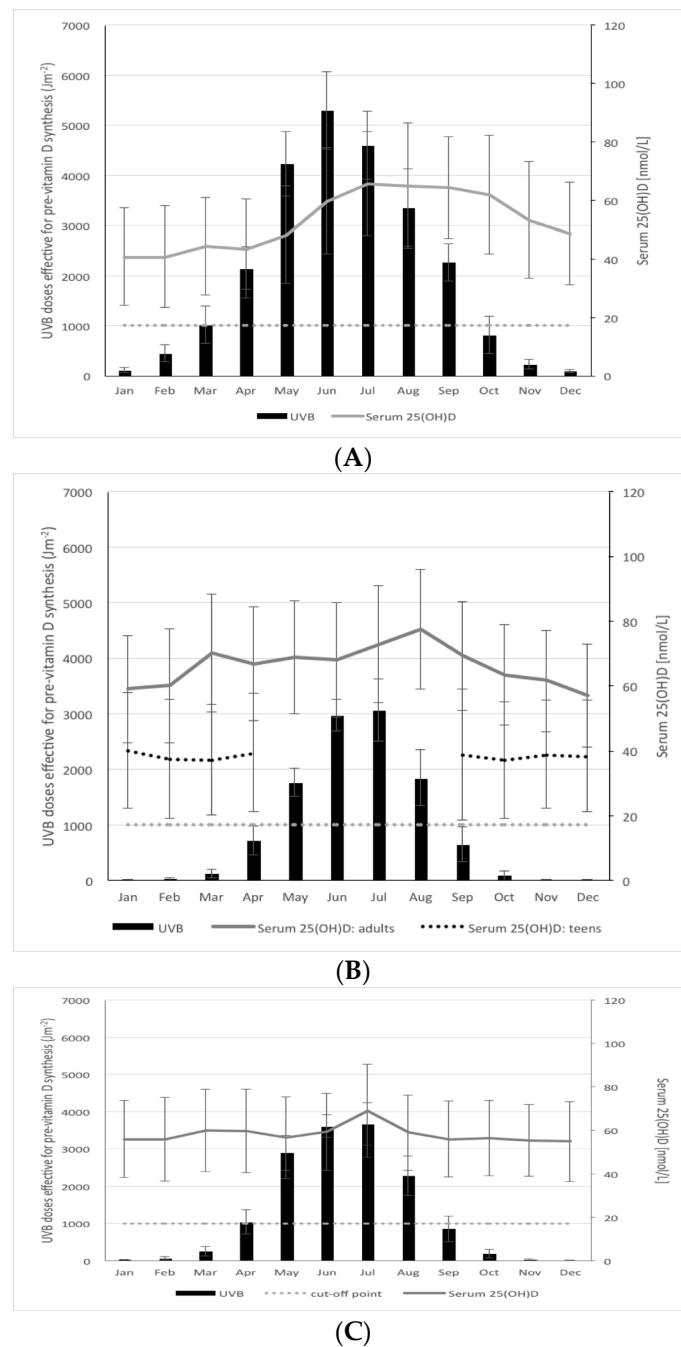
Figure 4. Mean modeled UVB doses effective for pre-vitamin D 3 synthesis (Jm -2 ) on a monthly basis in a typical year (mean of 2003–2012) in Ireland (51–54° N) and mean (SD) monthly serum 25(OH)D measured in adults (18–84 years) in the National Adult Nutrition Survey in Ireland [21] (A); in Tromsø, Northern Norway (69° N) and mean (SD) monthly serum 25(OH)D measured in adults (18–83 years) in the regionally representative Tromsø sixth cycle cohort [17] (solid line) and adolescents (15–18 years) in the Tromsø—Fit Futures study [18] (dotted black line) (B); and in Reykjavik, Iceland (64° N) and mean (SD) monthly serum 25(OH)D measured in adults (aged 66–96 years) in the regionally representative AGES-Reykjavik cohort in Iceland [19] (C). Note: Data on serum 25(OH)D for the four summer months (May to August) are absent in Tromsø—Fit Futures study as the adolescents were not sampled in this period due to school summer vacation. Dotted line reflects a threshold of 1000 Jm -2 as a guide to a dose below which dermal synthesis of pre-vitamin D 3 is relatively low. Black bars and error bars represent mean and SD monthly UVB doses, respectively.
