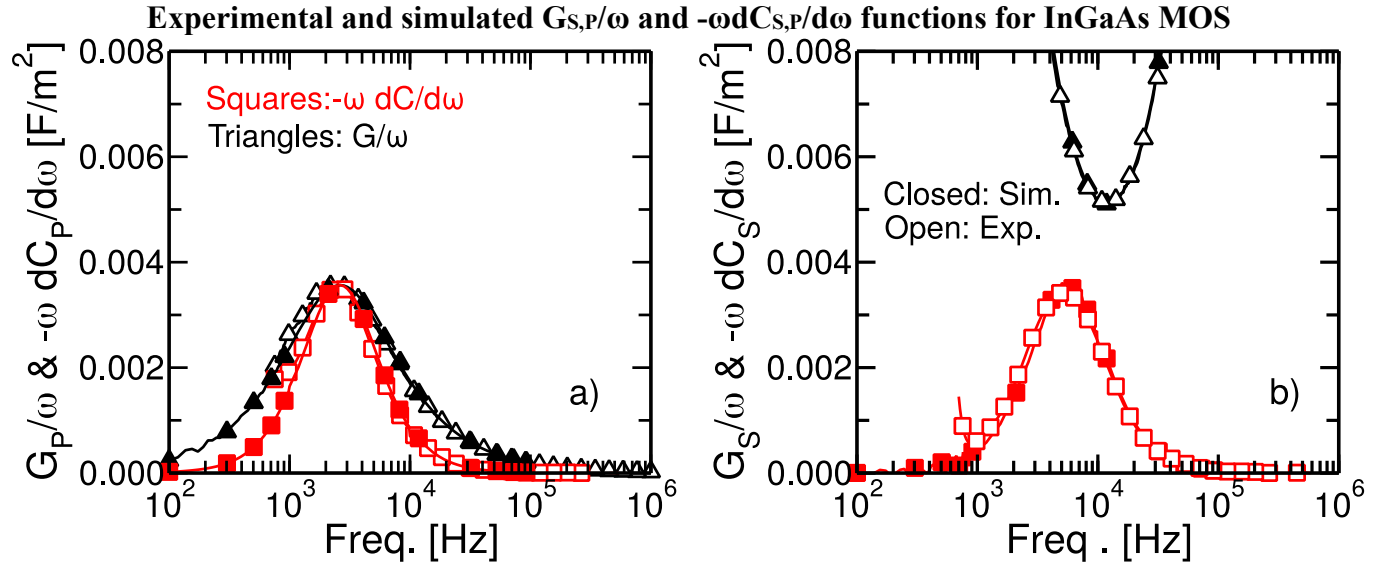
Figure 6. (a) G_P/\omega (triangles) and -\omega dC_P/d\omega (squares) functions constructed from the InGaAs MOS C(\omega, V)/G(\omega, V) responses shown in Figure 5 ( V_G = -3\text{V} ), (b) corresponding G_S/\omega and -\omega dC_S/d\omega . Simulations based on C_{OX} = 0.098 \text{ F/m}^2 , \tau_g = 80 \text{ ps} and N_D = 4.6 \times 10^{17} \text{ cm}^{-3} are in excellent agreement with the measurements for both circuit modes; the extracted N_D is in agreement with ECV measurements.
