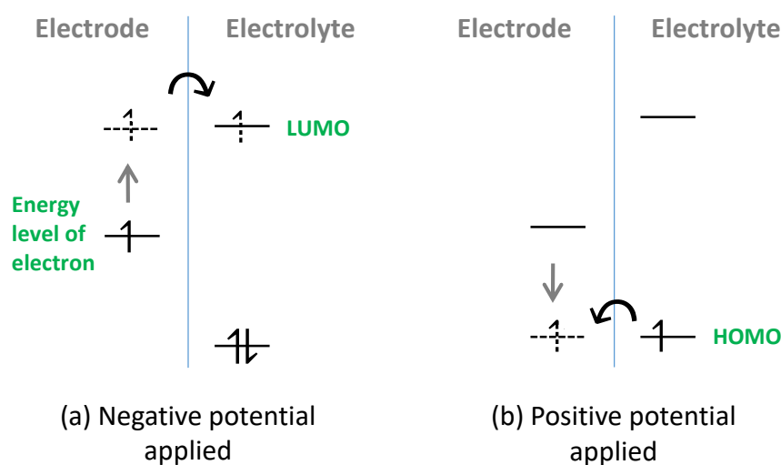
Figure 1.2: Representation of (a) a reduction of a species in solution where an electron moves into the LUMO of the electrolyte and (b) an oxidation of a species where it gains an electron from the HOMO of the electrolyte.
