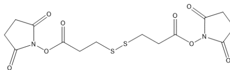
dithiobis(succinimidyl propionate)
