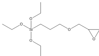
3-glycidoxypyltrimethoxysilane
