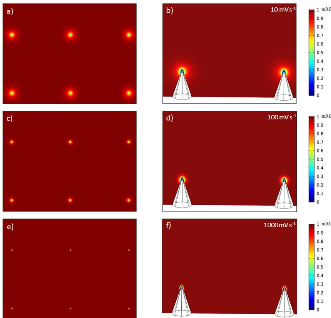
Figure 3.9: 1 mM FcCOOH concentration profile at 6.0 V for 3 x 2 array of electroactive tips (radius 20 \mu\text{m} ) with 1750 \mu\text{m} pitch at, shown top down (left) and side on (right) at (a, b) 10, (c, d) 100 and (e, f) 1000 \text{mV s}^{-1}
