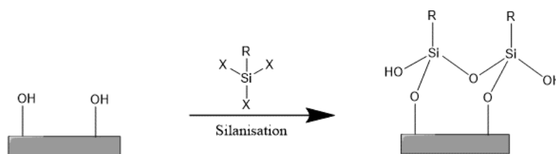
Figure 1.23: Schematic representation of possible mode of covalent attachment of a \text{RSiX}_3 to a hydroxyl-terminated surface, with cross-linking between adjacent silane molecules.
