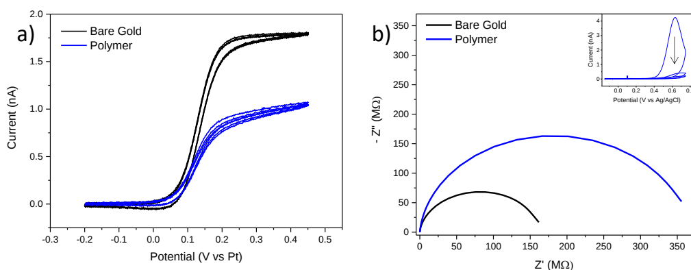
Figure 2.5: (a) CV at 50 \text{mV s}^{-1} and (b) EIS with 5 mV amplitude applied to 200 mV in 1 mM \text{FcCOOH} in 10 mM PBS before (black) and after (blue) the deposition of poly (aniline-co-o-anthranilic acid) in 0.5 M \text{H}_2\text{SO}_4 . Inset electropolymer deposition of poly (aniline-co-o-anthranilic acid) for 3 cycles at 50 \text{mV s}^{-1} . Arrow indicates the reduction of the oxidation peak with increasing cycle number.
