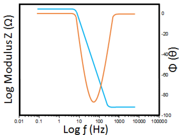
Figure 1.13: Bode plot with the impedance modulus (blue) and the phase angle (orange) vs log of the frequency.
