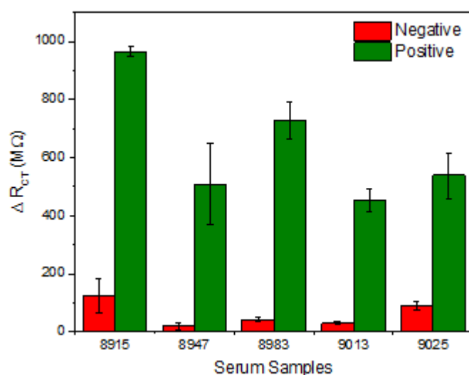
Figure 2.11: Bar chart comparison of R_{ct} for IgG negative serum samples with their respective IgG positive serum samples, with their respective NANNYcare® baseline subtracted. Samples were diluted 1:10 in 10 mM PBS pH 7.4.
