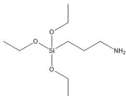
3-aminopropyltriethoxysilane
