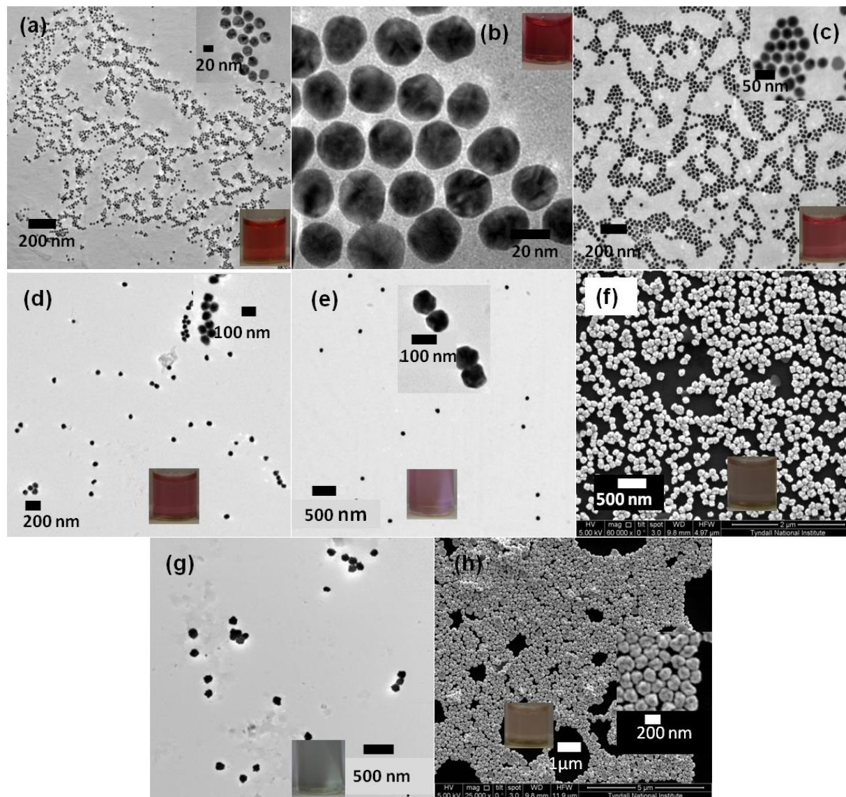
Figure 2. TEM micrographs of Au nanoparticles produced in this study with mean diameters of (a) ~15 nm (b) ~ 23 nm, (c) ~30 nm (d) ~ 63 nm (e) ~93 nm and (g) ~135 nm. SEM images of Au nanoparticles with diameters of (f) ~115 nm (h) ~170 nm. The insets show higher magnification electron micrographs, and optical photographs of the the corresponding colloidal solutions.
