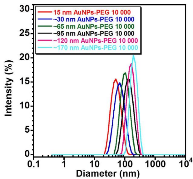
Figure 4. Size distribution by intensity of different AuNPs sizes coated with the mPEG 10 000 -SH (~245 EO units).
