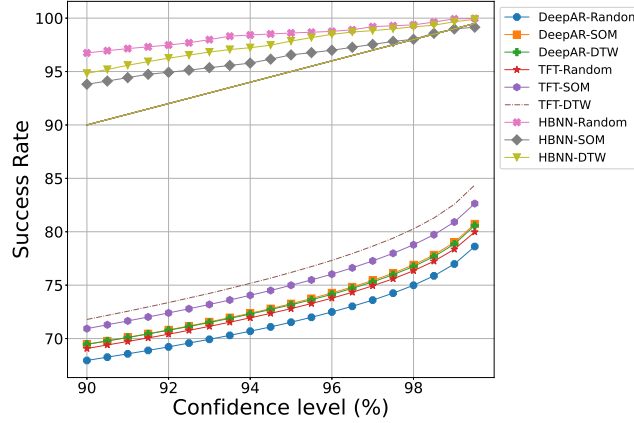
Fig. 2. Memory SR comparison of DeepAR, TFT and HBNN as a function of the confidence level with models trained with 1000 datasets. The model is the most accurate when the curve is closest to the line y = x . DTW and SOM-based selections improve the SR compared to the random selection of datasets.
