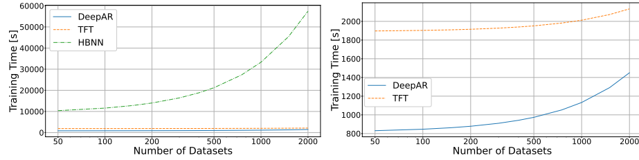
Fig. 4. Training time curve as a function of the number of datasets. On the left, all three models are plotted. On the right, we plot only DeepAR and TFT to show the differences between the two models. The training time increases when we increase L , but TFT grows slower when the number of datasets increases, compared to the other methods. The x-axis is in a logarithmic scale.
