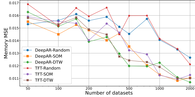
Fig. 1. MSE comparison of DeepAR and TFT for the memory demand. DTW and SOM are the best clustering-based selection approaches and allow the models to achieve the same MSE with fewer training datasets compared to a random selection. When the number of datasets is high, the MSE of all the approaches converge. The x-axis is in a logarithmic scale.
