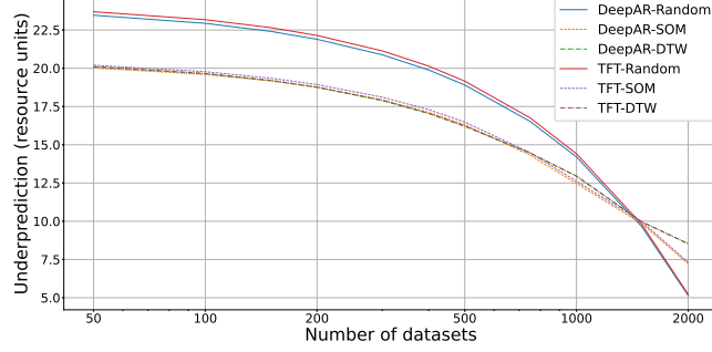
Fig. 3. Memory OP comparison of DeepAR and TFT. If DTW and SOM are applied, a much lower number of datasets is required to get the same OP compared to a random selection of the datasets. The x-axis is in a logarithmic scale.
