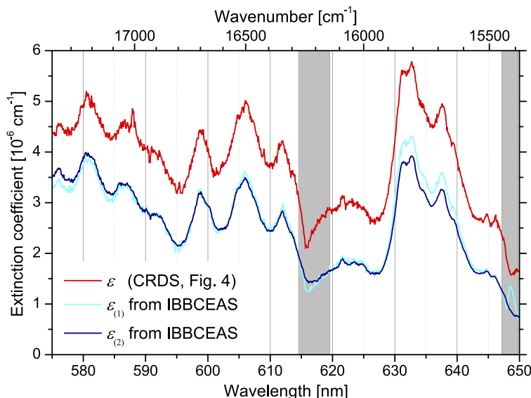
Fig. 6. Red trace: Broadband CRDS spectrum of gaseous static azulene in ambient air from Fig. 4. Blue traces: IBBCEAS spectra from Fig. 4 corrected using CRDS-based evaluation (1)-light blue ( \epsilon_{(1)} ), and CEAS-based evaluation (2)-dark blue ( \epsilon_{(2)} ).
