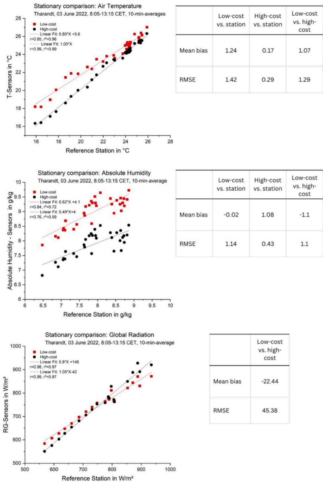
Fig. 5. Statistical results for the stationary comparison of the low-cost UrbanMobiClim and high-cost TUD backpack sensors to the reference weather station in Tharandt on 03 June 2022 with results for R^2 , mean bias, and RMSE.
