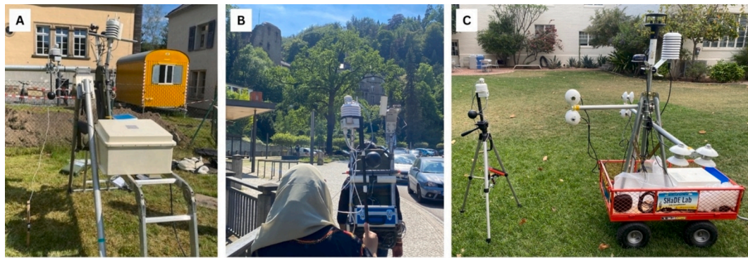
Fig. 4. Experimental set up for (A) Stationary comparison in Tharandt with UrbanMobiClim (left) and TUD backpack device (right) side by side (B) UrbanMobiClim (foreground) and TUD backpack device (background) being carried during the mobile comparison in Tharandt (C) Stationary comparison at Arizona State University courtyard location with UrbanMobiClim (left) and the MaRTy device (right) (Photos: Anonymous).
