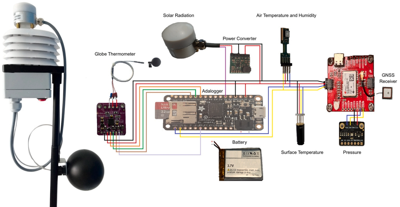
Fig. 1. Overview of the new low-cost mobile monitoring device, UrbanMobiClim, including: a picture of the device (left); device schematic (right), where red and black represent power lines, yellow and blue represent communication lines, other colours represent additional connections. (For interpretation of the references to colour in this figure legend, the reader is referred to the web version of this article.)
