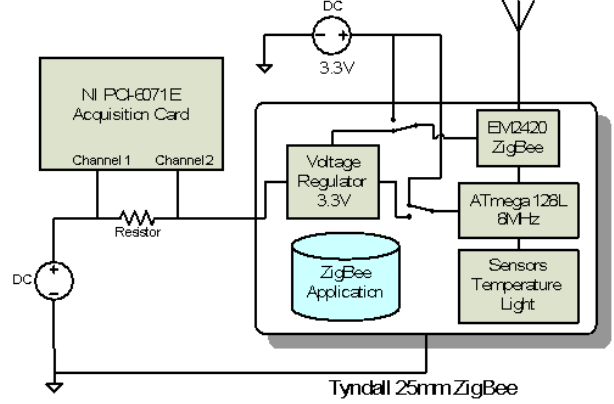
Figure 2. Measurement setup.
