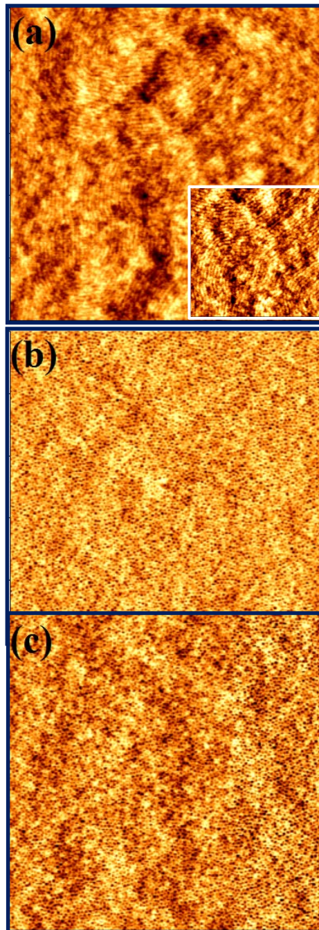
Figure 3 Tapping mode AFM images of a PS-PEO (16-5) thin film annealed in \text{scCO}_2 environment at a pressure of 100 bar and at a temperature of 45 °C for (a) 1 h (b) 1 h 30 m and (c) 2 h. Scale bar: 2 x 2 \mu\text{m} .
