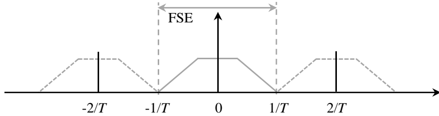
Figure 4.7: An FSE with tap spacing \tau > 2|f| satisfies the sampling theorem.
