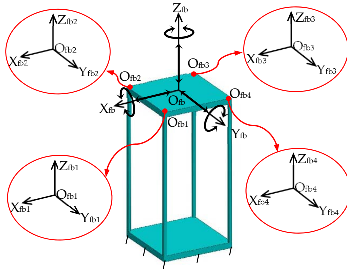
Figure 3.3 Illustration of a four-beam NBCM, the global coordinate system O_{fb}-X_{fb}Y_{fb}Z_{fb} , and the local coordinate systems O_{fb1}-X_{fb1}Y_{fb1}Z_{fb1} , O_{fb2}-X_{fb2}Y_{fb2}Z_{fb2} , O_{fb3}-X_{fb3}Y_{fb3}Z_{fb3} and O_{fb4}-X_{fb4}Y_{fb4}Z_{fb4}
