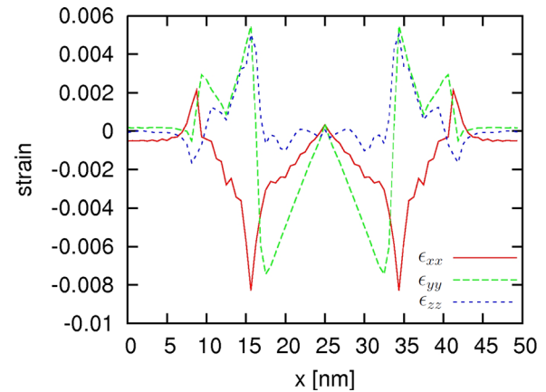
FIG. 5. (Color online) Diagonal components of the strain tensor plotted along the [010]-direction through the center of the dot and two leaves.
