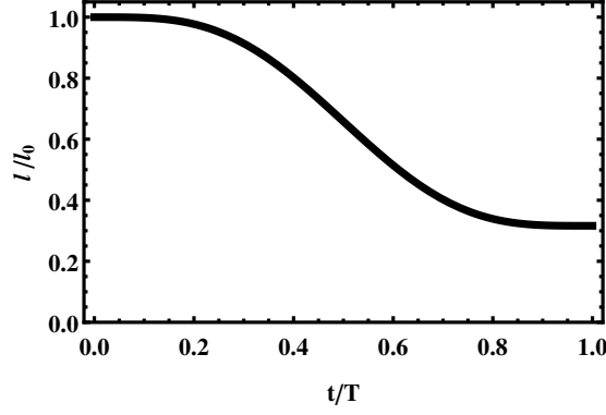
FIGURE 6.1: Auxiliary function l(t) versus t .
