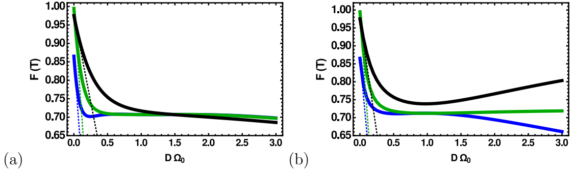
FIGURE 7.3: RAP scheme in a two-level system with H_0 \neq H_1 . \delta_0 = 3.5 \Omega_0 (black), \delta_0 = 1 \Omega_0 (green), \delta_0 = 0.5 \Omega_0 (blue). Numerically exact solution (solid lines) and small noise approximation (7.35) (dotted lines). (a) Fidelity F(T) against noise strength D for frequency error. (b) Fidelity F(T) against noise strength D for both timing and frequency error with c = 1 .
