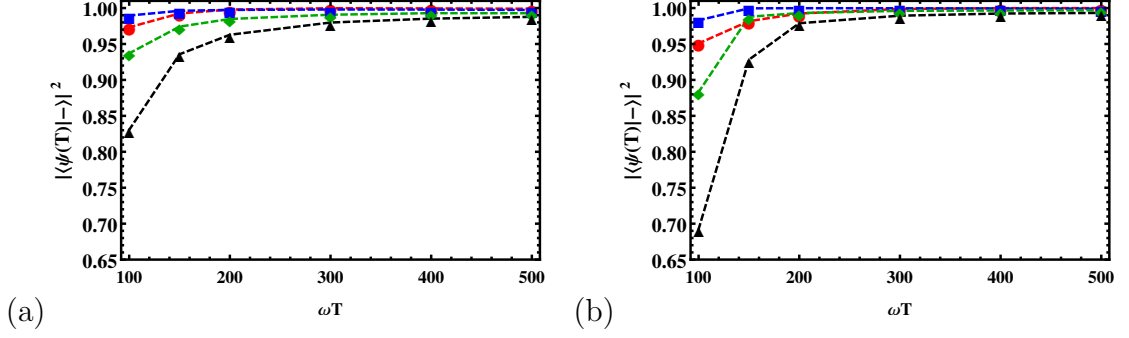
FIGURE 5.6: Fidelity |\langle\psi(T)|-\rangle|^2 against total time T for different lattice depths V_0 for a fixed trapping frequency \omega . Points joined with lines: V_0 = 2\hbar\omega (red circles), V_0 = 2.5\hbar\omega (blue squares), V_0 = 3\hbar\omega (green diamonds) and V_0 = 3.5\hbar\omega (black triangles); (a) polynomial scheme, (b) piecewise scheme ( t_S = 0.75T ).
