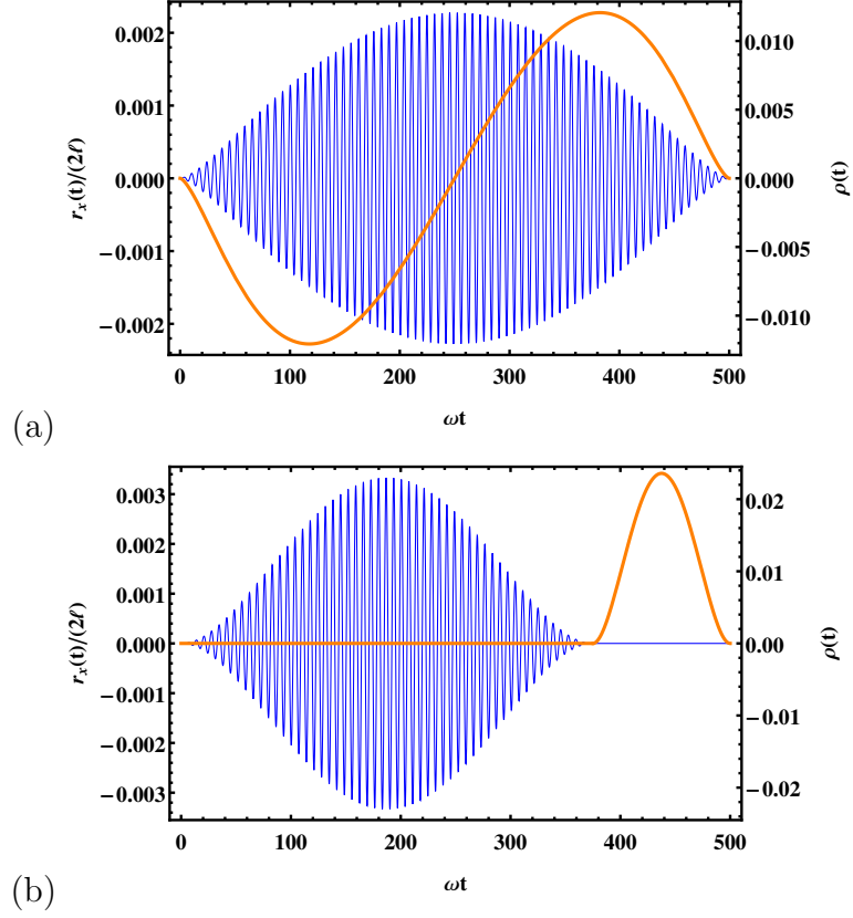
FIGURE 5.4: Shaking function r_x(t) with \omega_x = -\omega_d (thin, blue line) and relative phase between the polarisation vectors \rho(t) (thick, orange line) versus time for (a) the polynomial scheme and (b) the piecewise scheme ( t_S = 0.75T ). V_0 = 3\hbar\omega , T = 500\omega^{-1} and 2l = \pi/k is the lattice constant.
