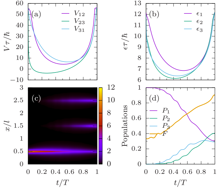
FIGURE 4.7: Same as figure 4.6(a-d) but for SNAP superposition scheme given in (4.27) in the continuum model. T/\tau = 400 . F = |\langle\psi_{\text{target}}|\psi(t)\rangle|^2 is the fidelity of the process.
