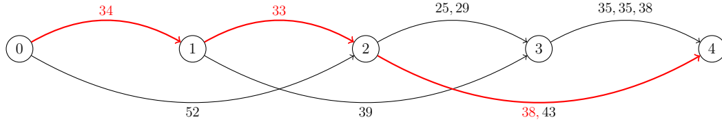
Figure 4.5: The network representation of the example problem with all possible cycle costs. The best path is highlighted in red.
