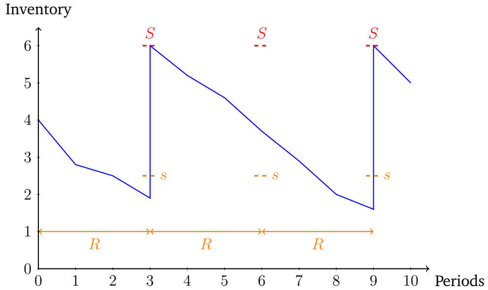
Figure 2.6: The expected inventory level under the (R, s, S) policy
