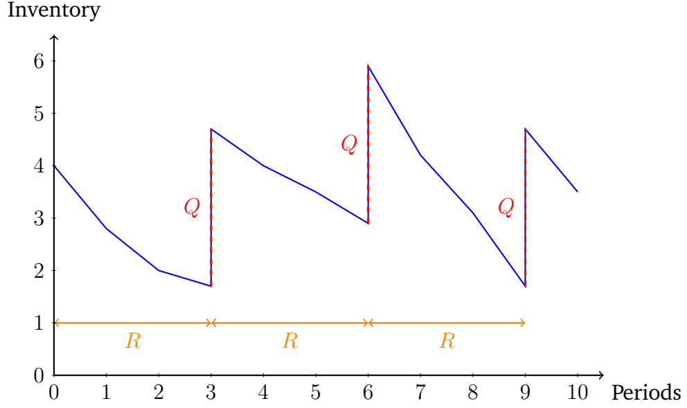
Figure 2.4: The expected inventory level under the (R, Q) policy
