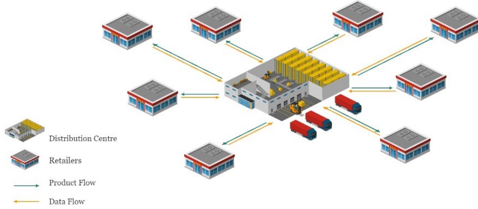
Figure 3.1: Schematic representation of the supply chain network.
