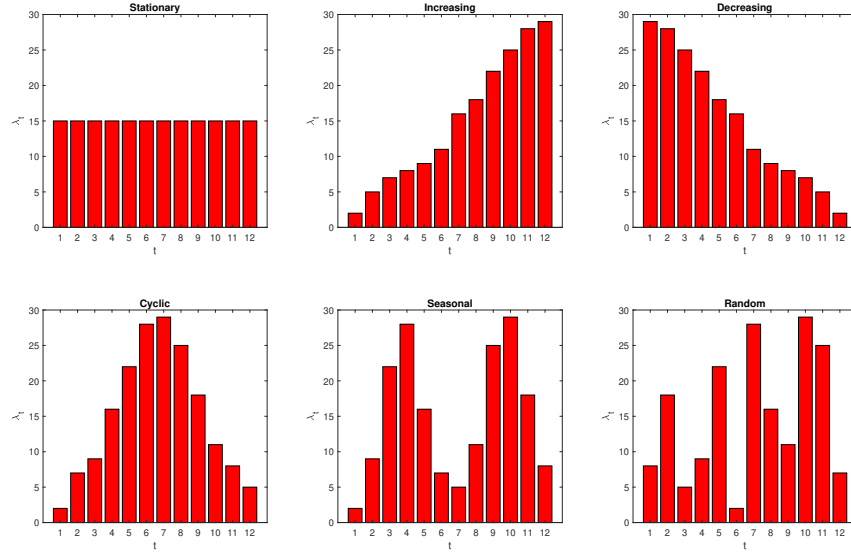
Figure 2.1: Various examples of demand mean patterns.
