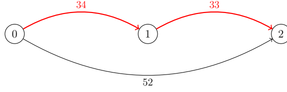
Figure 4.9: The best path at the end of period 2 with the corresponding cycle cost values.
