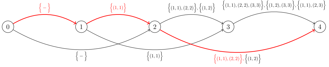
Figure 4.7: The network representation of the example problem with the previous replenishment cycle information. The best path is highlighted in red.
