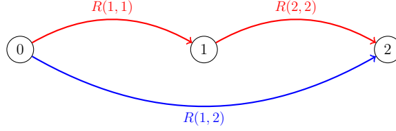
Figure 4.3: The possible paths to the end of period 2.
