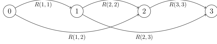
Figure 5.1: The network representation of all possible replenishment cycles of a perishable inventory model with T = 3 and M = 2 . Notice that each Node i = 1, \dots, T - 1 represent the end of Period i and the beginning of Period i + 1 , Node 0 and Node T represent the beginning and the ending of the planning horizon, respectively, and each arc (i, j) : i = 0, \dots, T - 1, j = 1, \dots, T, i > j , represents R(i + 1, j) .
