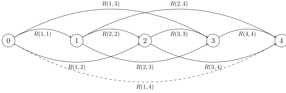
Figure 4.1: The network representation of all possible replenishment cycles of a perishable inventory model with T = 4 and M = 3 . Notice that each Node i = 1, \dots, T - 1 represent the end of Period i and the beginning of Period i + 1 , Node 0 and Node T represent the beginning and the ending of the planning horizon, respectively, and each arc (i, j) : i = 0, \dots, T - 1, j = 1, \dots, T, i < j , represents R(i + 1, j) .
