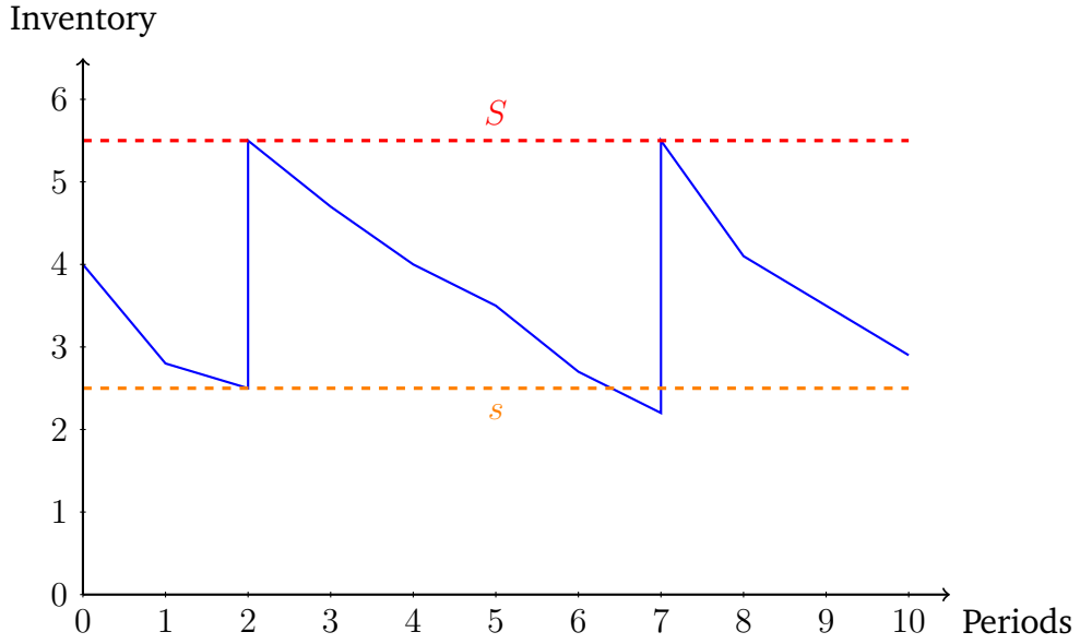
Figure 2.3: The expected inventory level under the (s, S) policy
