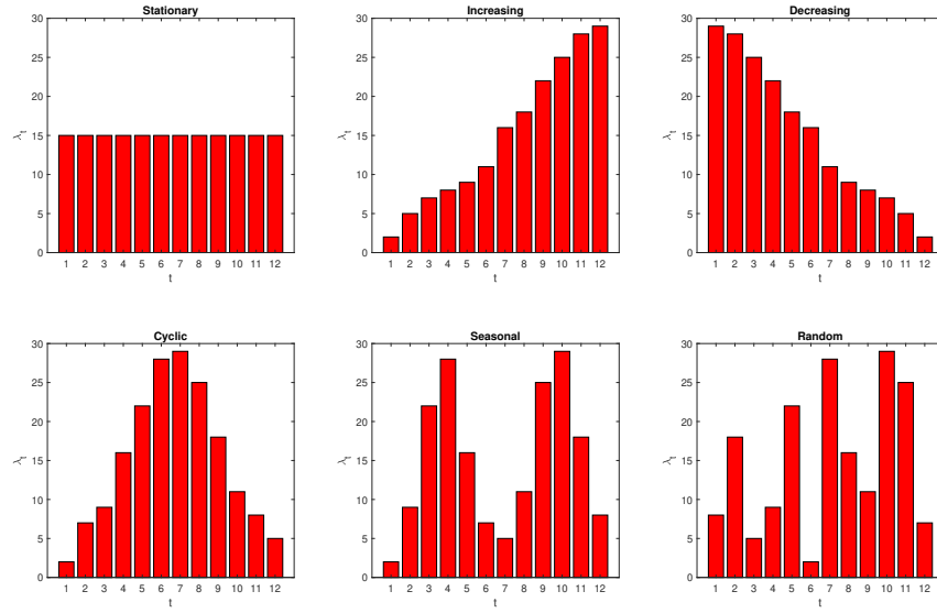
Figure 4.10: Demand patterns for each demand set.
