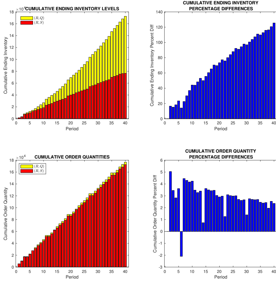
Figure 3.2: Comparison of the cumulative ending inventory levels and percentage differences found via the (R, Q) and (R, S) models.
