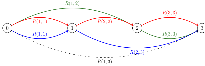
Figure 4.4: The possible paths to the end of period 3.
