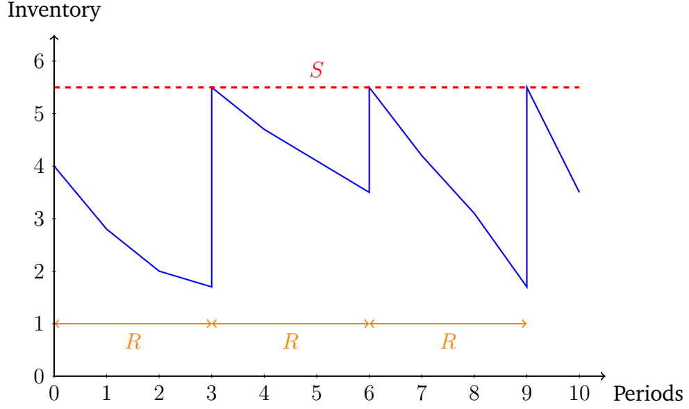
Figure 2.5: The expected inventory level under the (R, S) policy
