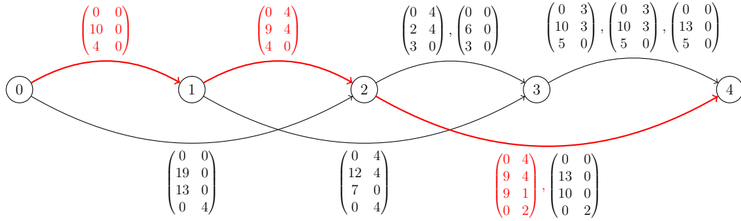
Figure 4.6: The network representation of the example problem with all possible inventory compositions. The best path is highlighted in red. The first and the second row represent the starting inventory at the beginning of the replenishment cycle and the inventory composition after the order is placed, respectively. The remaining rows show the inventory compositions at the end of each period in the replenishment cycle. The columns represent the number of items of each age; the first and the second columns show the number of items of Age 0 and 1, respectively.
