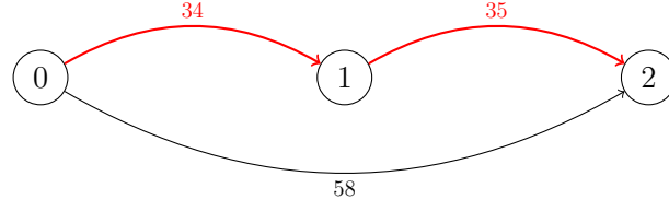
Figure 5.3: The best path at the end of period 2 with the corresponding cycle cost values.
