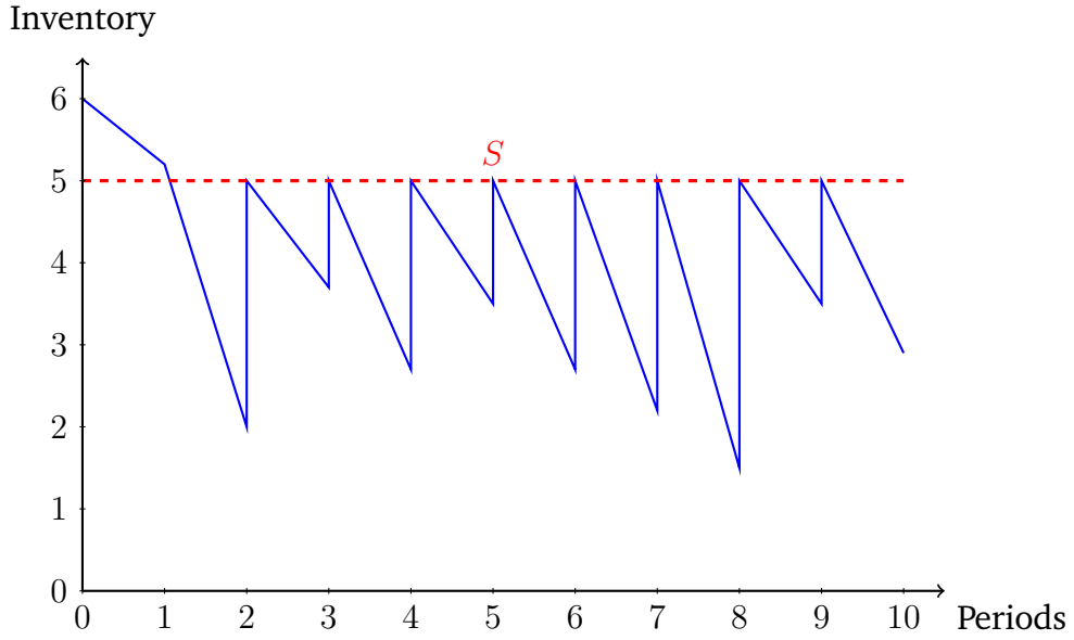
Figure 2.2: The expected inventory level under the base-stock policy
