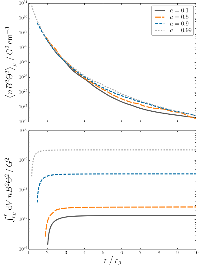
Figure 2. Time- and shell-averaged n B^2 \Theta^2 , weighted by the density. This quantity is proportional to the total synchrotron emissivity. The bottom panel shows n B^2 \Theta^2 integrated over volume with the integral taken between the horizon and r . This quantity is proportional to the total synchrotron power. It is clear that the (comoving) radiated power is dominated by the near horizon region.
