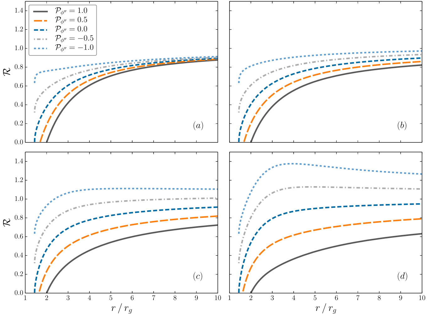
Figure 11. Redshifts for a source with a = 0.9 , and v^\phi = \epsilon v_K . We set v^\phi = 0 at the horizon, with a transition at r = r_{\text{ISCO}} . (a): \epsilon = 0.0 , (b): \epsilon = 0.2 , (c): \epsilon = 0.6 , (d): \epsilon = 1.0 .
