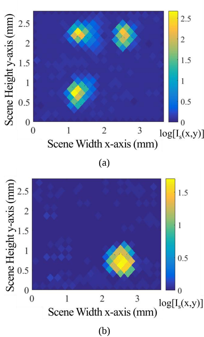
Fig. 9.3. (a) Visible scaled irradiance map obtained using the CAOS visible-NIR simultaneous dual optical band imager visible channel. (b) NIR scaled irradiance map obtained using the CAOS camera infrared channel.
