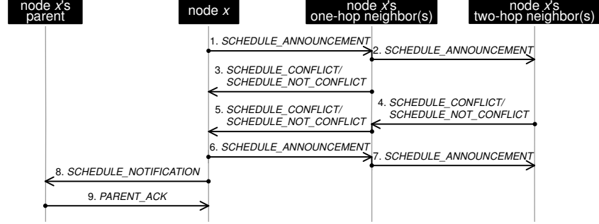
Figure 4: Message exchange in TDMA slot assignment
