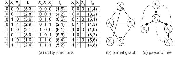
Figure 1: A MOCOP instance with 2 objectives.
