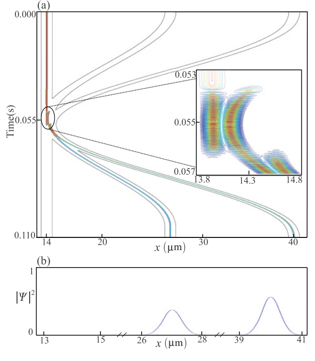
FIG. 5. (Color online) (a) Probability density for a single atom initially located in the trap on the left-hand side with respect to time for intuitive trap movement. The inset shows the tunneling area in greater detail, where Rabi oscillations between neighboring traps are clearly visible. (b) Density of the final state in each of the three traps.
