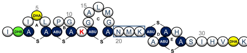
Figure 1. Structure of nisin A. The structure of nisin A is depicted, showing the location of its five (β-methyl)lanthionine rings (A–E) and modified residues dehydroalanine (yellow) and dehydrobutyrate (green). Position K12 is highlighted in red and the hinge region is boxed. doi:10.1371/journal.pone.0058530.g001
