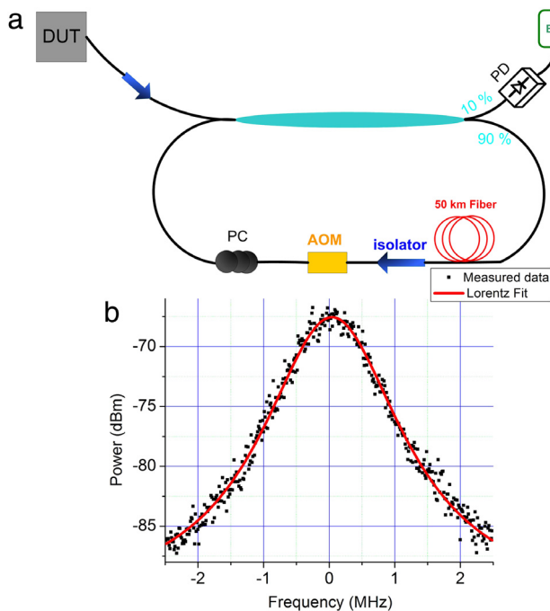
Fig. 6. (a) Re-circulating loop linewidth measurement setup (b) 500 kHz linewidth of the MZI laser.
