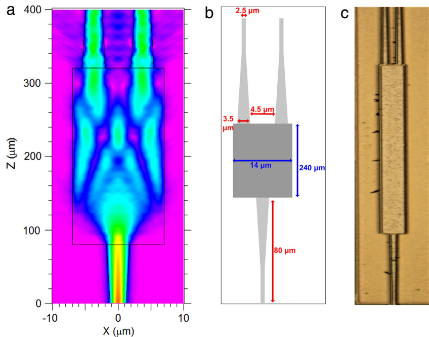
Fig. 2. (a) Simulation of the 1 × 2 MMI coupler (b) MMI dimensions (c) 1 × 2 MMI microscope image.
