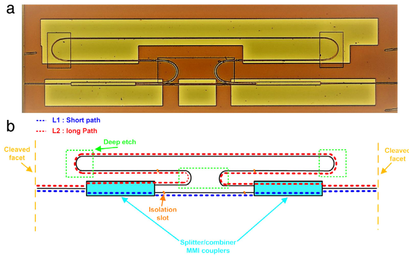
Fig. 1. (a) Microscope image of the MZI laser consisting of 2 MMI's and asymmetric arms (b) design illustration of the MZI laser cavity. (For interpretation of the references to color in this figure legend, the reader is referred to the web version of this article.)
