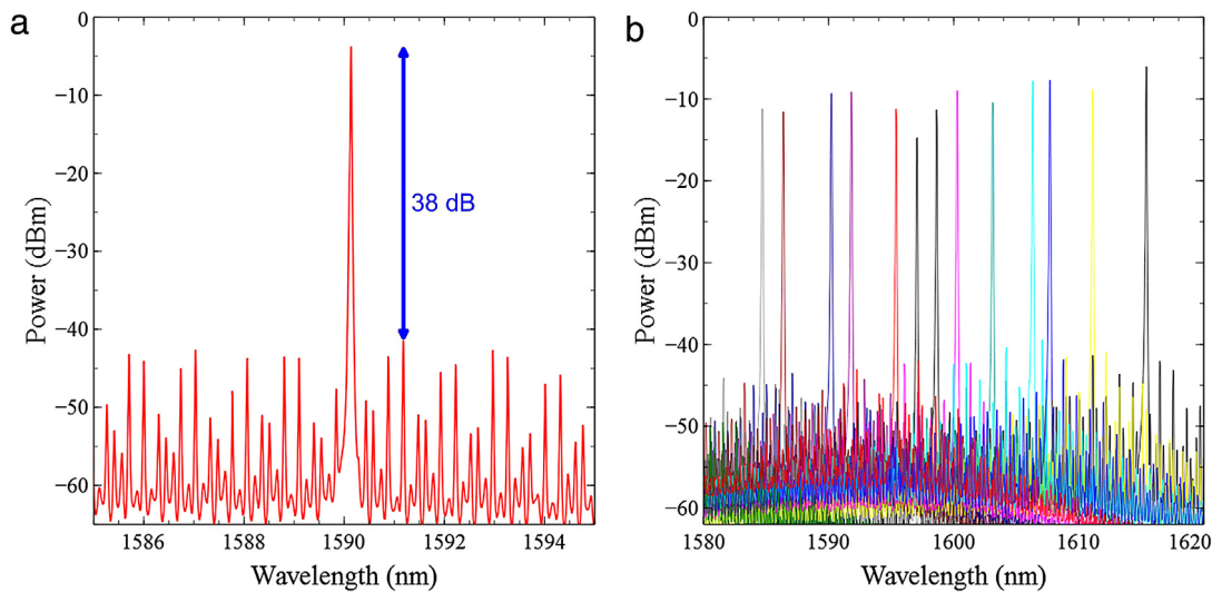
Fig. 5. (a) SMSR of 38 dB (b) tuning over 30 nm.
