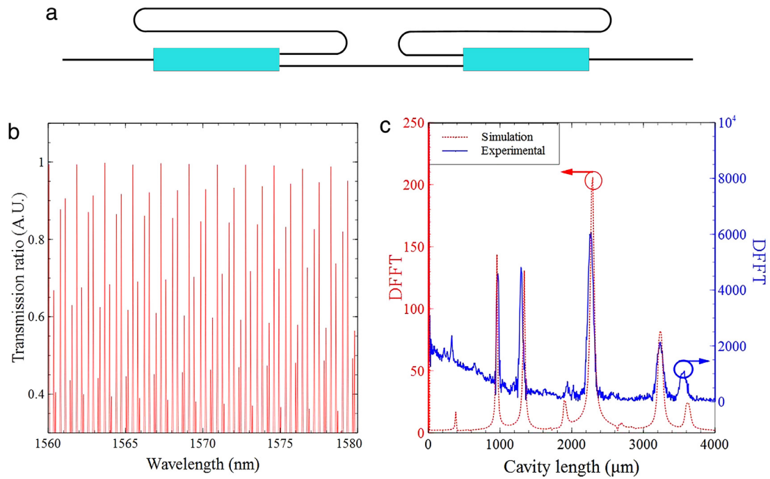
Fig. 3. (a) MZI path ways illustration (b) simulated optical transmission spectrum of the MZI cavity (c) FFT cavity analysis.
