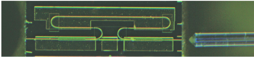
Fig. 4. Microscope image of the DUT.
