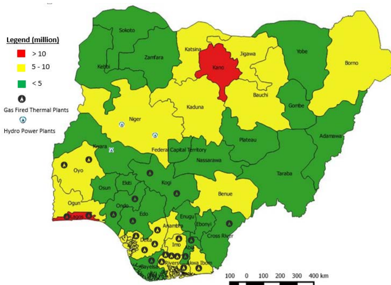
Figure 1 – Map of Nigeria showing population and power plant distribution
