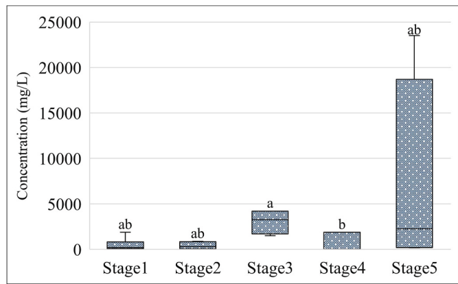
Fig. 6. Chloride ( \text{Cl}^- ) concentrations (mg/L) across the five seafood processing stages. Median, upper and lower quartiles, minimum and maximum values and outliers are shown. Different letters indicate significant differences between stages. Number of data (count) for each stage: Stage 1 = 8, Stage 2 = 6, Stage 3 = 4, Stage 4 = 6 and Stage 5 = 4.
