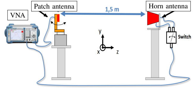
Fig. 2. Patch antenna characterization test-bench.
