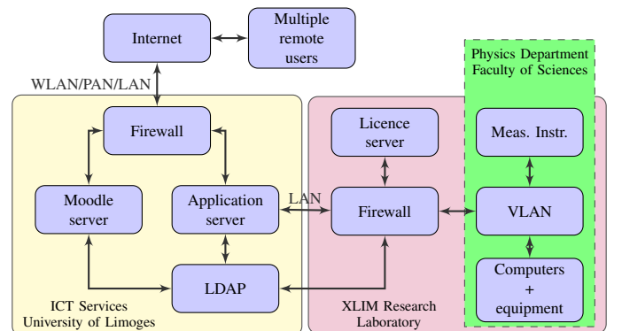
Fig. 1. University of Limoges: services and network infrastructure map.
