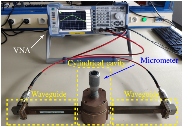
Fig. 3. Cylindrical resonant cavity test-bench.
