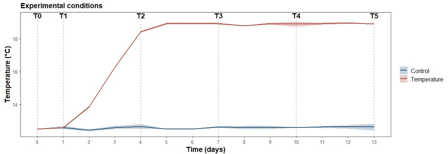
Figure S2. Mean ( \pm SD) temperature trajectory of the control and marine heatwave treatments over the course of the experiment. Grey dashed lines indicate the sampling intervals (T0–T5).
