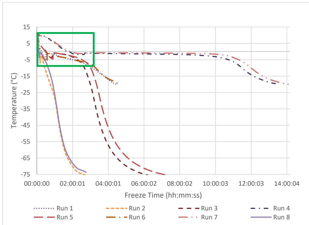
Figure 3-17: Freezing profile of FDS measured by the top probe for each DoE run
