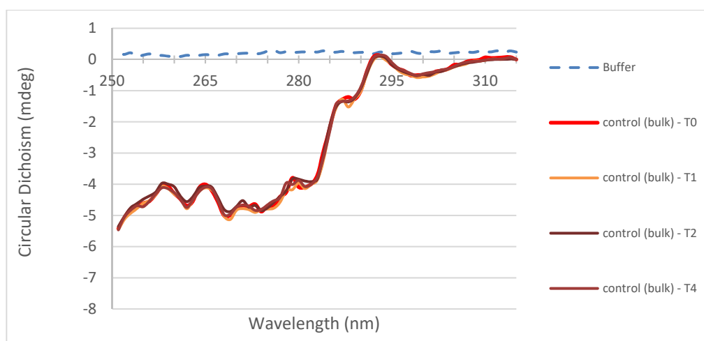
Figure 3-31: Protein Y normalised and aligned CD spectra (near-UV) of bulk control across 4-weeks storage period at 45 °C
