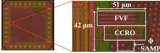
Fig. 9. Die micrograph showing zoomed-in view of the CDC.
