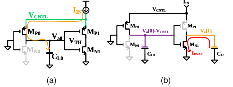
Fig. 3. Schematics illustrating (a) the effect of I_{IN} on V_{CNTL} and V_{TH} and (b) the finite cell discharge time t_{dead} .
