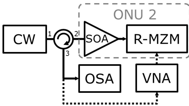
Fig. 4 Integrated ONU characterization setup (OSA: Optical Spectrum Analyzer; SOA: Semiconductor Optical Amplifier; R-MZM: Reflective Mach-Zehnder Modulator; VNA: Vector Network Analyzer).
