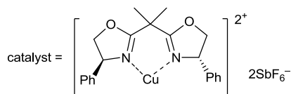
Scheme 7
