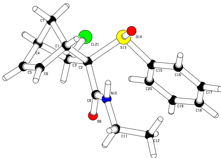
Figure 2 Crystal Structure of 4b- endo
