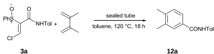
Scheme 11
