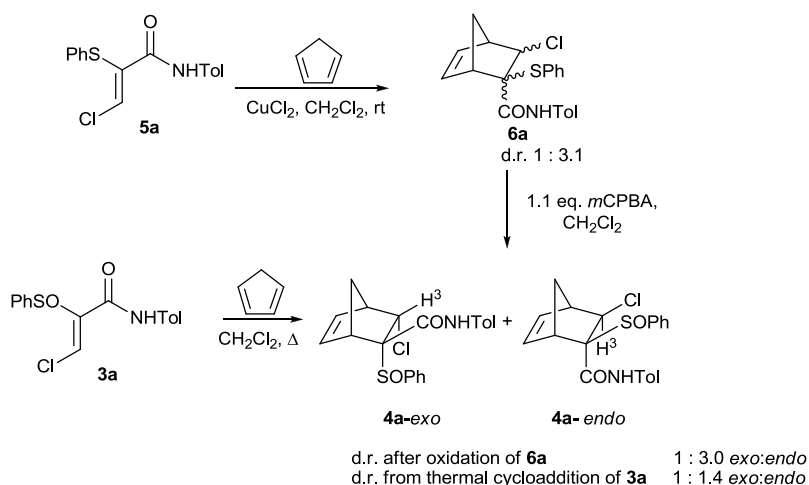
Scheme 6
