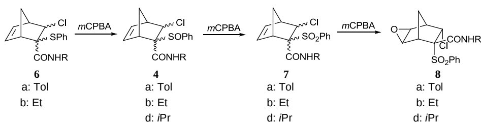
Scheme 9
