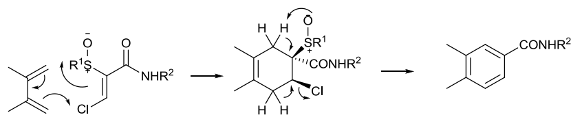
Scheme 12
