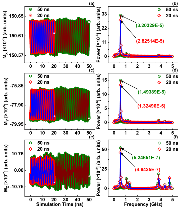
Figure 8.14: Comparison between 20 ns and 50 ns long simulation to verify the time domain stability of MMA. The calculated oscillations of the components of the magnetizations along longitudinal, transverse, and out-of-plane direction in (a), (c), and (e), respectively. The corresponding FFT spectra yield the auto-oscillation resonance peaks of the mutually synchronized MMA in (b), (d), (f), respectively [5].
