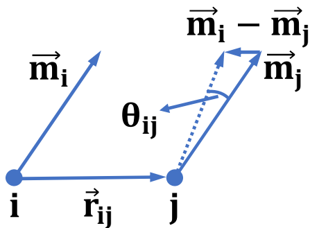
Figure 5.3: Representations of reduced moments m_i and m_j at neighbouring sites i and j separated by a vector \vec{r}_{ij} . The angles between the reduced moments, m_i , and m_j , is \theta_{ij} [2].
