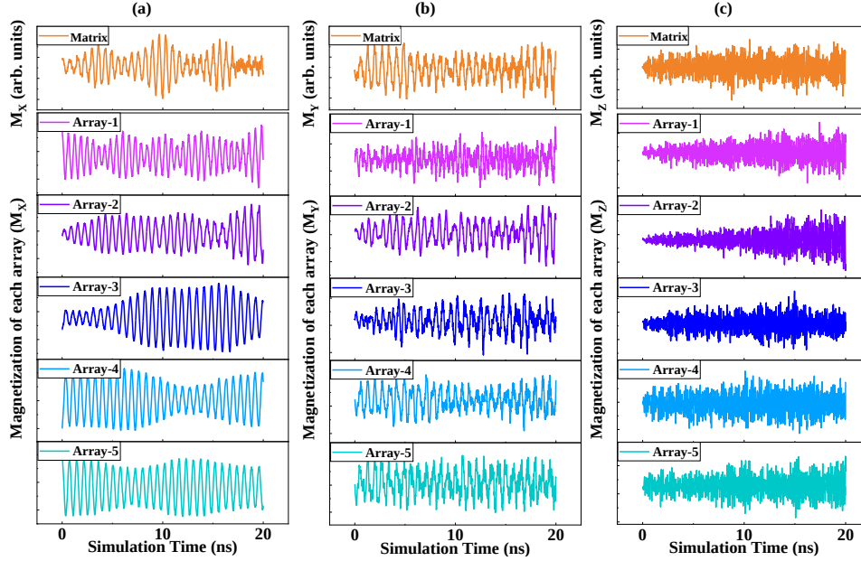
Figure 8.7: For the nanodot array, the (a) M_X , (b) M_Y and (c) M_Z components of each array, respectively while, the top row depicts the overall magnetization responses arising from the whole system [5].
