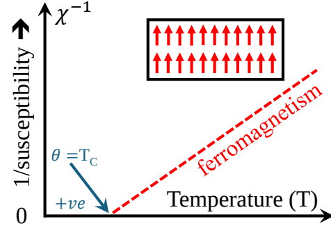
Figure 1.1: The variation of the inverse ferromagnetic susceptibility as a function of temperature, where T_C is the Curie Temperature of the material.
