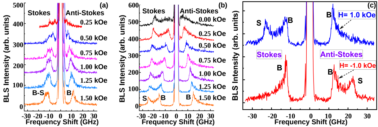
Figure 5.4: BLS Spectra of (a) non-ES (1.4 \mu\text{m} ) and (b) ES (5.7 \mu\text{m} ) CoP thin film at different in-plane bias magnetic fields measured from 1.50 kOe to 0.25 kOe [in (a)] and 0.00 kOe [in (b)] with the backscattering geometry. (c) BLS Spectra of 5.7 \mu\text{m} in a bias magnetic field of +1.0 and -1.0 kOe revealing the effect of the reversal of the magnetisation on the frequency position of the Damon-Eshbach wave [2].
