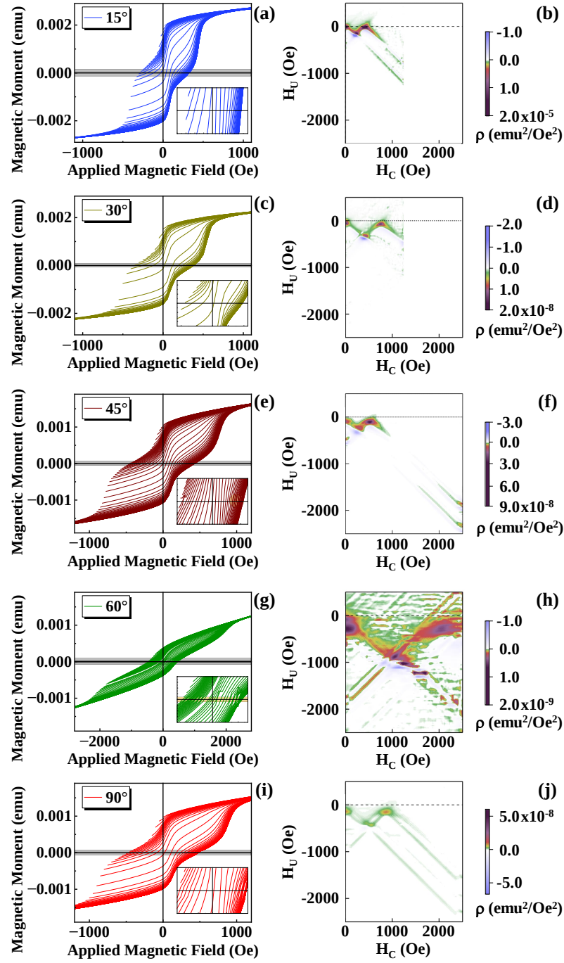
Figure 4.8: OOP angle dependent raw minor loops and its corresponding FORC distribution of 0.68 μm film indicating transverse ES nature [1].
