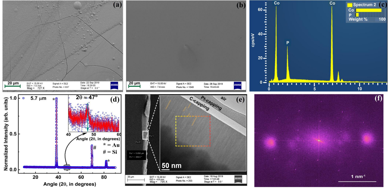
Figure 5.1: Typical SEM top surface morphology of (a) stressed thin film, (b) stress free thin film. (c) EDX spectrum of one of the samples. (d) XRD-spectrum of the sample. (e) Cross-sectional TEM micrograph of the electrodeposited CoP thin films showing the individual striations (white lines in the NHS) in (thickness 2-5 nm) nm range, typical and (f) FFT of the selected region of TEM as highlighted in (e) [2].
