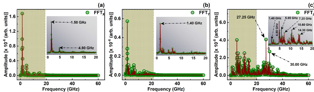
Figure 7.9: Power distribution of the patterned a matrix of nanodots in the MMA along x -, y -, z - directions in (a), (b), (c), respectively. In each of the Graph, the corresponding insets reveal the magnified frequency spectra (0 – 20 GHz range) of M_X , M_Y , M_Z of the highlighted region at left side of the parent Power-Frequency spectra (0 – 60 GHz range) [4].
