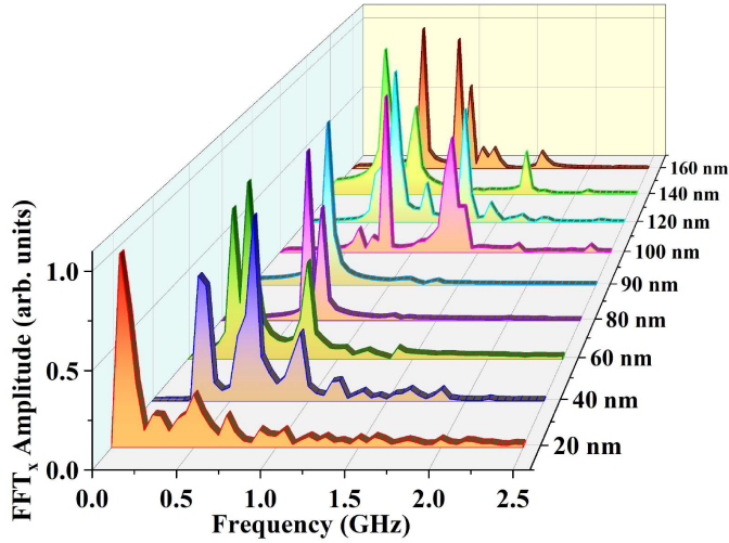
Figure 8.3: Variation of the power distribution obtained from fast Fourier Transformation (FFT) of magnetization as a function of NW spacing [5].
