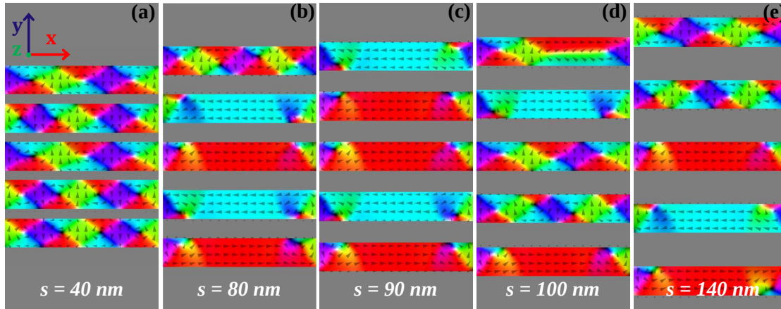
Figure 7.5: (a)-(e) Final spin configuration of the NWs after completion of 20 ns of micromagnetic simulation showing the non-volatility nature of the domains for the separation values, 40 nm, 80 nm, 90 nm, 100 nm and 140 nm, respectively [4].
