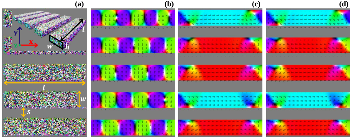
Figure 7.2: Micromagnetic modelling of NWs: (a) Initial random magnetization configuration. l , w are length, width of each of the NWs along the x , y directions, respectively, and s is the separation between the NWs along y direction of 40 nm thick NWs. (b) Multidomain state in presence of transverse stress along Y . (c) Single domain state upon launching of the SAW along X . (d) Final spin configuration after completion of 20 ns simulation confirms that the domain configurations are non-volatile in nature [4].
