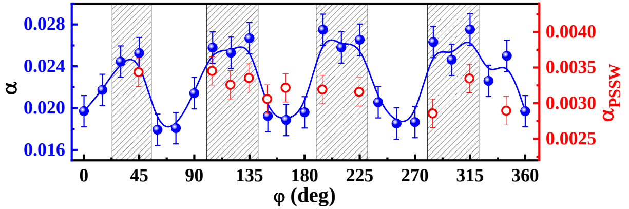
Figure 6.5: The variation of \alpha of Kittel modes (solid blue scattered points) and PSSW modes (open red scattered points) with different in-plane angles at an external bias magnetic field of 1.35 kOe with the pump fluence of 10 mJ/cm 2 . Blue solid line is guide to eye [3].
