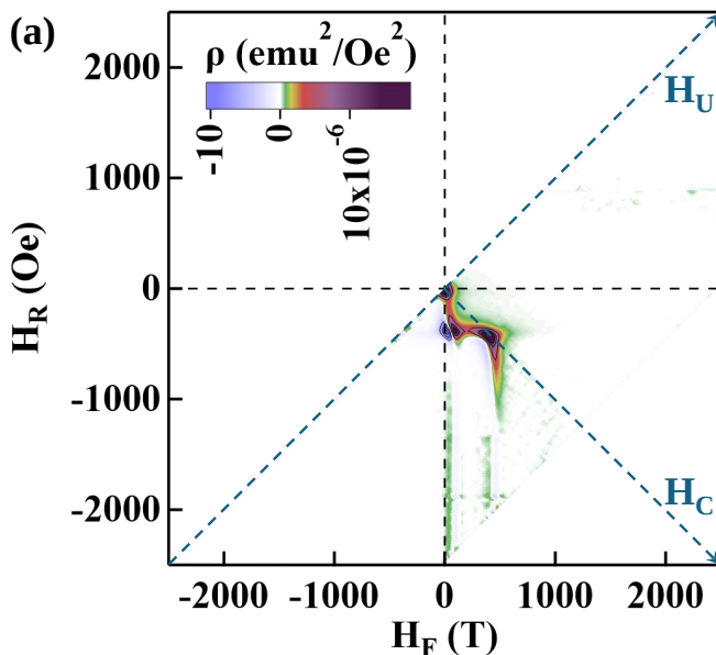
Figure 1.5: A typical example of an unrotated FORC distributions of a 0.68 \mu\text{m} cobalt based thin film alloy in (H_R, H_F) plane. During the measurement, the sample was inclined at 15^\circ out-of-plane angle with the applied magnetic field ( H ). Here, \rho is the required FORC parameter defined as a double derivative function of (H_R, H_F) , which determines the reversibility or irreversibility of the magnetic phenomena. The terms, H_C and H_U represent the local coercivity and the present bias magnetic field of the sample.
