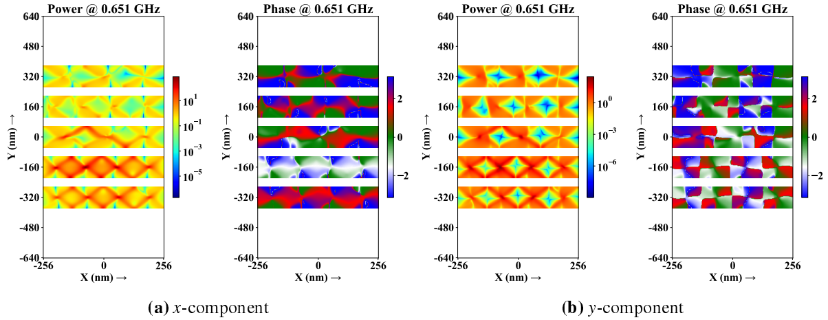
Figure 8.9: Magnon power profile and phase distribution for ‘s’=40 nm configuration showing partially synchronized state [5].
