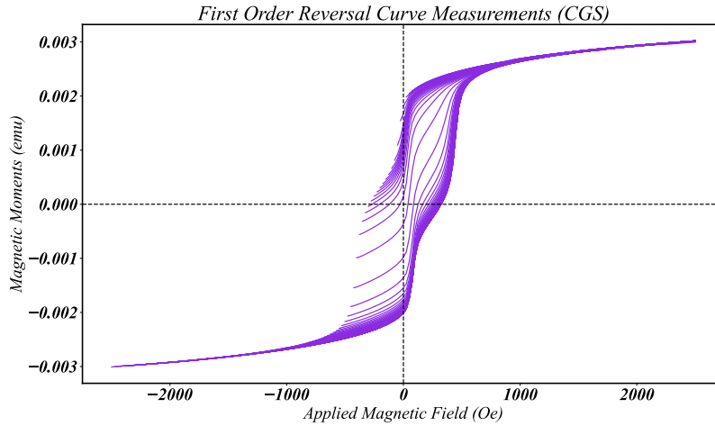
Figure 1.4: A typical example of a raw FORC distributions of a 0.68 \mu\text{m} cobalt based thin film alloy within the parent hysteresis curve revealing the series of minor/partial hysteresis loops.
