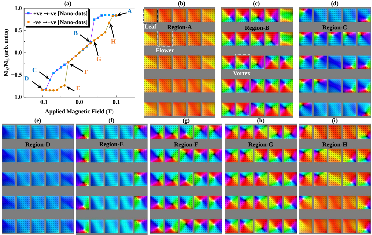
Figure 8.16: Magnified (for field range \pm 0.1 T) simulated hysteresis loop for the square nanodot matrices after applying the SAW along longitudinal ( x –) direction, where ‘A’–‘H’ signifying the different position of magnetic field which are shown in (b)–(i), respectively. ‘ Flower ’ (parallel to the longitudinal axis), ‘ Leaf ’ (domains parallel to the diagonal of the nanodots), ‘ Vortex ’ (flux closure of the magnetization) are highlighted to signify different domain states originated in the square nanodot matrix [5].
