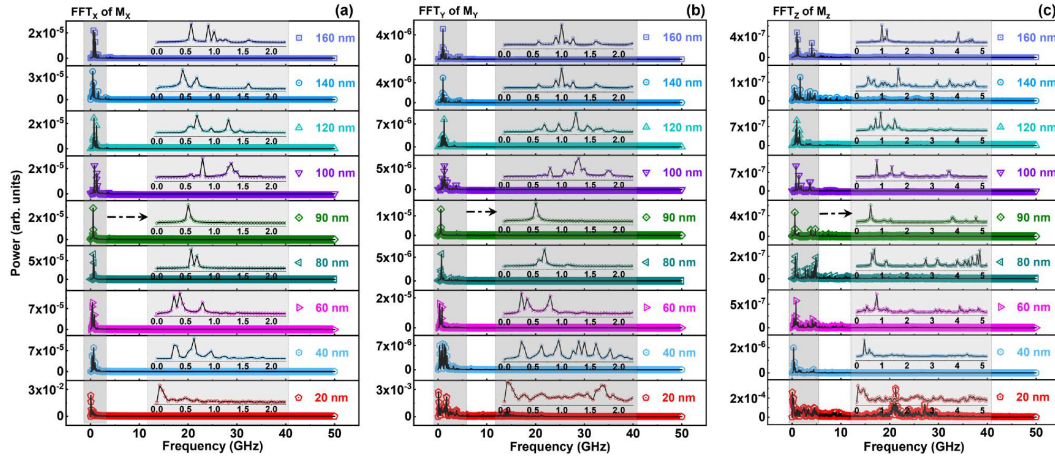
Figure 7.4: Power distribution as a function of spacing between NWs along x , y , z directions in (a), (b), (c), respectively. Corresponding insets reveal magnified frequency spectra (0-2.5(5) GHz range) of M_X & M_Y ( M_Z ) of the highlighted region at left side of the parent Power-Frequency spectra (0-50 GHz range) [4].
