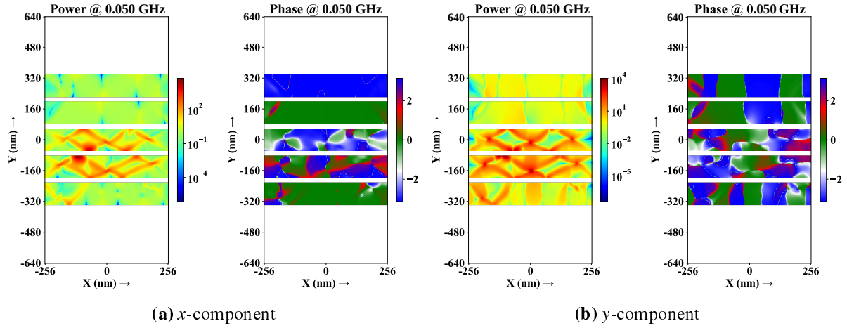
Figure 8.8: Magnon power profile and phase distribution for ‘s’=20 nm configuration showing out of synchronized state [5].
