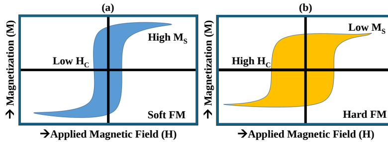
Figure 1.6: Typically, (a) soft ferromagnetic materials show low coercivity ( H_C ) and high saturation magnetization ( M_S ), while (b) hard ferromagnetic material show high coercivity ( H_C ) and low saturation magnetization ( M_S ).
