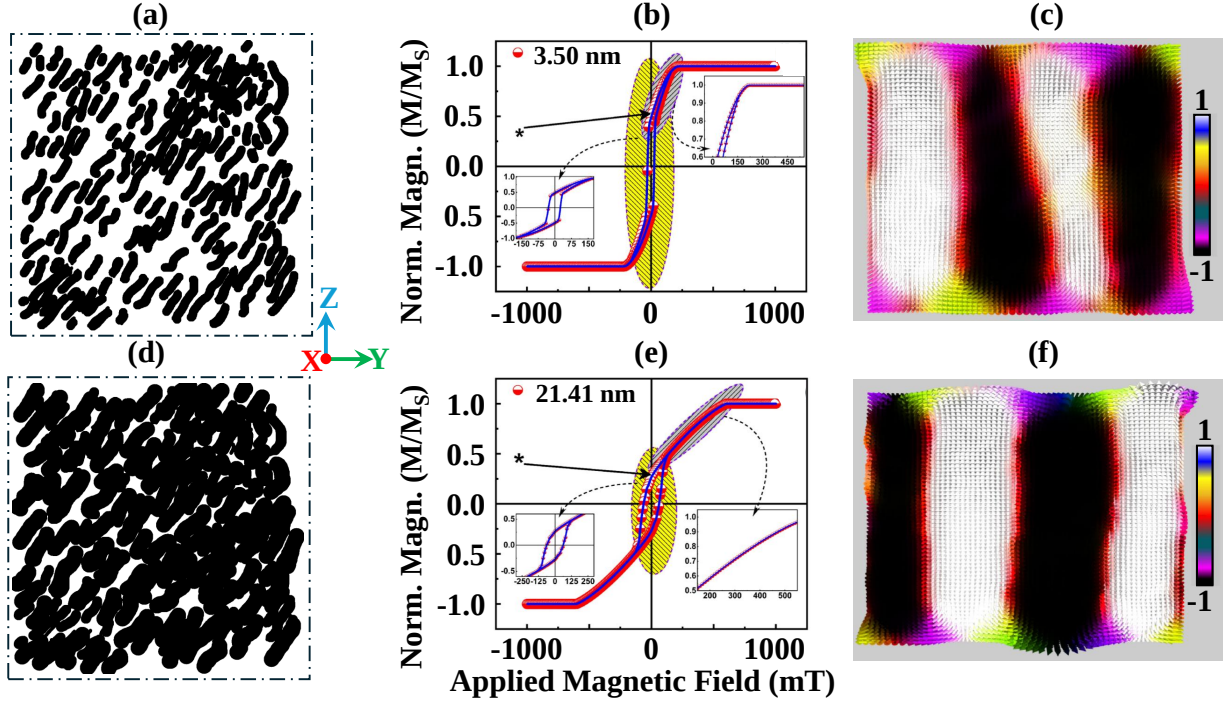
Figure 4.9: (a) An average of dispersed 3.50 nm thick NHS utilized as an input image in simulation at YZ plane. (b) Simulated three slope hysteresis loop with the complex geometry. (c) Cross-sectional macro-spin behaviour of ‘*’ marked position in the hysteresis loop. (c) thick NHS. (d) \approx 6 times dense 21.41 nm thick NHS utilized as an input image in YZ plane. (e) The simulated large hysteresis loop considering the NHS in (c). (f) the macro-spin behaviour as marked in (e) [1].
