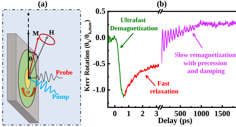
Figure 6.3: (a) Schematic of experimental geometry, sample is in x-y plane and x-z is the plane of the laser beam and (b) typical TR-MOKE data from Si/Ti (20 nm)/Au (200 nm)/CoP (3.173 \mu\text{m} ) sample at an external bias magnetic field of 1.35 kOe. The three important temporal regimes at pump fluence of 10 \text{mJ}/\text{cm}^2 are indicated in the graph [3].
