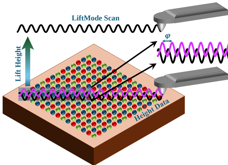
Figure 3.15: Schematic of working principle of MFM (magnetic force microscopy). Magnetic Forces cause the phase shift denoted by \phi over different domains during the 'LiftMode Scan'.
