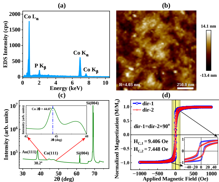
Figure 6.1: (a) Typical EDX spectrum of the sample at room temperature showing the presence of Co and P. (b) AFM image showing the surface topography. (c) X-ray diffraction pattern showing the amorphous property with nanocrystalline Co-fcc phase. (d) Typically measured in-plane hysteresis loop of one of the samples at two different in-plane directions showing anisotropic nature of the sample, here, dir.-2 = dir.-1 + 90^\circ . Inset: magnified hysteresis loop [3].
