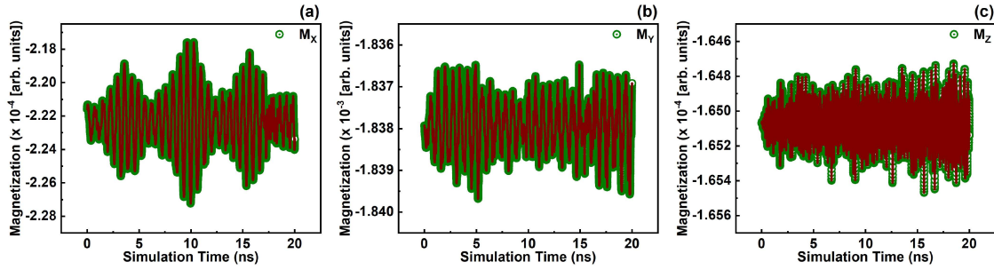
Figure 7.8: Calculated oscillations in the magnetization components, M_X , M_Y , M_Z , in a matrix of nanodots in the MMA along x -, y -, z - directions in (a), (b), (c), respectively, while the exciting SAW frequency remain kept constant at 0.5 GHz throughout the simulations [4].
