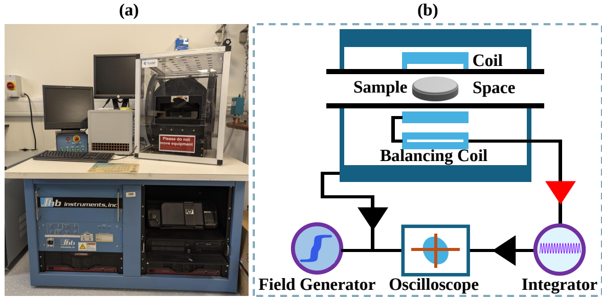
Figure 3.10: (a) Experimental setup of Mesa 200HF hysteresis loop tracer (ShB Instruments Inc.) in our laboratory (b) Schematic of hysteresis loop tracer (MESA 200 HF) by SHB Instruments Inc.
