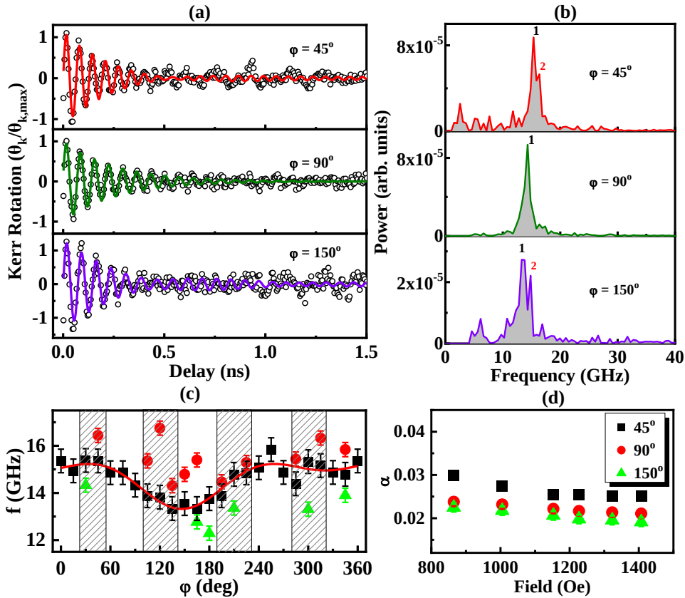
Figure 6.4: (a) Background subtracted time-resolved Kerr rotation data for external magnetic field of 1.35 kOe applied along three different in-plane angles ( 45^\circ , 90^\circ and 150^\circ , respectively w.r.t. the x axis along x-y plane) at a fixed pump fluence of 10 \text{ mJ/cm}^2 . The solid lines are fitted curves using the damped sine function. (b) FFT spectra corresponding to three different angles showing the magnetic modes. (c) In-plane angle dependent precessional frequency at the same external magnetic field of 1.35 kOe. The solid line is fitted the Kittel mode. i.e., Eq. (6.2). (d) Bias field dependent Gilbert damping constant of the Kittel mode at \varphi = 45^\circ , 90^\circ and 150^\circ reveals the suppression of extrinsic effects at higher field [3].
