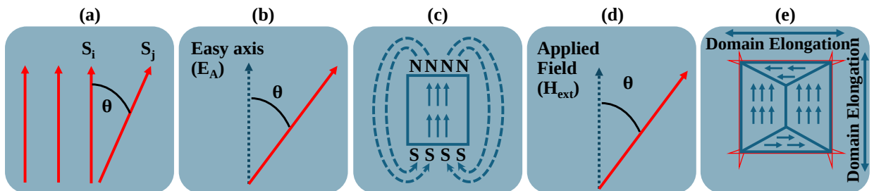
Figure 1.8: Illustration of ferromagnetic (FM) energetics to graphically explain different energies, namely (a) exchange energy, (b) anisotropy energy, (c) magnetostatic energy (d) Zeeman energy, and (e) magnetoelastic energy, respectively.
