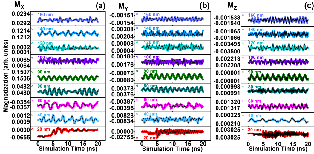
Figure 7.3: Calculated magnetization oscillations as a function of spacing between the NWs in MMA along x , y , z directions in (a), (b), (c), respectively, while the exciting SAW frequency remain kept constant at 0.5 GHz throughout the simulations [4].
