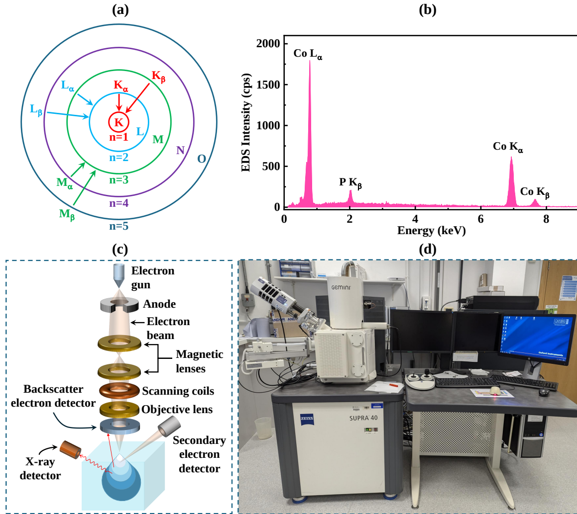
Figure 3.6: (a) Schematic showing electron transitions to lower atomic levels, illustrating the generation of K, L, and M lines. (b) A typical experimental EDX spectrum, displaying characteristic X-ray lines from various elements in the sample. (c) Schematic detailing the components of a scanning electron microscope (SEM). (d) EDX system attached to the Zeiss FE-SEM utilized for sample characterization at Tyndall National Institute.
