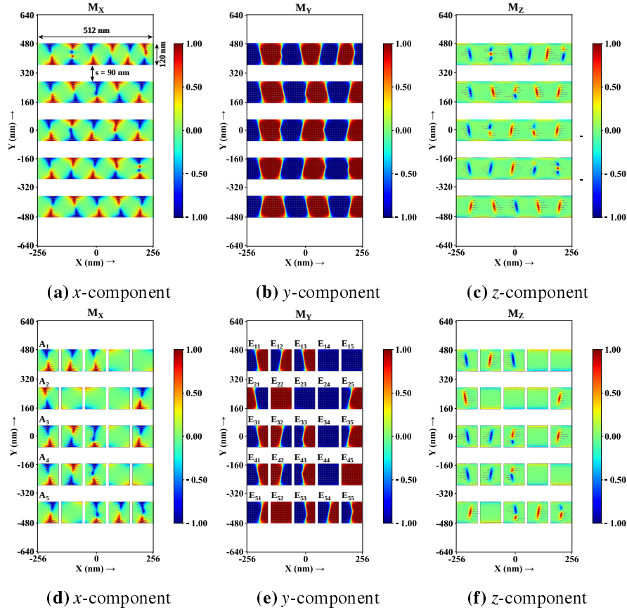
Figure 8.2: For separation, ‘s’ = 90 nm configuration, (a) x –, (b) y – and (c) z – components of the multidomain state in presence of the transverse stress along the y -direction and for nanodots that are in (d), (e) and (f), respectively. Length and width of the individual nanowires remain constant throughout the study at 512 nm and 120 nm, respectively. For the nanodots, while the separation along y -axis (vertical direction) is 90 nm that along the x -axis (horizontal direction) is 14 nm. Here, A_1 to A_5 denote the nanodot array while the E_{ij} denotes the individual nanodot elements for i^{\text{th}} row and j^{\text{th}} column, where i, j = 5 [5].
