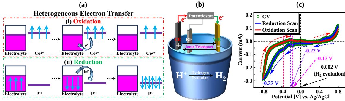
Figure 4.1: (a) Heterogeneous electron transfer: (i) oxidation of Co and (ii) reduction of P (b) The schematic of the electrochemically controlled NHS formation by hydrogen evolution. (c) A three electrode Cyclic Voltammogram curve recorded with standard Ag/AgCl electrode [1].
