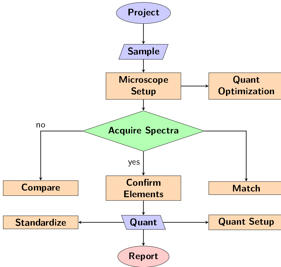
Figure 3.5: Schematic of SEM on analyser mode
