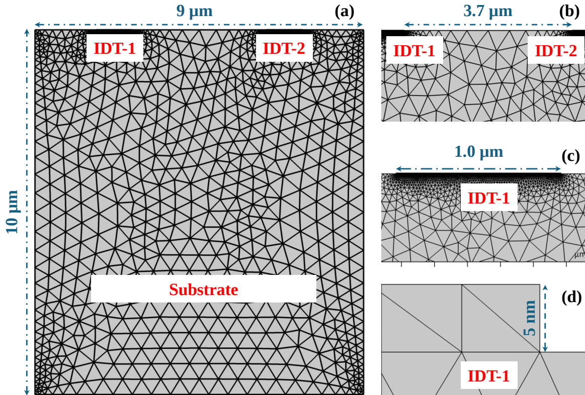
Figure 3.1: IDTs made with Aluminium (Al) on Substrate in COMSOL Geometry design with Mesh for generating SAW to operate MMA. (a) Required 10 \mu\text{m} thick \text{LiNbO}_3 substrate with width 9 \mu\text{m} having IDT structure on it. (b) Magnified region of (a) illustrates the separation between two IDTs. Both the IDTs have similar structure having width 1 \mu\text{m} and thickness 5 nm as exhibited in (c) and (d), respectively.
