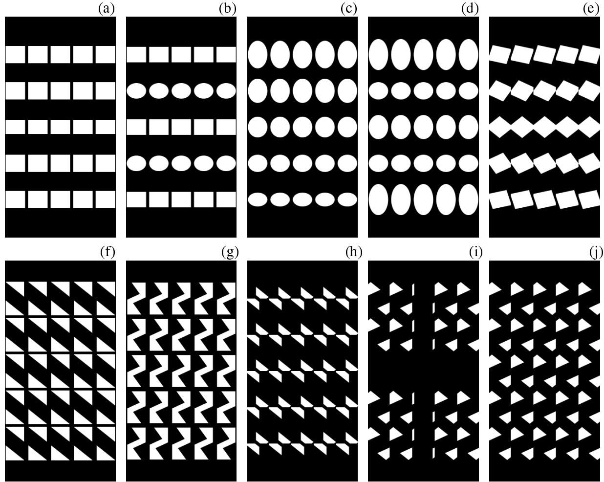
Figure 10.1: Several proposed design of nanostructured MMA to incorporate further nonlinearity in magnon power-phase distribution, which would eventually make the MMA compatible for reservoir computing.
