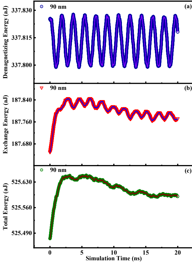
Figure 8.5: Variation of the (a) De-magnetization Energy, (b) Exchange Energy, (c) Total Energy, as a function of simulation time of the MMA at 90 nm separation ensuring efficient coupling for the auto-oscillation and mutually synchronized state of the NWs [5].
