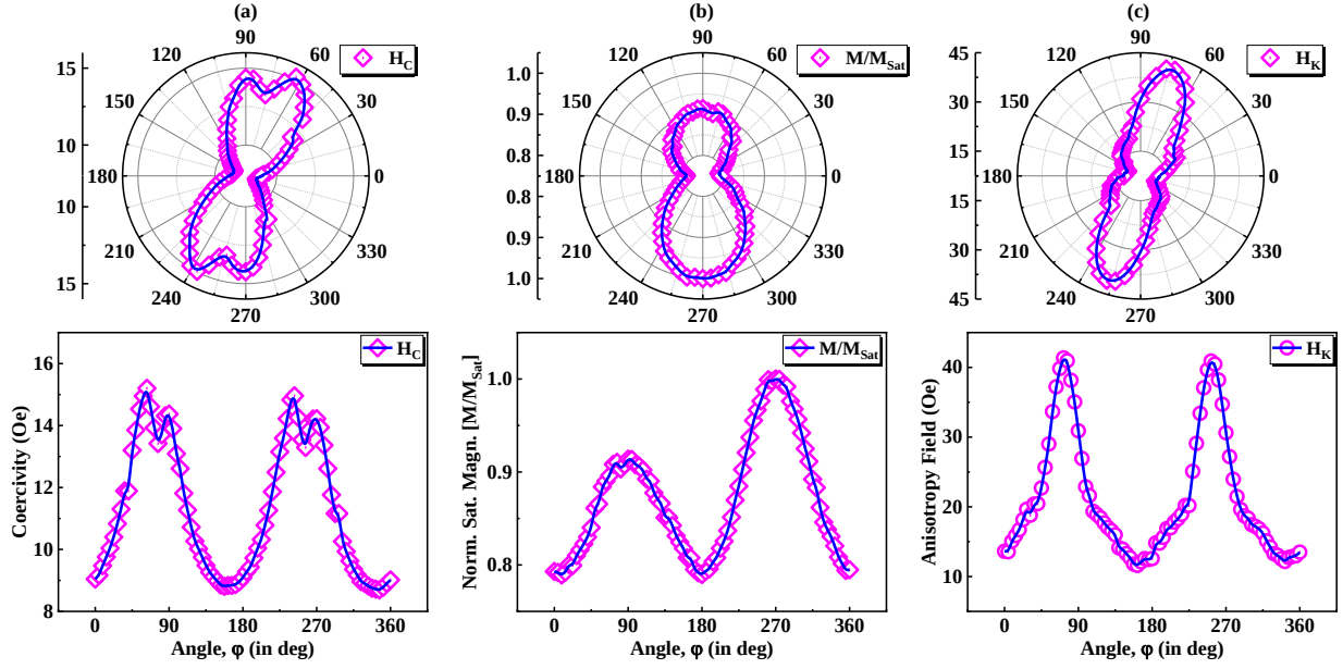
Figure 6.2: The variation of the (a) coercive field ( H_C ), (b) saturation magnetization ( M_{Sat} ) and (c) anisotropy field ( H_K ) of the material as a function of angle (in degrees). The top row exhibits the polar plot of the corresponding parameters [3].
