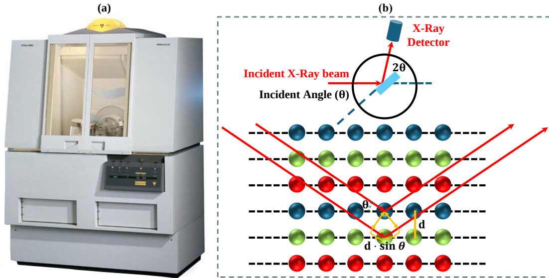
Figure 3.7: (a) Experimental setup of a PANalytical X'Pert Pro MPD X-ray diffractometer (XRD) in our lab at Tyndall National Institute. (b) Bragg's Law: Schematic illustration of the working principle of the XRD method.
