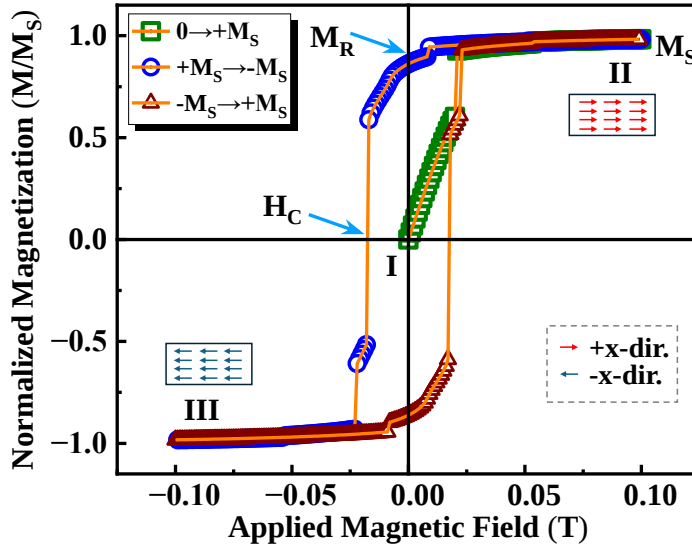
Figure 1.2: Simulated hysteresis loop of a typical ferromagnetic material. Here, H_C , \pm M_S , and M_R are the coercivity, positive/negative saturation magnetization, and remanence of the ferromagnetic material, respectively. The domains with the red and right arrows dictate +x direction domains while that in blue and left arrows highlight the -x direction domains.
