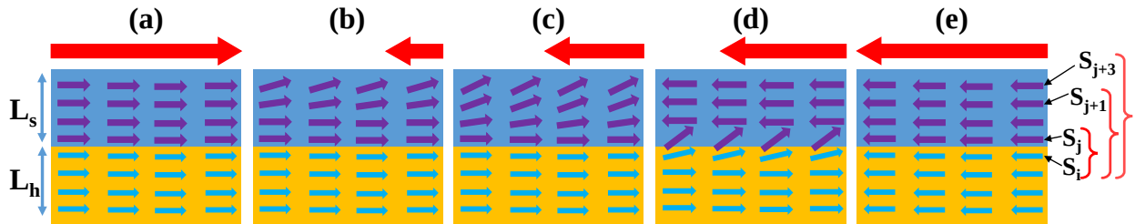
Figure 2.1: (a) Enough magnetic field applied to saturate the magnet (b) Demagnetization process starts when the magnetic field is applied in the reverse direction. (c)-(d) Demagnetization steps (e) Demagnetization complete. Here, the violet arrows denotes the magnetic moment for soft phase while that in the blue colour highlights the magnetic moments for hard phase. The rightward red arrow on top of the figure signifies that the magnetic field applied in the forward direction while that in the leftward direction indicates that the field is applied in the reverse direction.
