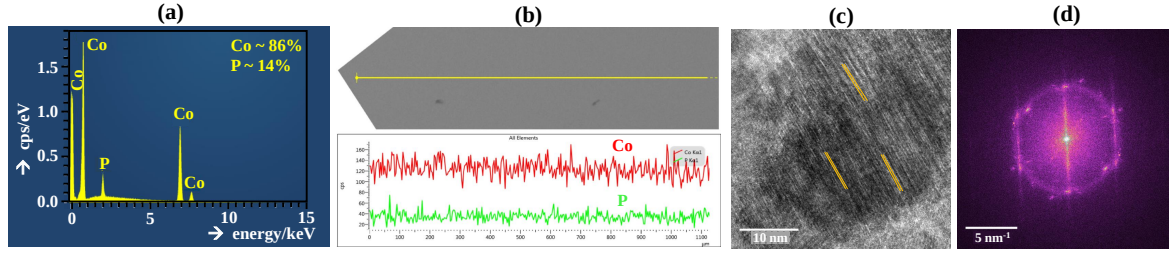
Figure 4.2: (a) Typical EDX spectrum showing the presence of Co and P in the films. (b) Top: EDX linescan path on the surface (yellow line). Bottom: Red curve denotes linescan for Co , and green curve for P . (c) A cross-sectional HR-TEM image of the film showing the striations in nm range formed due to stress caused by H -evolution. (d) FFT of the TEM image (c) confirms crystalline phases ( Co – hcp ) present in the amorphous CoP matrix [1].
