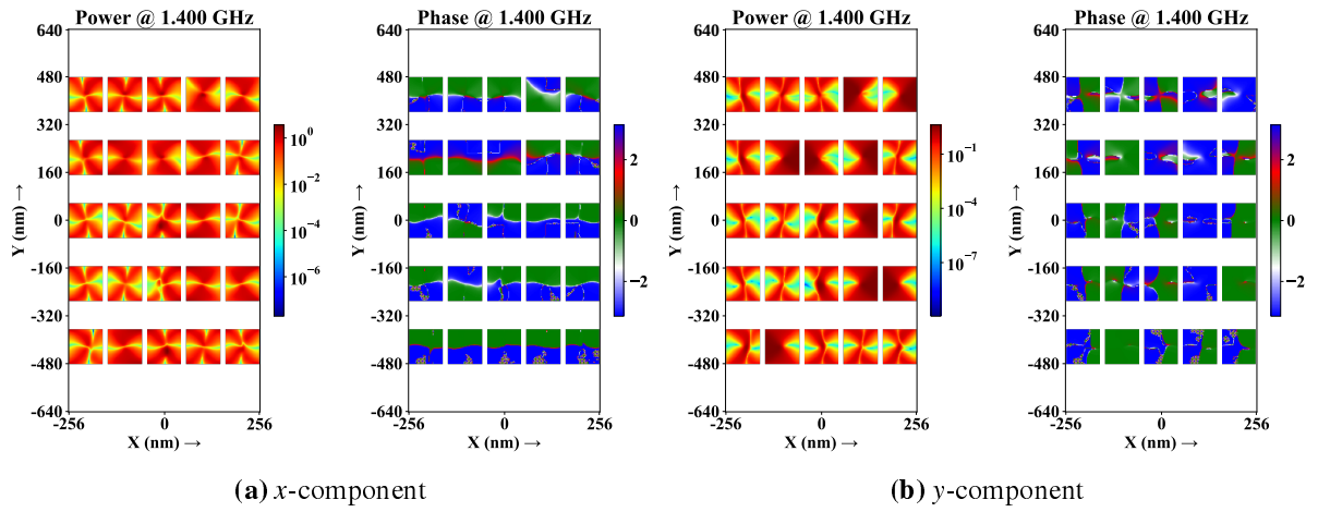
Figure 8.11: Magnon power profiles and phase distribution for the array configuration showing complex synchronization state within the nanoelements of the matrix.
