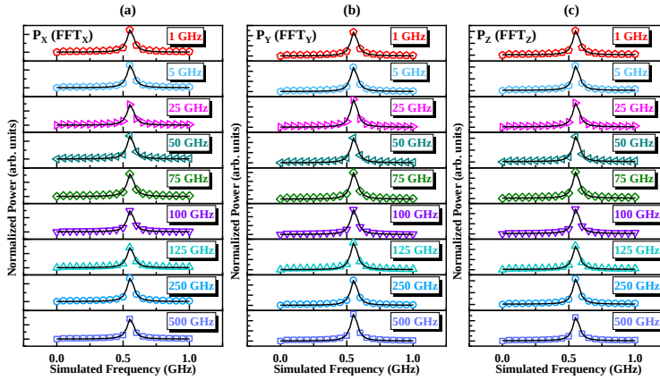
Figure 8.13: Power distribution of the frequency locked states as a function of frequency along x –, y –, z – directions, respectively [5].
