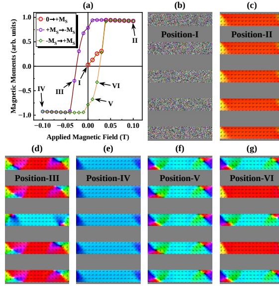
Figure 1.3: (a) Simulated hysteresis loop of a magnetostrictive FeGa nanowire (NW) array. Here, ‘I’—‘VI’ denote different values of magnetic field of the hysteresis loop. The dimension of each of the nanowires is 512 \times 120 \times 40 \text{ nm}^3 while the constituent NWs are separated at a distance of 160 nm. Each of the domain configurations of the position ‘I’—‘VI’ is given in (b)-(g), respectively.
