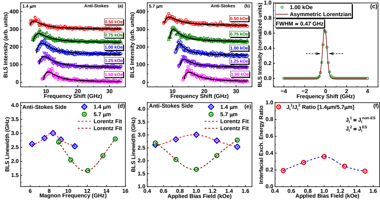
Figure 5.6: Lorentzian fittings of the anti-Stokes BLS peak as a function of magnetic field of (a) 1.4 \mu\text{m} non-ES and (b) 5.7 \mu\text{m} ES CoP thin film. (c) Lorentzian fitting to a typical elastic peak in the BLS spectra. BLS linewidth ( \Delta f ) as a function of (d) corresponding anti-Stokes magnon frequencies and. (e) applied bias magnetic field for 1.4 \mu\text{m} and 5.7 \mu\text{m} thick thin films. (f) The J_1^1/J_1^2 ratio as function of bias magnetic field. The symbols correspond to the experimental data while the lines joining the symbols are guide to eyes [2].
