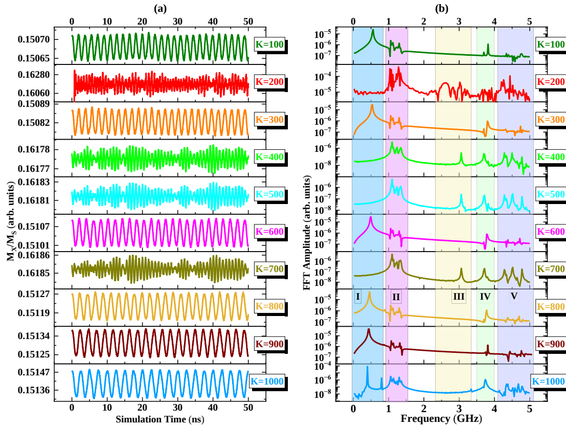
Figure 8.18: Variation of (a) magnetization oscillation and (b) its corresponding frequency as a function of applied stress [5].
