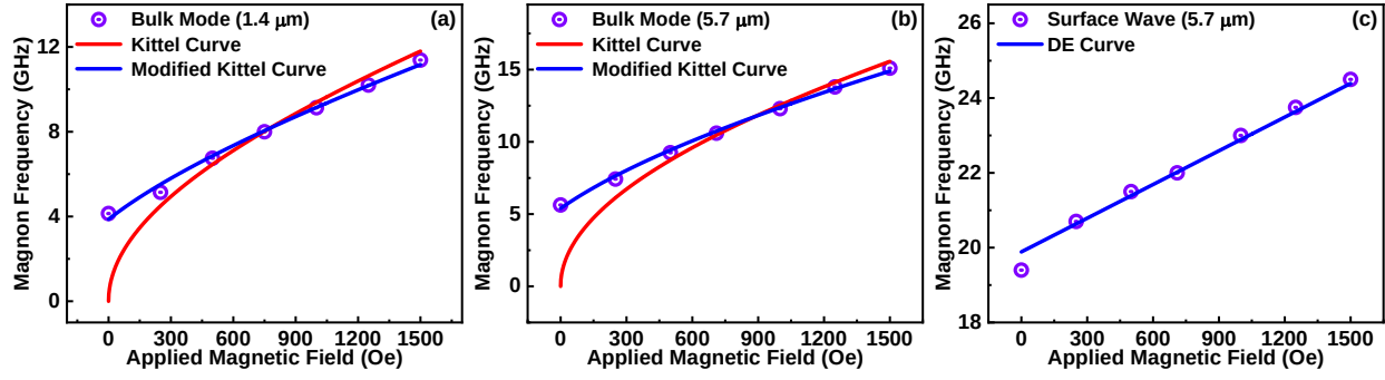
Figure 5.5: Spin wave frequencies of (a) bulk mode (1.4 \mu\text{m} non-ES film), (b) bulk mode of ES and (c) Damon-Eshbach surface wave as a function of magnetic field of 5.7 \mu\text{m} ES CoP thin film [2].
