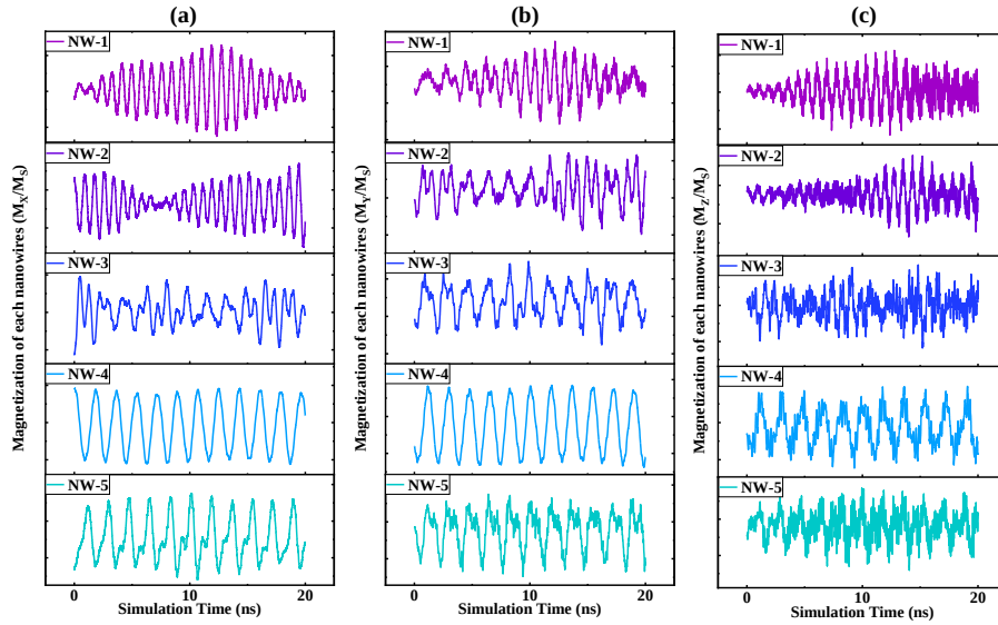
Figure 8.6: The (a) M_X , (b) M_Y and (c) M_Z components of each nanowire for 90 nm configuration, respectively while, the top row highlights the overall magnetization of the whole system [5].
