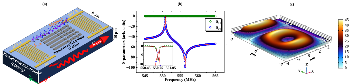
Figure 8.1: (a) 3D schematic of the magnon microwave antenna (MMA) with magnetostrictive (FeGa) nanowires (NWs). k_{\text{SAW}} and k_{\text{SW}} are the wave vectors associated with the SAW and the SW, respectively. Here, the width and thickness of the piezoelectric substrate ( \text{LiNbO}_3 ) are 9 \mu\text{m} and 10 \mu\text{m} and that of the interdigitated transducer electrodes [IDT-1 and IDT-2 in the schematic] of Al (stands for Aluminum) are 1 \mu\text{m} and thickness 100 nm, respectively. (b) S_{11} and S_{21} parameters confirm the resonance frequency of SAW at 550.75 MHz. (c) Deformed shape plot at the resonance SAW mode estimates the penetration depth of 45 nm [5].
