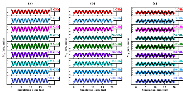
Figure 8.12: Magnetization dynamics along x -, y -, z - directions as a function of SAW frequency altered from 1 GHz to 500 GHz with included with 0.5 GHz parent frequency. The inter-distance between the neighbouring five NWs remain constant at 90 nm to ensure sufficient exchange coupling and the dipolar interaction [5].
