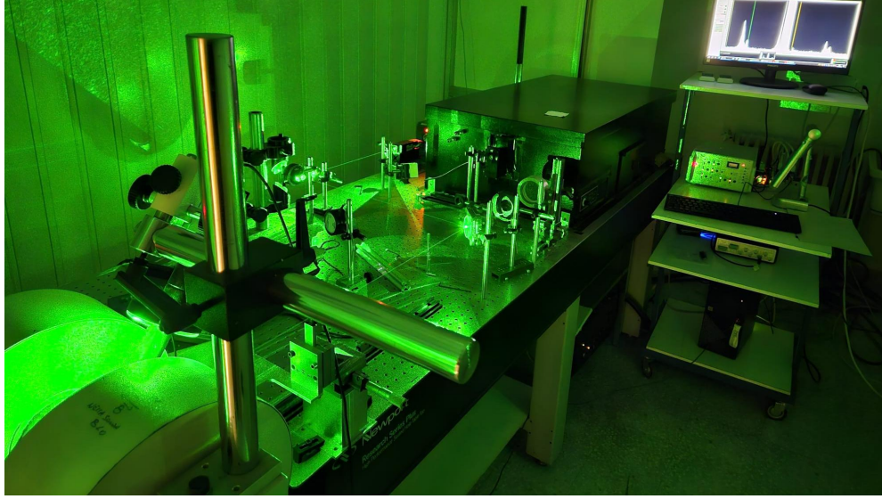
Figure 3.16: Experimental setup of the Brillouin Light Scattering (BLS) setup in the GHOST laboratory at CNR-IOM, Perugia, Italy.
