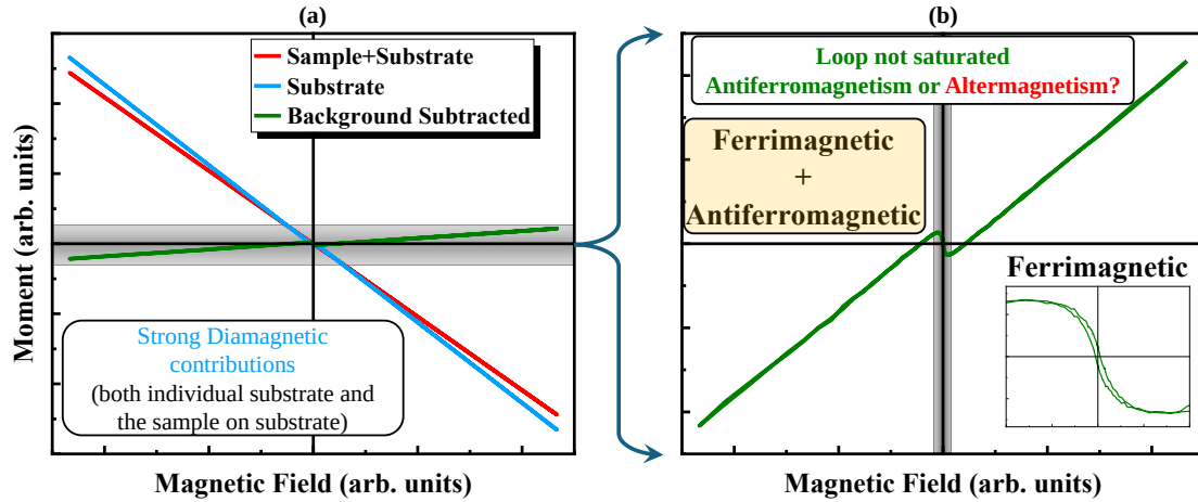
Figure 3.14: (a) At room temperature, different hysteresis loops of a thin magnetic material grown on a diamagnetic substrate. (b) Magnified version (obtained after subtracting the substrate contribution) shows the real/actual magnetic behaviour of deposited magnetic material.
