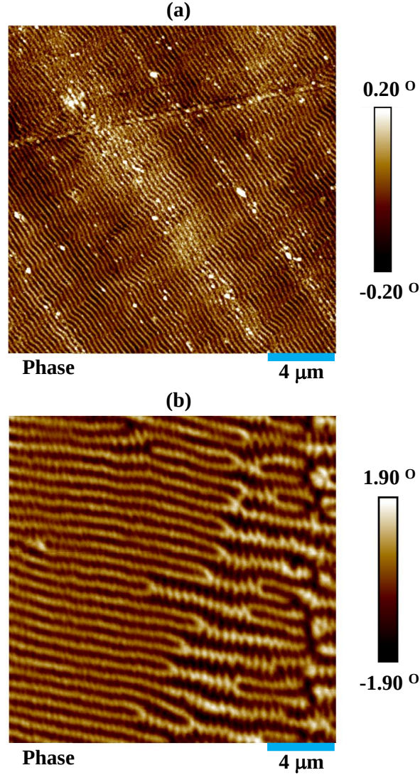
Figure 4.4: (a) Typical stripe domain structure in low current ( \sim 5.5 \text{ mA/cm}^2 ) sample (thickness 0.31 \mu\text{m} ). (b) Modified domains featuring corrugated stripes with domain branching in comparatively higher current \sim 137 \text{ mA/cm}^2 sample (thickness \sim 5 \mu\text{m} ). Both the scale bars are 4 \mu\text{m} and right side is the image colour scale [1].
