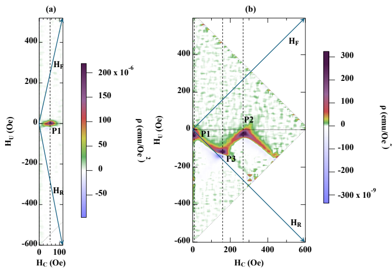
Figure 4.6: IP FORC measurement of (a) 0.31\ \mu\text{m} and (b) 0.68\ \mu\text{m} films in (H_C, H_U) plane [1].
