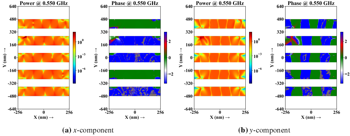
Figure 8.10: Magnon power profile and phase distribution for ‘s’ = 90 nm showing the synchronized state with uniform distribution [5].
