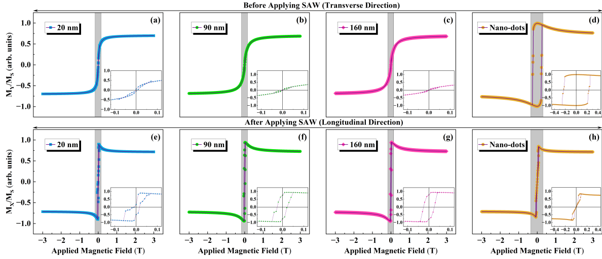
Figure 8.15: Simulated hysteresis loops of 20 nm, 90 nm, 160 nm separated NWs (a)-(c) and the nanodots (d) before applying the SAW along transverse (y-) direction, while the same for the same configurations, (e)-(h) after the application of the SAW along longitudinal (x-) direction [5].
