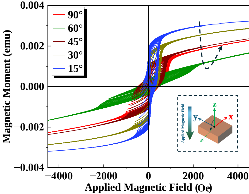
Figure 4.7: OOP Angle dependent raw FORC curves of 0.68 \mu\text{m} film. The inset shows the schematic of the sample and applied magnetic field orientation reveals that the OOP angle is varying along the z -direction while the applied magnetic field direction is fixed along the perpendicular direction [1].
