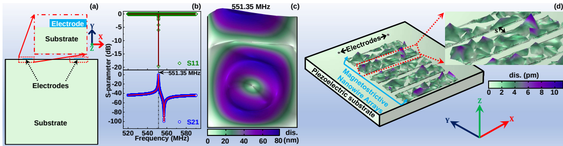
Figure 7.1: COMSOL design of the magnon microwave antenna with magnetostrictive nanowires: (a) 2D cross-sectional model in COMSOL to calculate the generated SAW frequency. Substrate width 9 \mu\text{m} , thickness 10 \mu\text{m} ; Aluminium (Al) electrodes (the magnified version of the highlighted region) width 1 \mu\text{m} and thickness 5 \text{ nm} . (b) S_{11} and S_{21} parameters confirm the surface acoustic wave (SAW) resonance frequency at 551.35 MHz. (c) Deformed shape plot of the resonance SAW mode confirms the maximum penetration depth of the SAW. (d) The magnetostriction effect in nanowires shows some mechanical displacement of NWs caused by the SAW [4].
