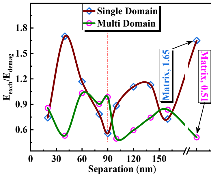
Figure 8.4: Variation of the exchange energy ratio to the demagnetizing energy as a function of spacing between the NWs for the single domain state and multidomain state, respectively. The same for the nanodot matrix is annotated on the graph [5].
