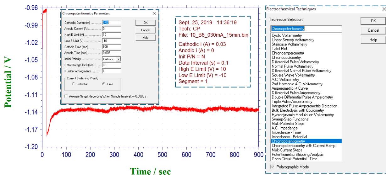
Figure 3.3: The software interface of CHI 660B potentiostat displaying different options: The right panel reveals all the possible available “Electrochemical Techniques” which could be performed with the CHI 660B potentiostat. Out of all those options, the “Chronopotentiometry” is highlighted as it was one of the selected techniques to utilize during one of the thin film fabrications. The left inset describes different “Chronopotentiometry Parameters” to perform the electrodeposition. The middle one is the confirmation panel after completing the electrodeposition.
