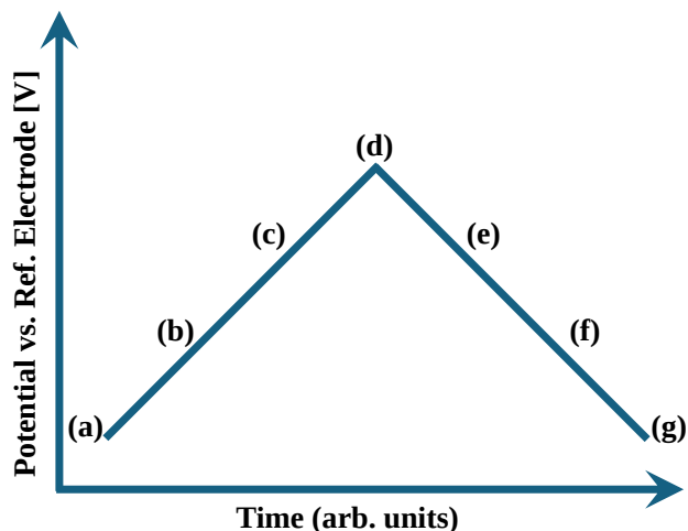
Figure 3.4: Schematic representation of the CV excitation signal.
