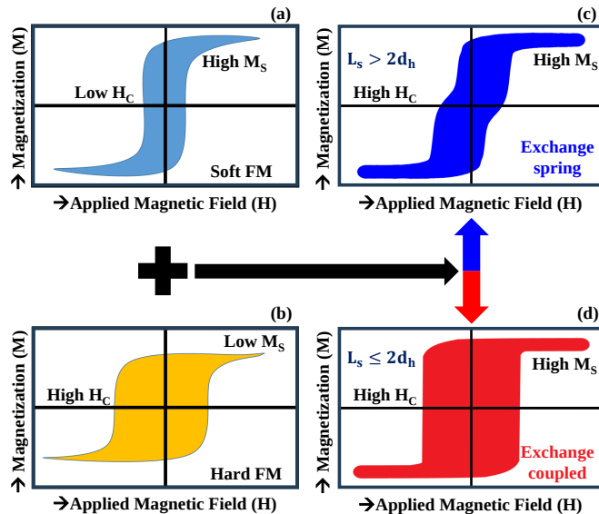
Figure 1.7: Schematic of hysteresis loops of nanostructured soft and hard magnets are in (a) and (b), respectively. Formation of magnetic nano-hetero-structures, namely (c) exchange spring and (d) exchange coupled nanomagnets depending upon the critical conditions.
