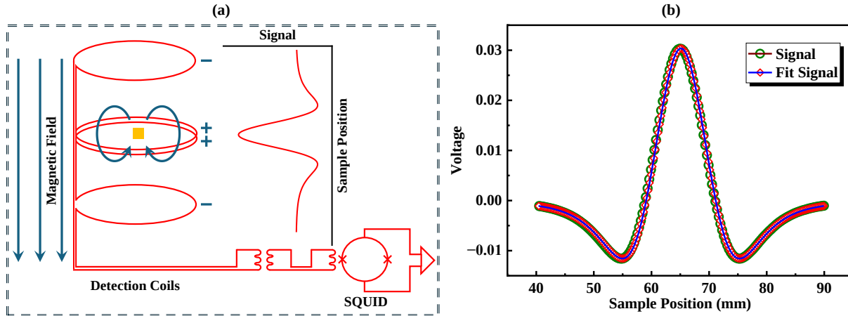
Figure 3.13: (a) Schematic of SQUID detection. (b) Sample offset value in mm to keep the sample holder in the center position.
