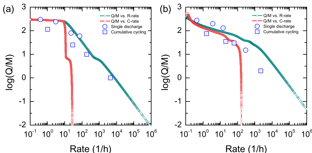
Figure 10. Q/M plots for o-IO and c-IO \text{V}_2\text{O}_5 Li battery electrodes in a flooded cell after potential step to the lower cut-off voltage of 1.2 V ( \text{Li}^+/\text{Li} ) as a function of C-rate and R-rate. Specific capacity values extracted from galvanostatic discharge curves of o-IO and c-IO electrodes (e.g. refer to Figs. 3 and 6) are independently (not fitted) overlaid on the Q/M plots. Two different measurements of specific capacity data for o-IO and c-IO \text{V}_2\text{O}_5 electrodes are shown: (1) fresh un lithiated electrodes each discharged at 0.5 C, 5 C, 10 C, and 30 C (1st discharge). (2) A single o-IO or c-IO electrodes that underwent 25 cycles at each of the four C-rates. The plots were also fitted using Eqs. 3 and 4.
