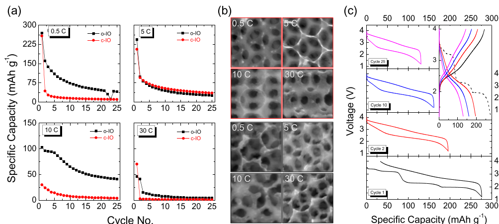
Figure 7. (a) Specific capacity from initial lithiation vs cycle number of o-IO and c-IO V 2 O 5 electrodes in flooded 3-electrode Li battery cells at rates of 0.5, 5, 10 and 30 C. (b) Corresponding SEM images of the c-IO (red outline) and o-IO (black outline) morphology after 25 cycles. (c) Charge-discharge cycles (25 cycles) showing the voltage fade, cycle hysteresis, capacity fade for an o-IO electrode cycles at 0.5 C. No constant potential charging was applied to this cathode after the first galvanostatic charge.
