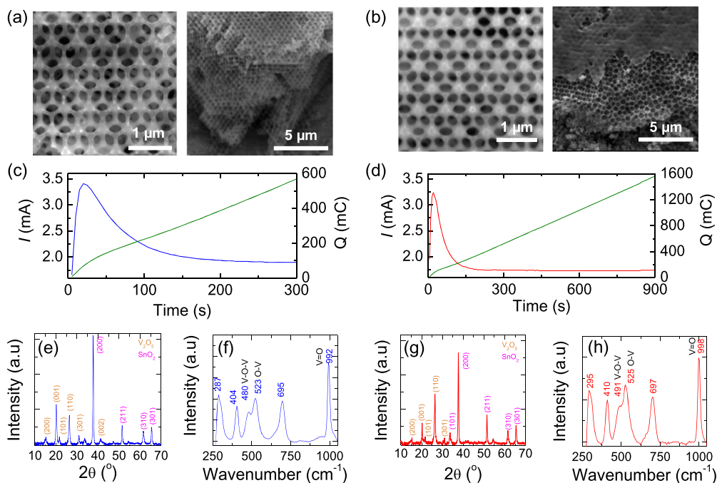
Figure 2. (a) SEM images of \text{V}_2\text{O}_5 IO grown by electrodeposition at a potential of 2 V (vs SCE) for 300 s and (b) for 900 s. Tilted images confirm IO formation throughout the original opal template and the overlayer characteristic of longer growth times. We refer to these as open IO (o-IO) and closed IO (c-IO). (c) Corresponding potentiostatic I(t) chronoamperograms for growth of \text{V}_2\text{O}_5 IO for 300 s and (d) 900 s. The cumulative charge passed, Q , is overlaid. (e), (g) XRD patterns of \text{V}_2\text{O}_5 indexed to PDF 41-1426. Reflections from the underlying FTO substrate (PDF 46-1088) are marked. (f), (h) Raman scattering spectra for IO deposits following growth for 300 s and 900 s respectively.
