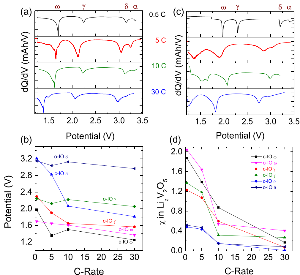
Figure 4. Differential charge curve for (a) o-IO formed by ED for 300 s and (c) for the c-IO grown over 900 s, from the first galvanostatic discharge at each C-rate. The corresponding \text{Li}_\chi\text{V}_2\text{O}_5 phases are indicated. (b) Potential (V) vs C-rate of each \text{Li}_\chi\text{V}_2\text{O}_5 phase for \text{V}_2\text{O}_5 o-IO and c-IO structures. (d) Lithium mole fraction ( \chi ) vs C-rate for both open (o-IO) and closed-top (c-IO) \text{V}_2\text{O}_5 IO structures from the first discharge.
