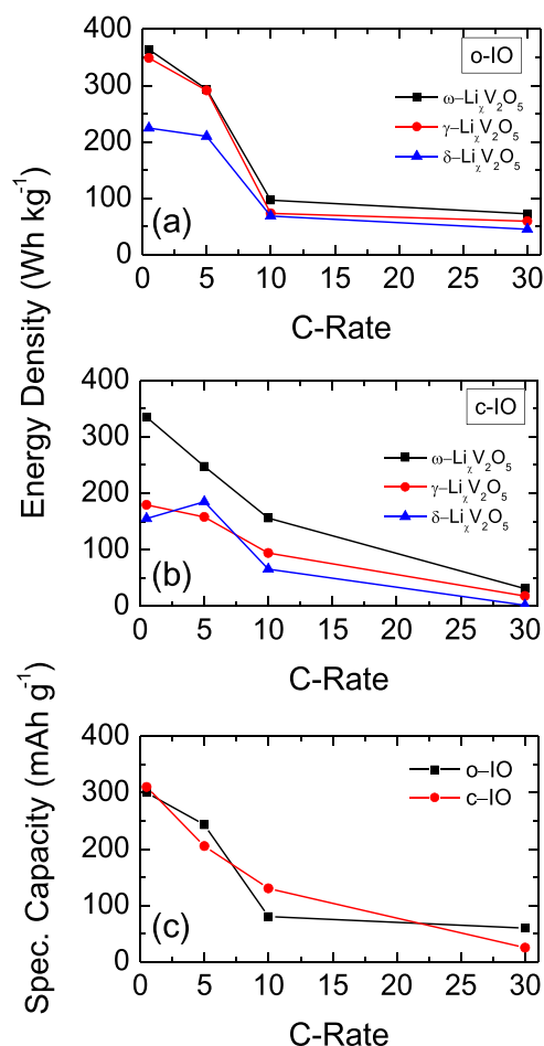
Figure 5. Energy density as a function of C-rate associated with each Li_xV_2O_5 phase change for the (a) o-IO and (b) c-IO V_2O_5 Li battery cathodes grown by electrodeposition. The total specific capacity of each electrode at all rates are also shown in (c).
