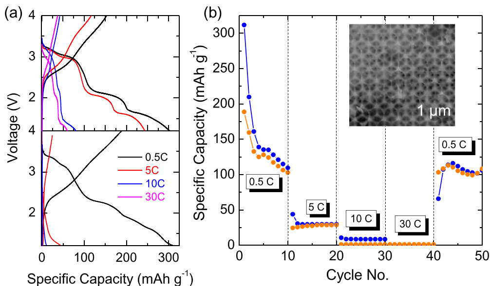
Figure 6. (a) First charge-discharge curves of separate o-IO V_2O_5 cathodes, each of which were discharged and charged at various C-rates. Underneath is the corresponding charge-discharge profiles of a single o-IO cathode successively discharged and charged at each C-rate. (b) A single o-IO V_2O_5 cathode cycled for 10 cycles at each C-rate for a total of 50 cycles, with SEM image of the material after cycling.
