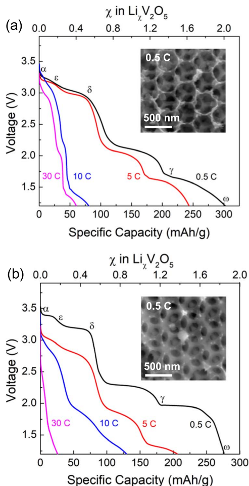
Figure 3. Galvanostatic 1st discharge curves for \text{V}_2\text{O}_5 IO electrodes in lithium batteries at various C-rates in the range 0.5–30 C. The cathode materials were formed by electrodeposition at 2.0 V (vs SCE) for (a) 300 s and (b) 900 s. The definitive phase changes to the orthorhombic \text{V}_2\text{O}_5 crystal structure during lithiation are marked \alpha – \omega . The insets show electron microscopy images of the internal IO network after discharge to 1.2 V (vs \text{Li}^+/\text{Li} ) at a rate of 0.5 C. The image shown in (b) is of the c-IO electrode that was not covered with the dense \text{V}_2\text{O}_5 overlayer.
