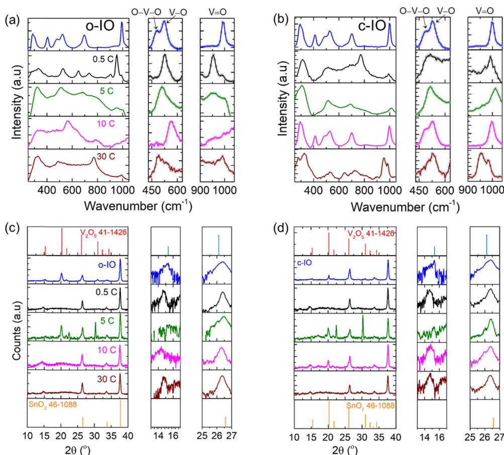
Figure 8. Raman scattering spectra of electrodeposited (a) o-IO \text{V}_2\text{O}_5 and (b) c-IO cathodes after 25 cycles at each C rate. Electrodes were analysed in ambient environment after removal from the electrolyte. The spectrum of the as-deposited \text{V}_2\text{O}_5 IO is also provided in each case cf. Fig. 1 for spectral bond identification. (c) XRD patterns for as-deposited IO, o-IO and (d) c-IO \text{V}_2\text{O}_5 cathodes at each C rate. Reference patterns for \text{V}_2\text{O}_5 (PDF 41-1426) and \text{SnO}_2 (PDF 64-1088) are also shown. The \text{SnO}_2 reflections come from the FTO coating on the underlying substrates.
