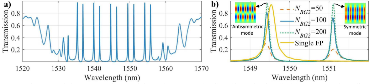
Fig. 3. a) Simulated transmission spectrum of the coupled FPs with N_{BG2}=200 . b) Effect of increasing the reflectivity of DBRs in the auxiliary FP.
