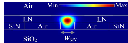
Fig. 1. The TE mode in the LN-on-SiN waveguide.
