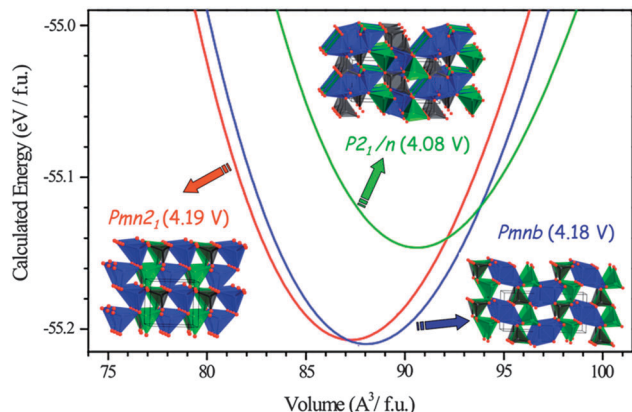
Fig. 15 Calculated total energy versus volume curves of \text{Li}_2\text{MnSiO}_4 polymorphs; Pmn2_1 (red), Pmnb (blue) and P2_1/n (green). DFT (GGA + U , U_{\text{effect}} = 4 eV) data were fitted to the Murnaghan equation of state. Calculated average voltage for the 2 electron process is given in parentheses. Reprinted with permission from ref. 193. Copyright 2008 American Chemical Society.
