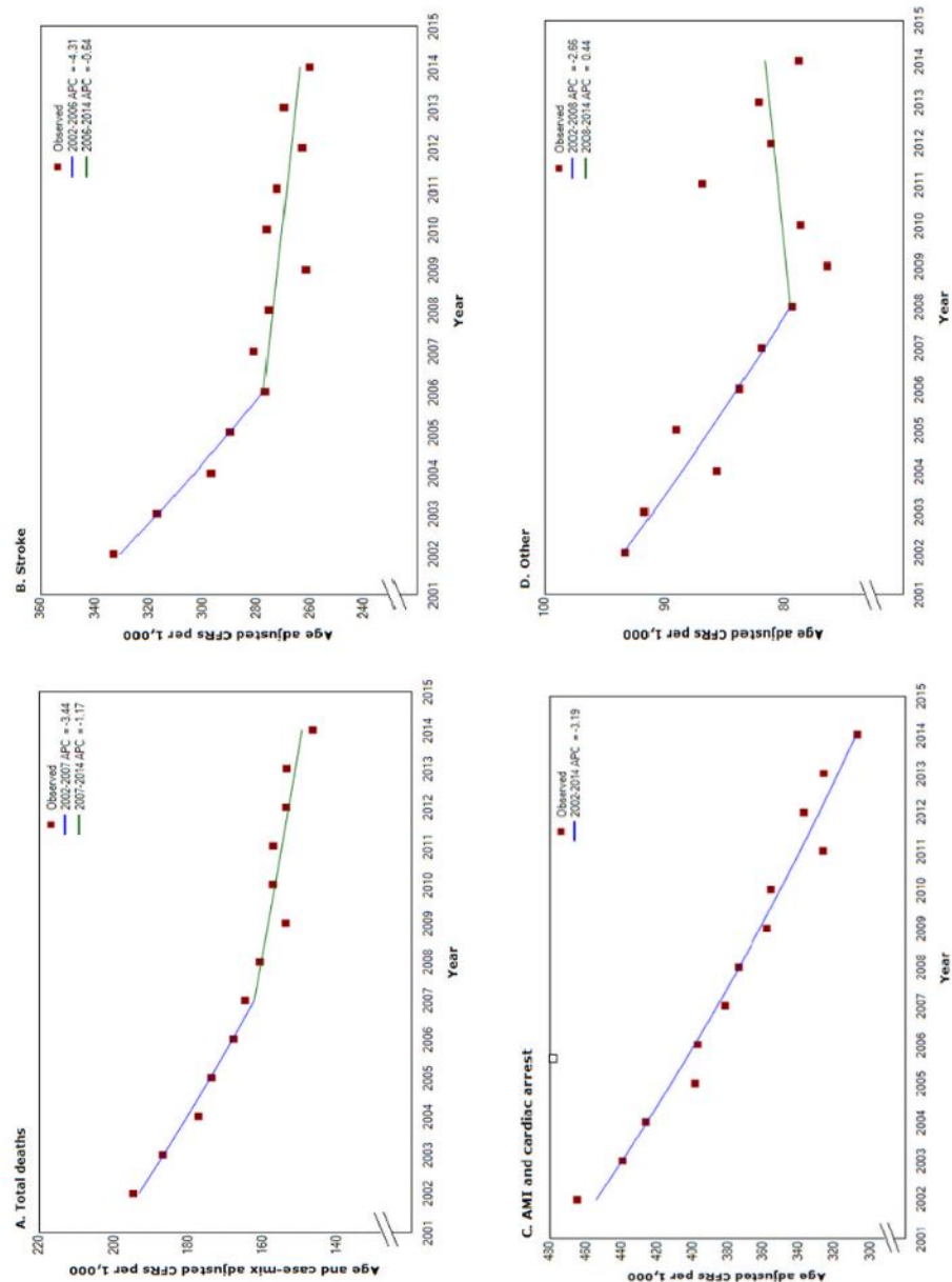
FIGURE 7.2: Joinpoint analyses of adjusted CFRs
