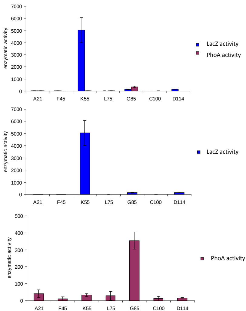
Fig. 3. . Activity of Ltntl-LacZ and Ltntl-PhoA fusions in E. coli CC118.
