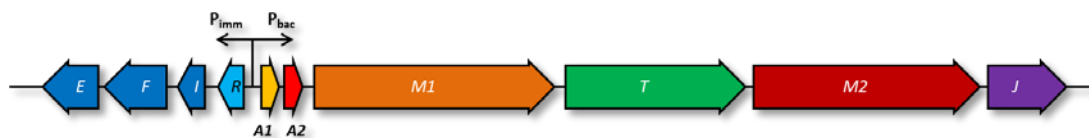
Fig. 1. The 12.6kb lactacin 3147 gene cluster. Two promoters P_{imm} and P_{bac} are located at the interface of the two divergent operons: ltnRIFE and ltnA 1 A 2 M 1 TM 2 J , which are responsible for the biosynthesis, immunity and export of the final lantibiotic.
