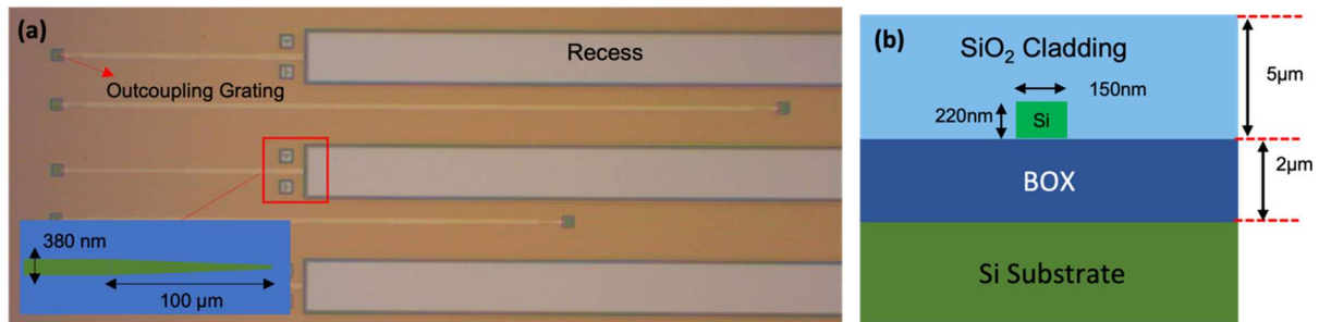
Fig. 1. a) 2.5 mm long and 120 \mu\text{m} wide recess on SOI wafer (Inset: schematic of Si waveguide coupler inverse tapered from 150 nm to 380 nm over 100 \mu\text{m} distance) and b) Cross section of a single tip inverse taper coupler design.
