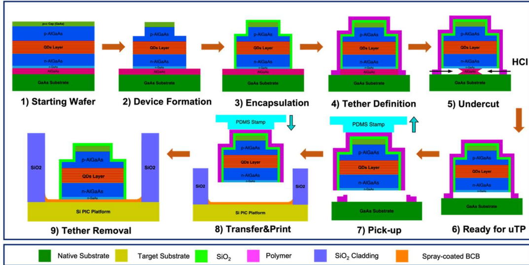
Fig. 3. Device fabrication flow on an epitaxial structure including an AlGaAs release layer (1-2). Coupons were encapsulated by \text{SiO}_2 for facet and epitaxial structure protection during release etch (3). A polymer (resist) anchor system (4) keeps coupons in place during sacrificial layer etch by \text{HCl}:\text{DI} (5). Then, devices are picked-up by a PDMS (Polydimethylsiloxane) stamp (7) and transfer-printed into 7 \mu\text{m} deep Si recess (8). Finally, the resist tethers were removed for electrical connection (9).
