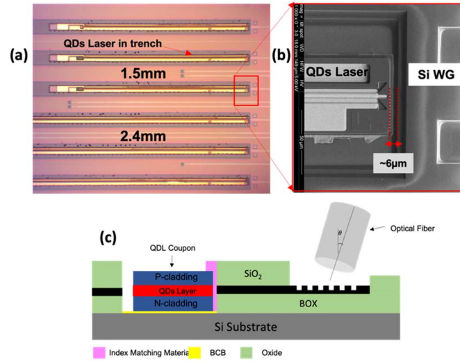
Fig. 4. a) Optical image that shows QD laser coupons >1.5\text{ mm} length transfer-printed into a deep trench on SOI, b) SEM image of a laser coupon inside a recess next to a Si waveguide coupler and c) Edge coupling schematic describing light coupling from laser to Si waveguide and from Si grating to fiber.
