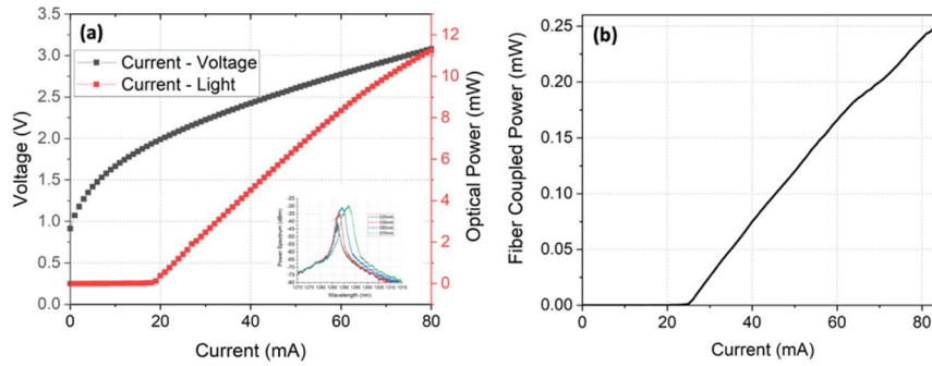
Fig. 5. a) LIV plots of a transfer printed 1.8\text{ mm} QD laser on 1\mu\text{m} Intervia on Si (Inset: spectrum at different bias current) and b) Current versus coupled light into the Si waveguide from a 1.8\text{ mm} long laser coupon.
