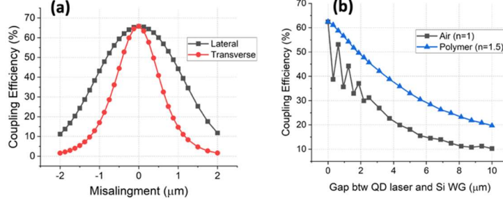
Fig. 2.a) Lateral and transverse misalignment tolerance simulation for an inverse single tapered waveguide, and b) Longitudinal tolerance as a function of spacing and refractive index of filling material.
