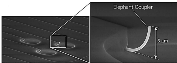
Fig. 12. SEM image of a vertically bent optical coupler, obtained by ion implantation in a silicon waveguide. The bent waveguide is 5\text{ }\mu\text{m} long, and the curvature radius is approximately equal to 3\text{ }\mu\text{m} . Reproduced from [43].
